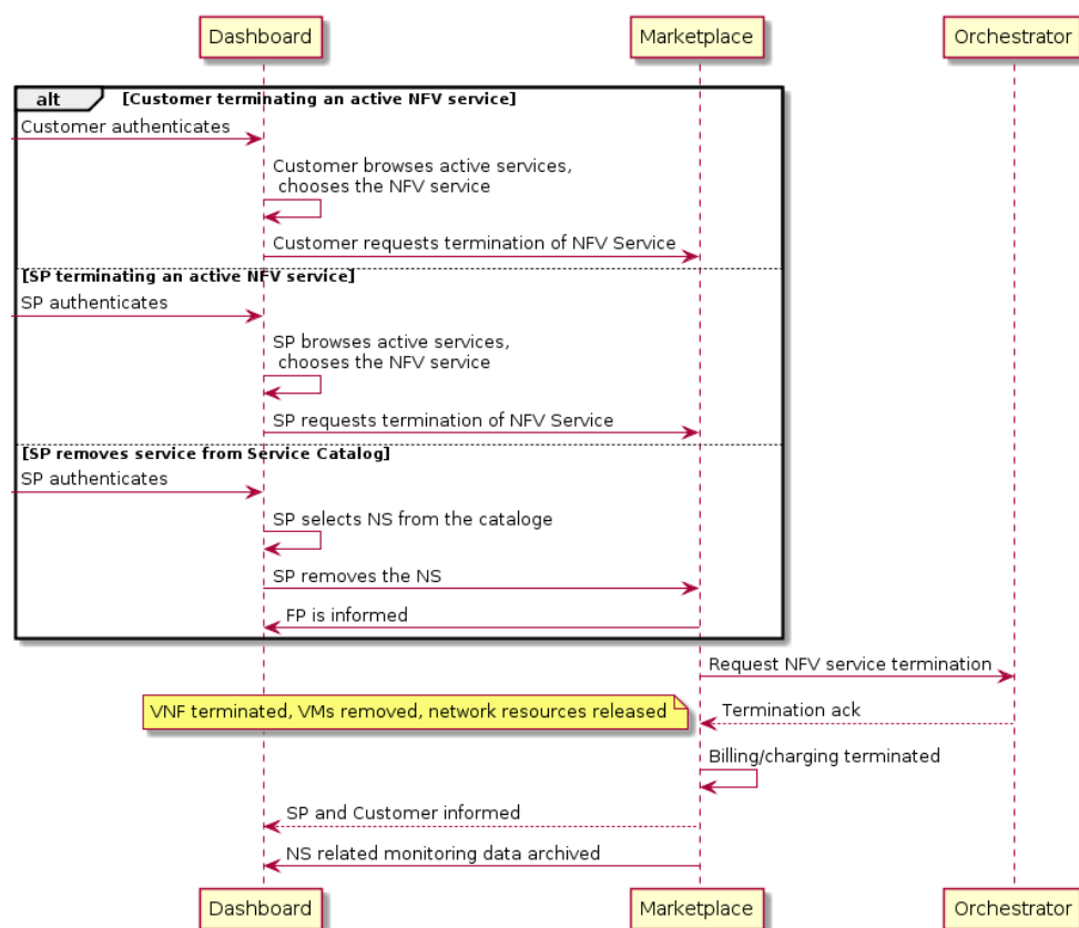
Figure 37 UC7 Sequence Diagram
