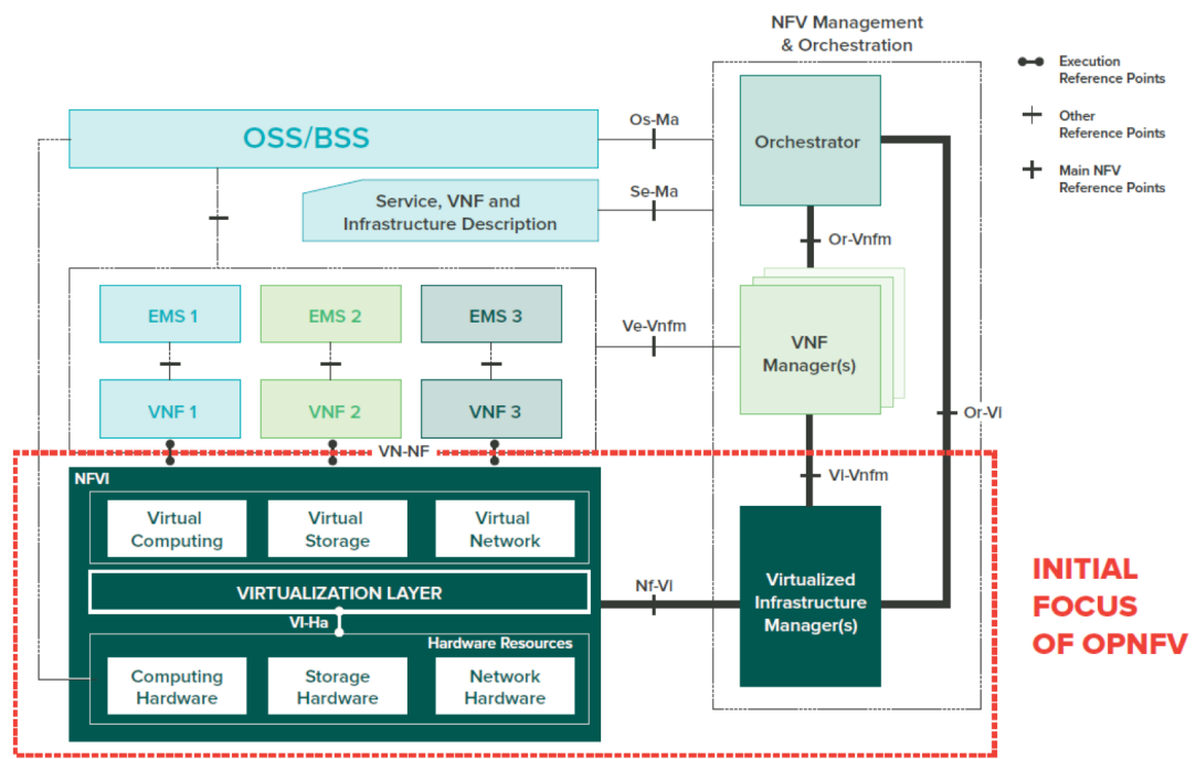
Figure 3. OPNFV mapping to ETSI reference architecture
