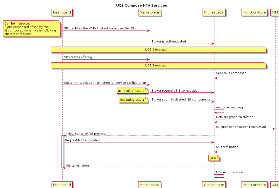
Figure 27 UC2 NfV Service Composition Sequence Diagram
