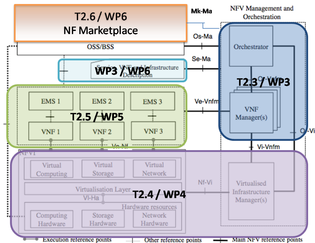
Figure 25. T-NOVA scope mapping into ETSI NFV reference architecture
