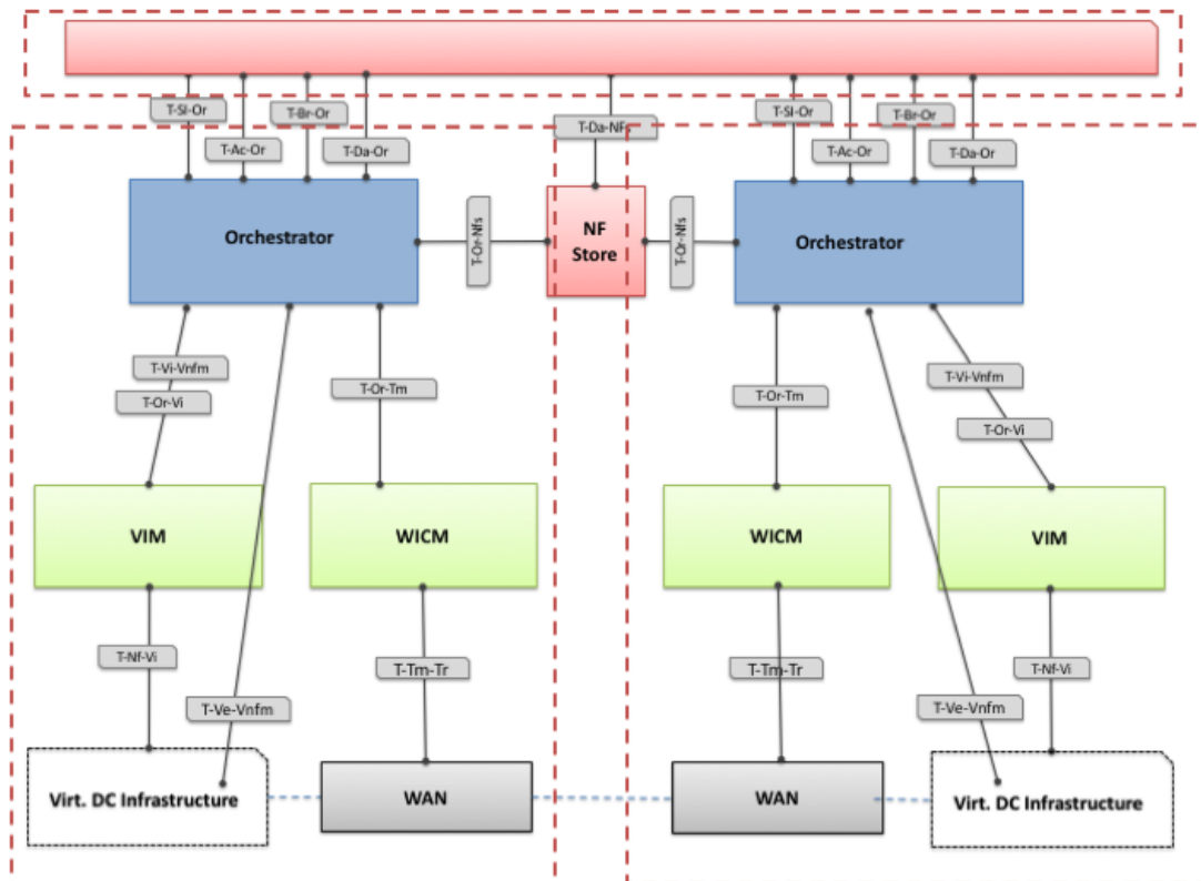
Figure 41. Architecture extension to support multiple SPs under a common broker
