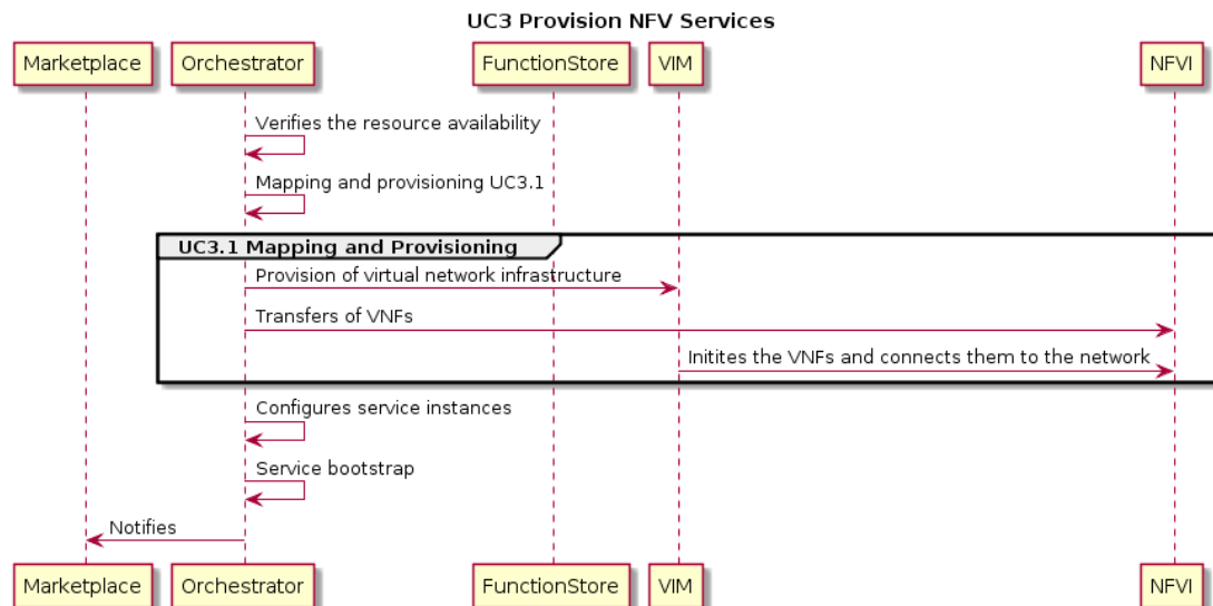
Figure 30 UC3 Provision of NFV Services Sequence Diagram
