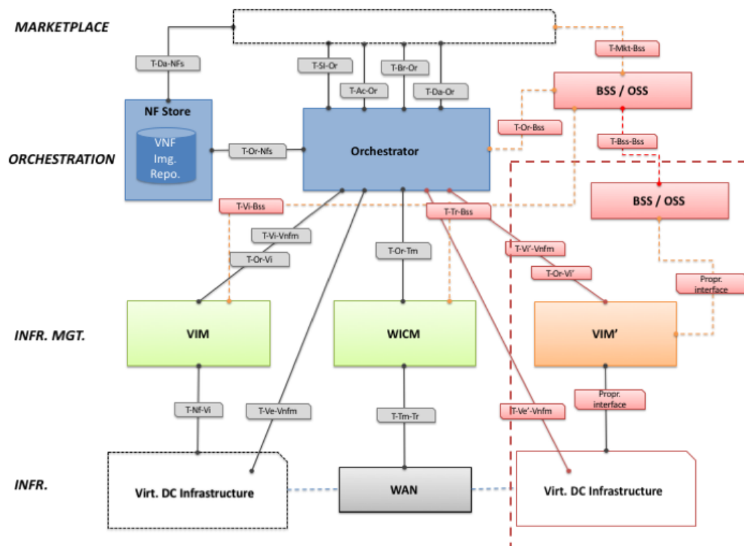
Figure 40. Architecture extension to support multiple NFVI-PoP providers
