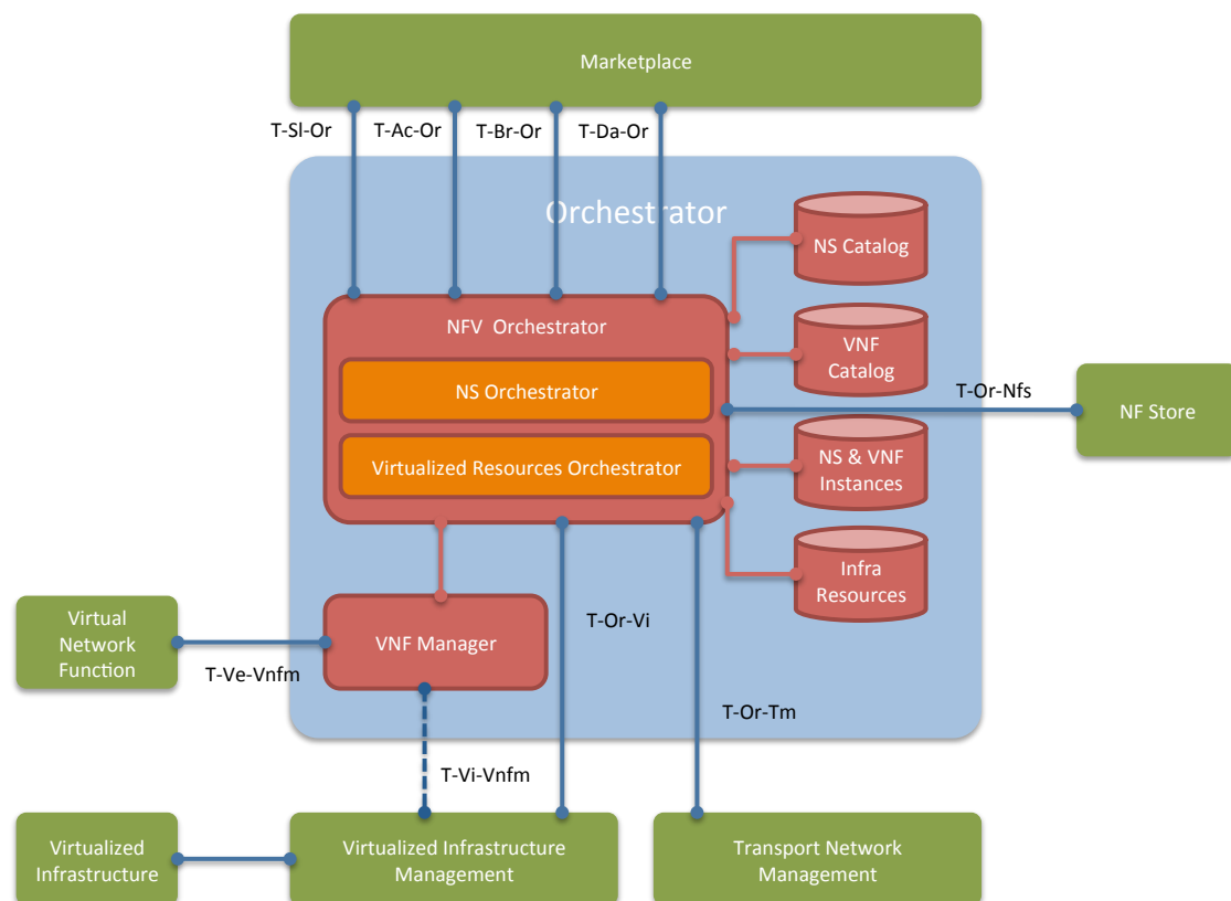
Figure 23. T-NOVA Orchestrator Reference Architecture and Interactions
