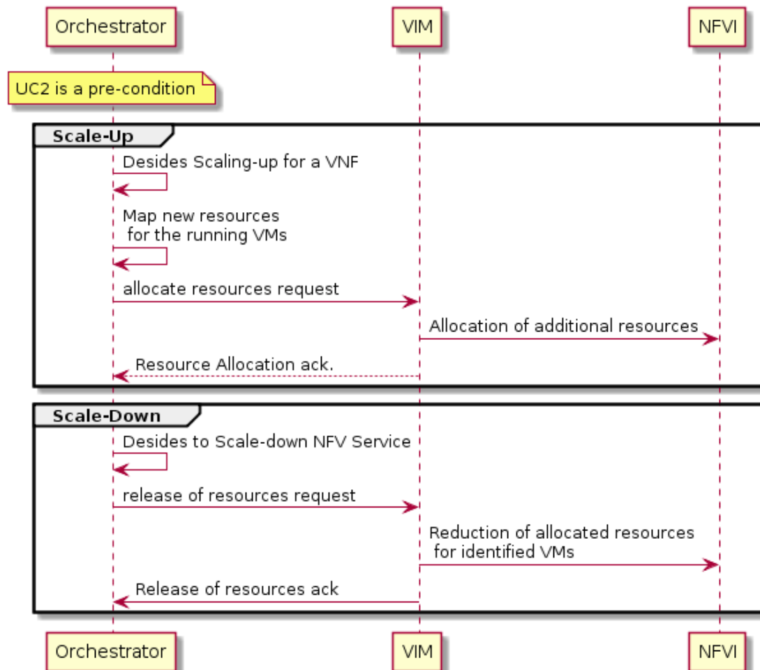
Figure 32. UC4.2 Sequence Diagram
