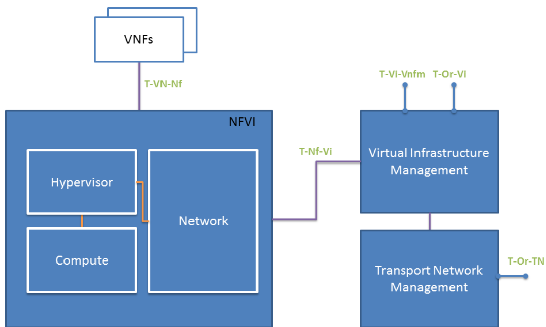
Figure 24. High-level architecture of T-NOVA IVM.
