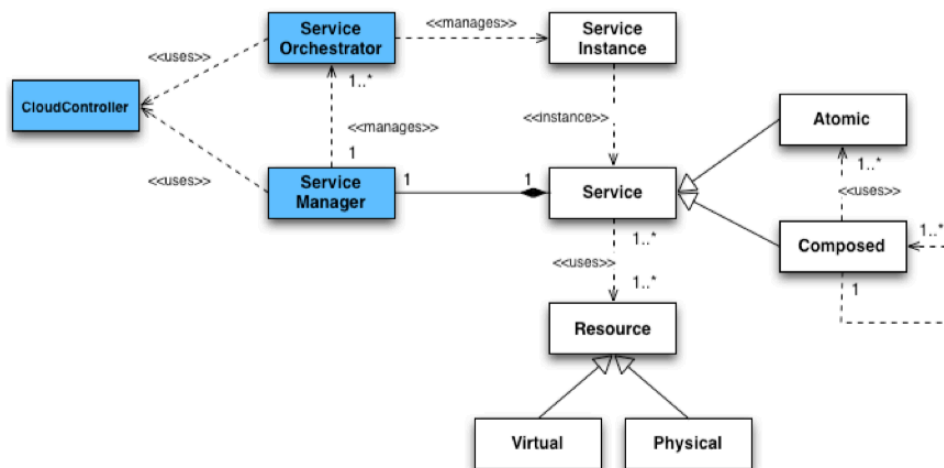
Figure 16. MCN Architectural Entities Relationship
