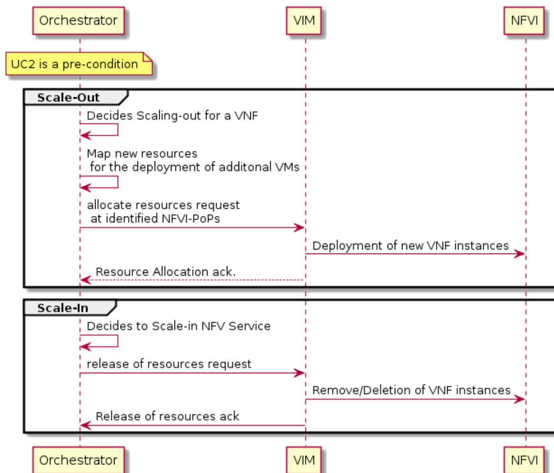
Figure 31. UC4.1 Sequence Diagram
