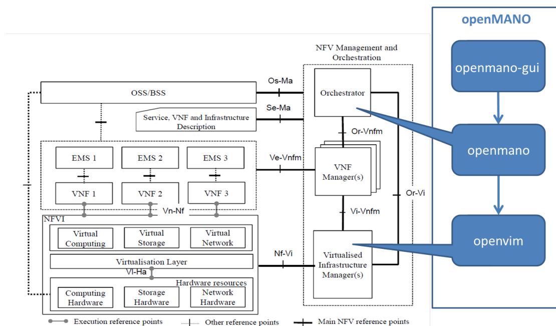
Figure 11. OpenMANO relation to ETSI NFV architecture
