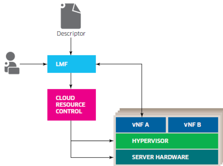
Figure 10. VNF deployment sequence
