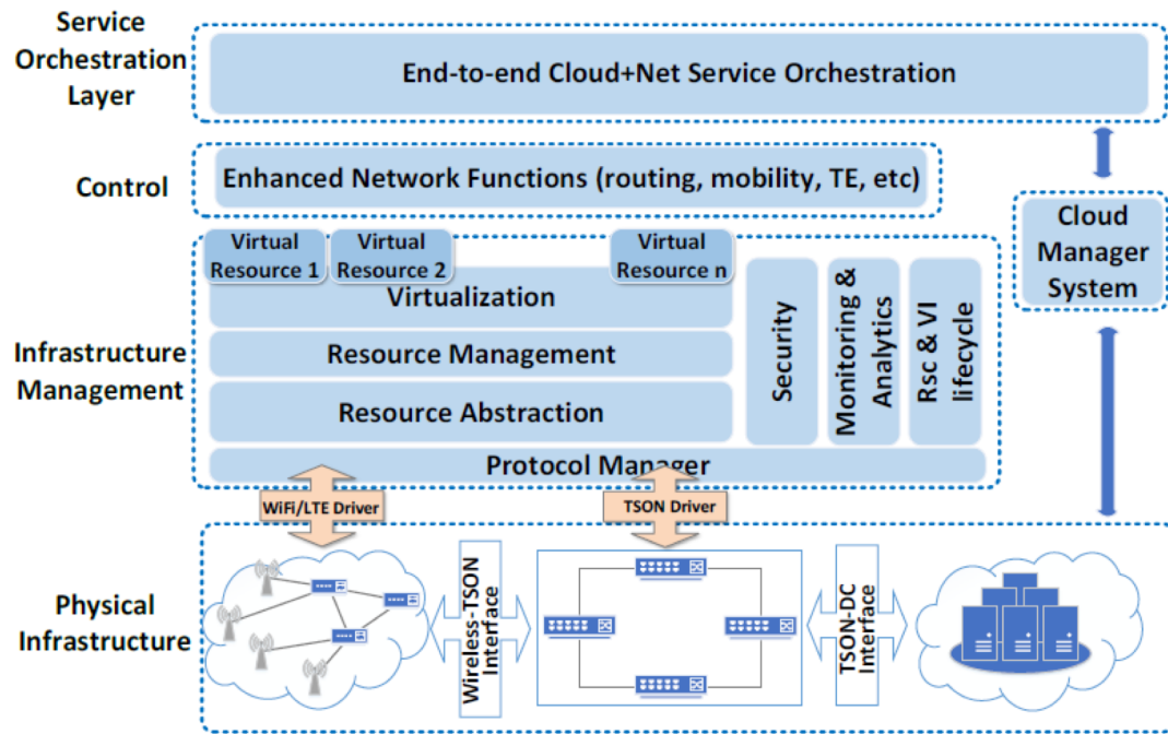
Figure 17. Overall CONTENT layered architecture
