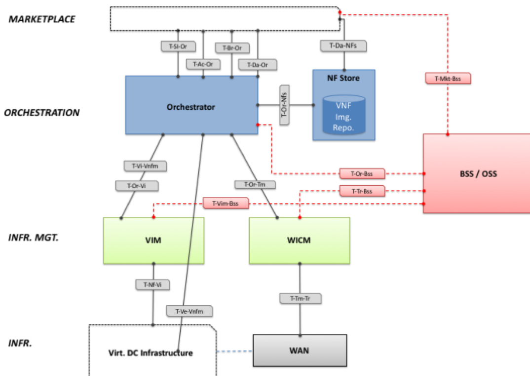
Figure 39. Architecture extension for interfacing with BSS/OSS
