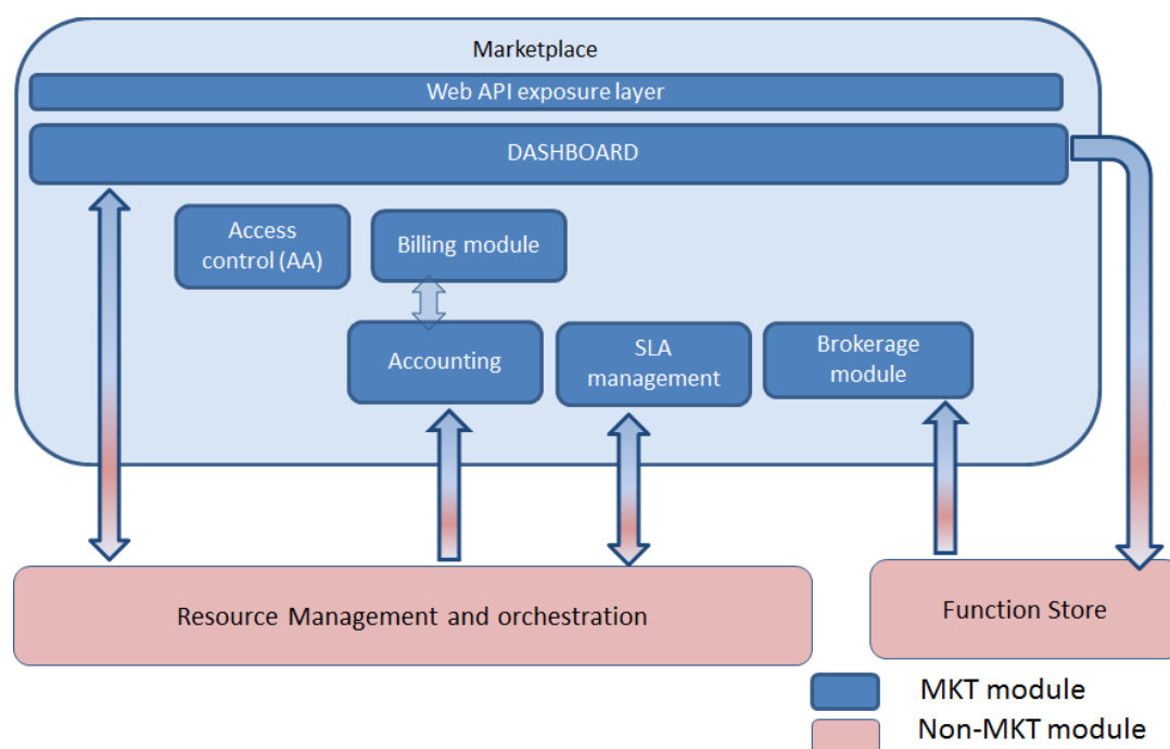
Figure 22. Marketplace external interfaces
