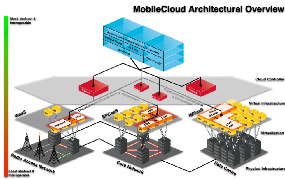
Figure 14. Mobile Cloud Networking Vision
