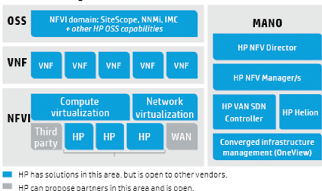
Figure 5. HP OpenNFV model
