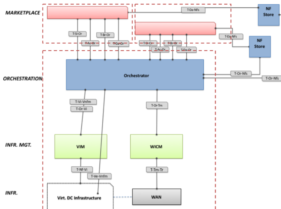
Figure 43. Architecture extension for multiple brokers under the same SP
