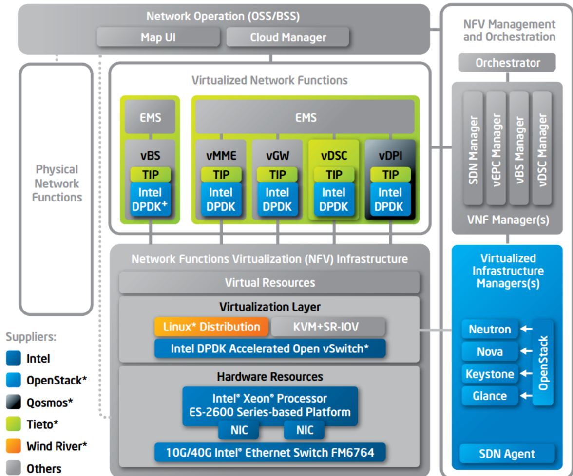
Figure 7. Intel NFV High Level Architecture
