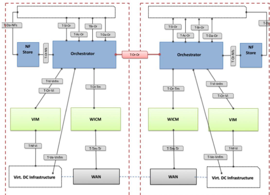
Figure 42. Architecture extension for SP federation
