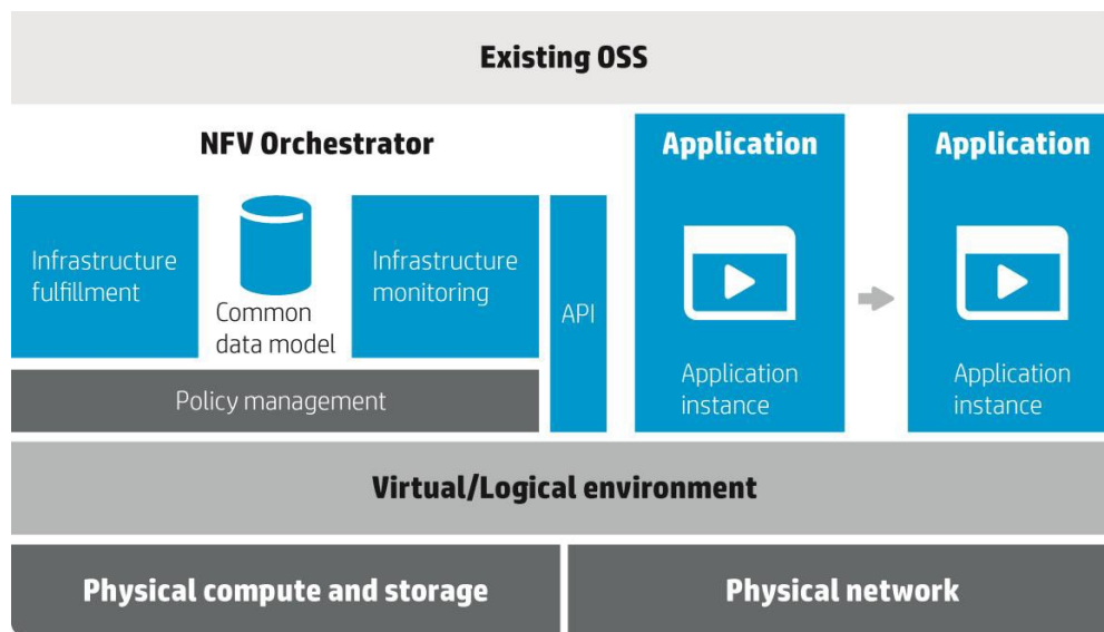
Figure 6. HP OpenNFV Functional Architecture
