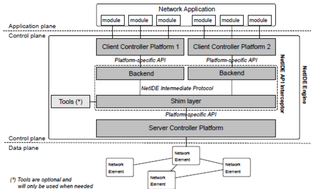
Figure 18. NetIDE Network Engine Architecture
