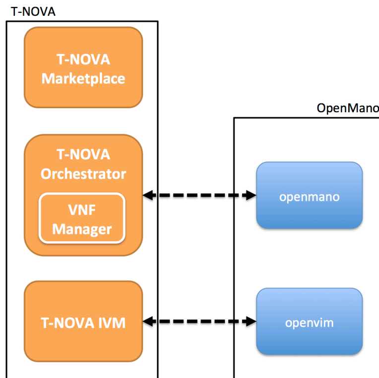
Figure 12. OpenMANO relation to T-NOVA components
