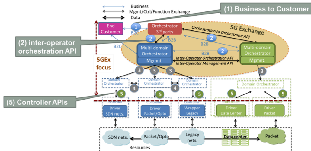
Figure 38. 5GEx concept
