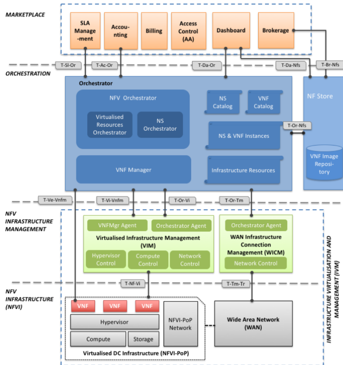
Figure 20. High-level view of overall T-NOVA System Architecture
