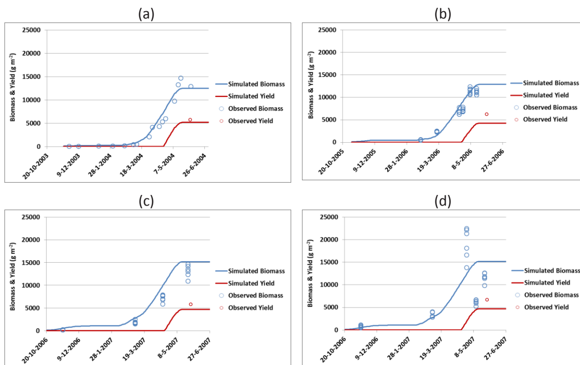
Figure 2: Comparison of the simulated biomass and yield against the observations for winter wheat crop at Fengqiu experimental site in different years.
