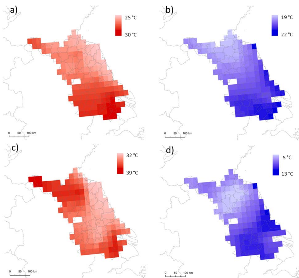
Figure 5 Daily maximum (a) and minimim (b) temperature averaged out from June to October 2006. Maximum value reached by daily maximum temperature (c) and minimim value reached by daily minimum temperature (d) from June to October 2006.
