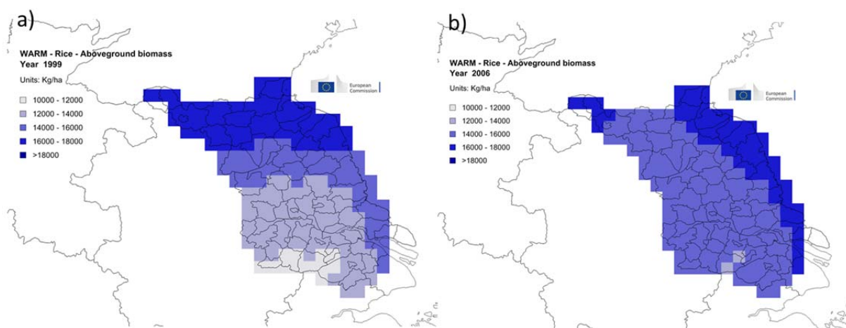
Figure 2 Maximum value of aboveground biomass simulated by WARM in: a) 1999 growing season; b) 2006 growing season. Grid cell resolution is about 25 \times 25 \text{ km} .
