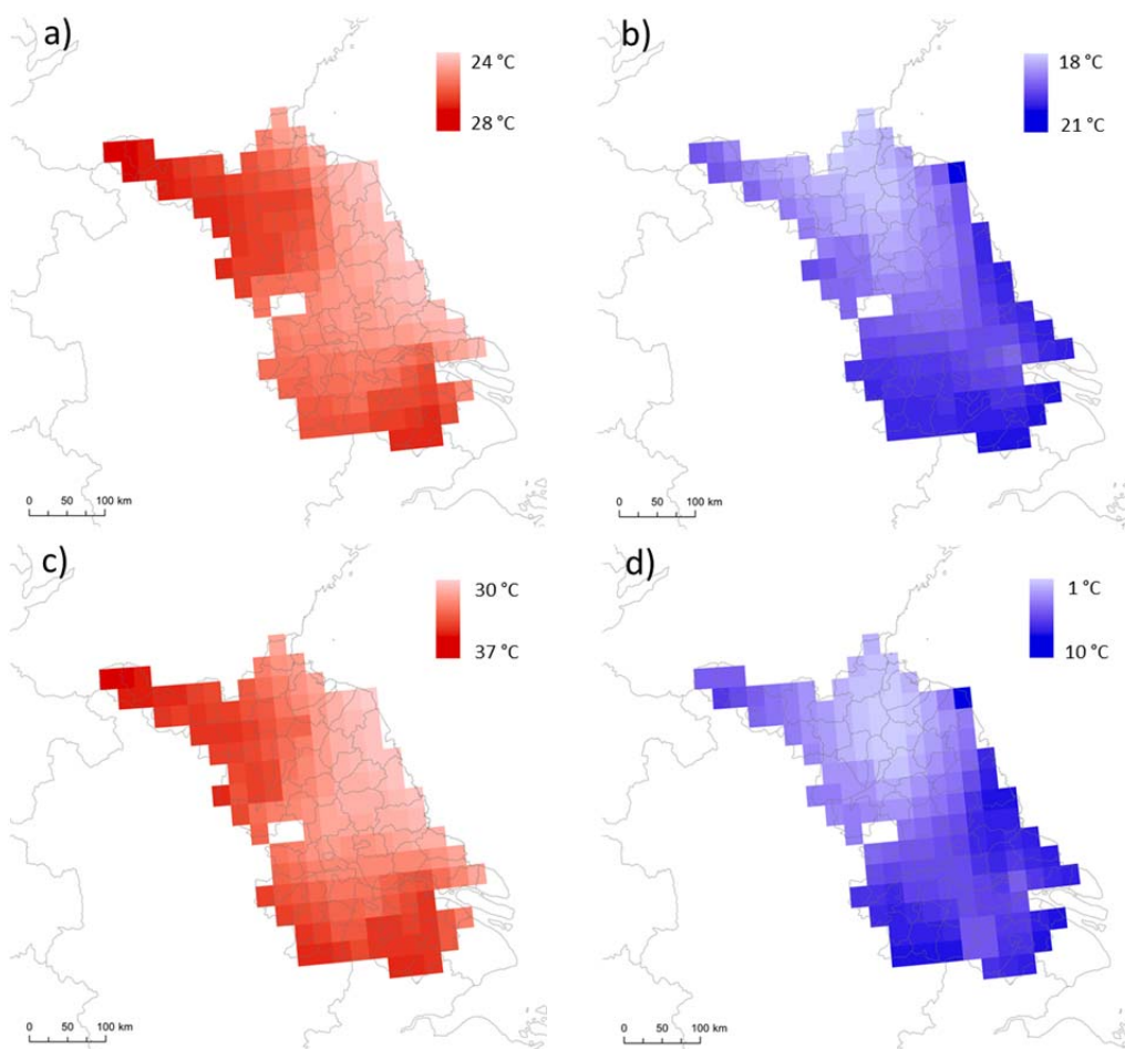
Figure 4 Daily maximum (a) and minimim (b) temperature averaged out from June to October 1999. Maximum value reached by daily maximum temperature (c) and minimim value reached by daily minimum temperature (d) from June to October 1999.
