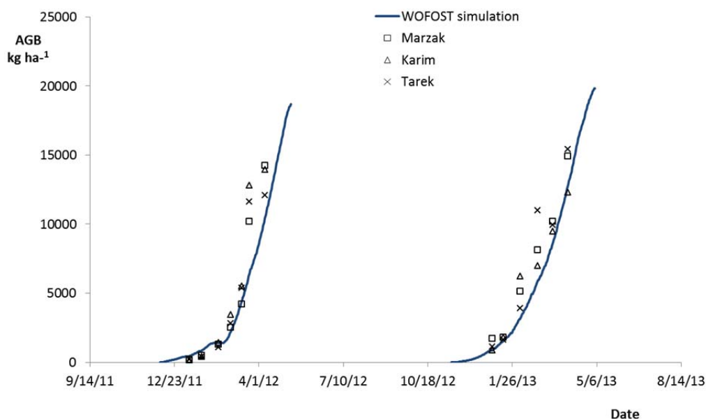
Figure 17. Comparison between measured (squares, triangles and crosses identify the different cultivars) and simulated (blue line) aboveground biomass of durum wheat in 2011-2012 and 2012-2013 cropping seasons. Sidi-El-Aydi, WOFOST model
