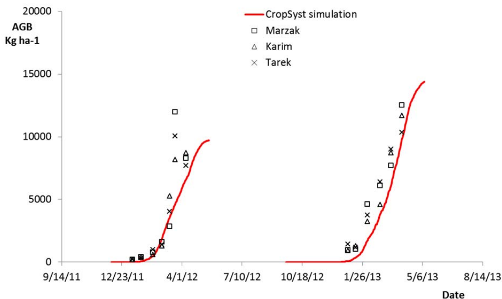
Figure 30. Comparison between measured (squares, triangles and crosses identify the different cultivars) and simulated (red line) water limited aboveground biomass of durum wheat in 2011-2012 and 2012-2013 cropping seasons. Sidi-El-Aydi, CropSyst model
