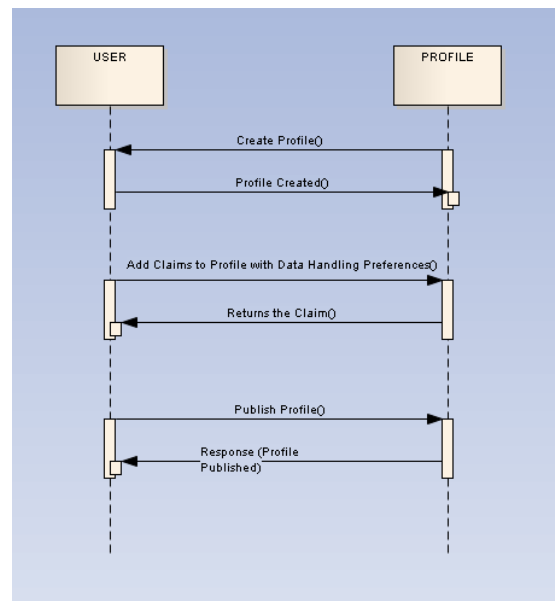
Figure 16: eCV Profile
