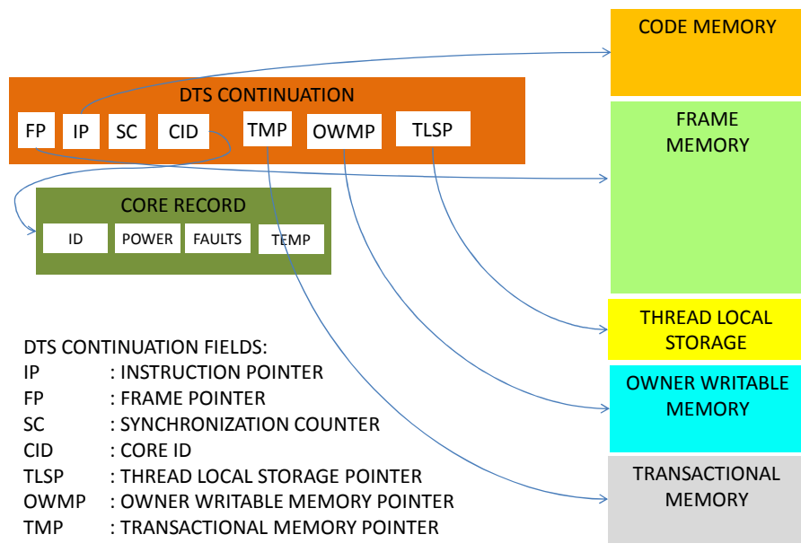
Figure 2 – High Level Model Implementation (a design option for the DTS continuation).
