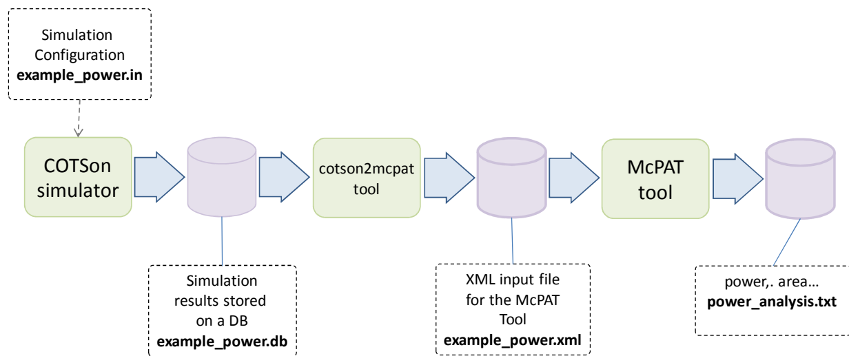
Figure 1 – Extracting power data in COTSon.
