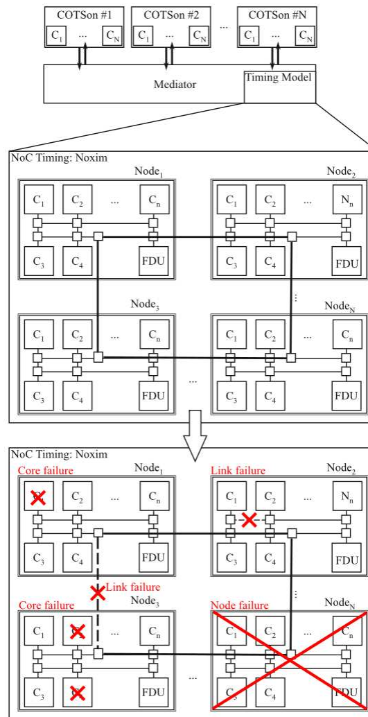
Figure 3 - Faults in COTSon/Noxim.
