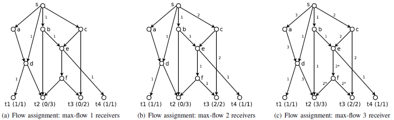
Figure 5 - Different stages of the MultiLayer-MaxFlow algorithm: layer assignment per link and rate achieved vs. maximum flow per receiver
