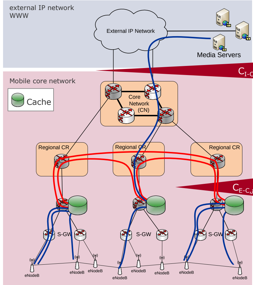
Figure 16 - Scenario 4: Collaborative regional caches
