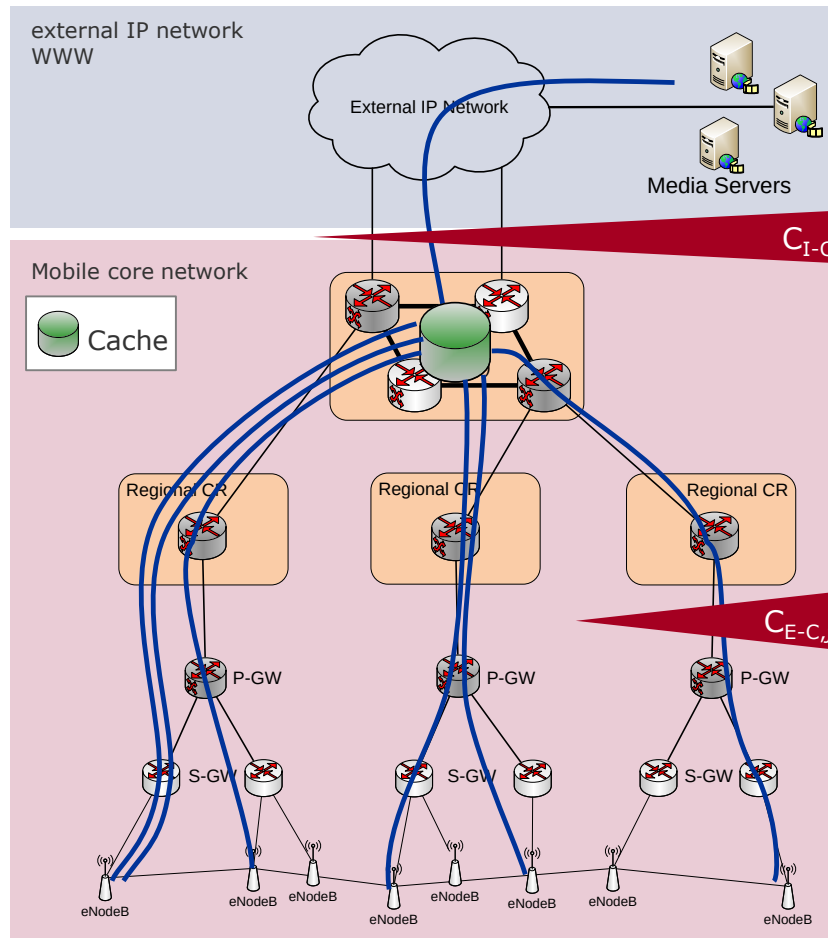
Figure 12 - Scenario 2: One centralized cache
