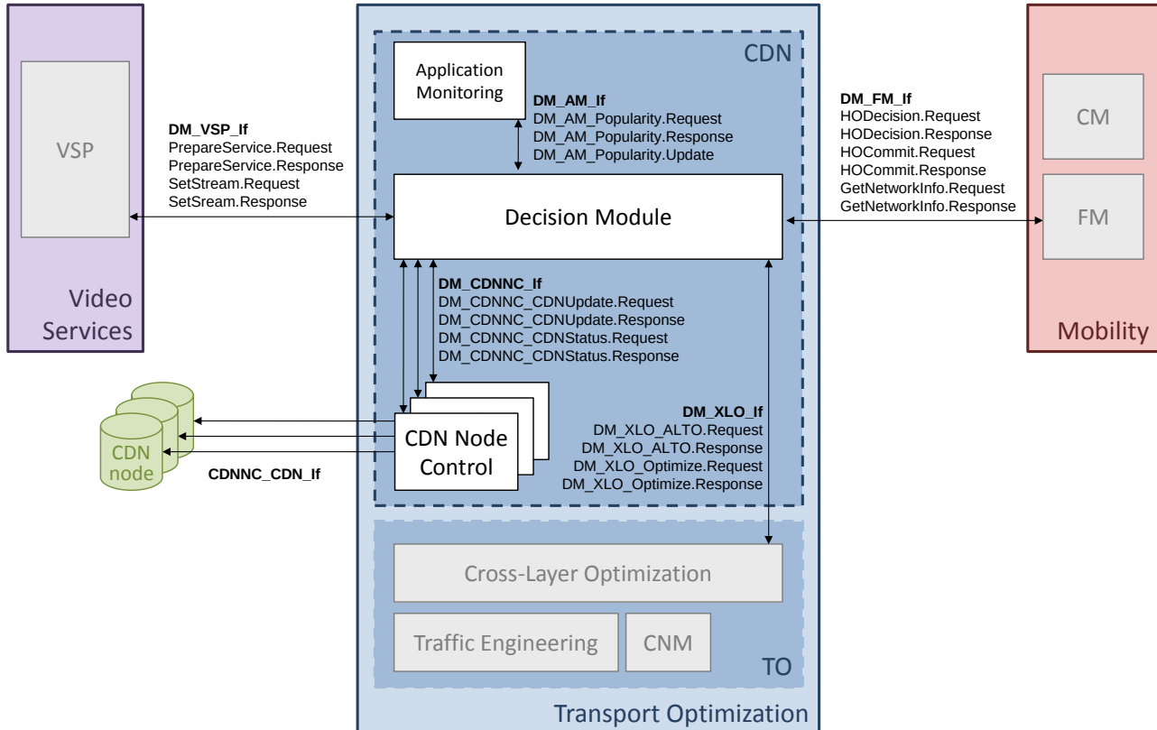
Figure 6 - Building blocks of the CDN component
