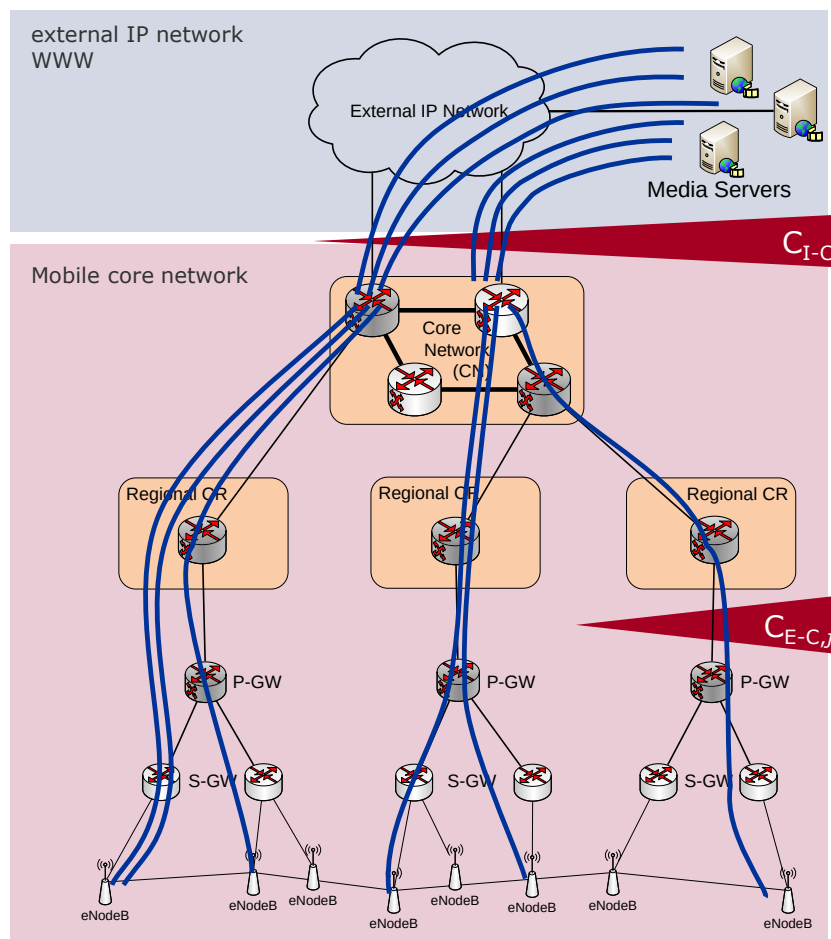
Figure 11 - Mobile operator network topology
