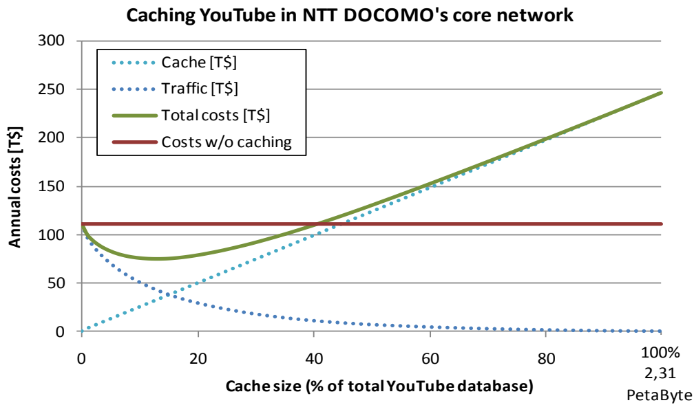
Figure 22 - Total annual costs when caching the caching the Top X videos
