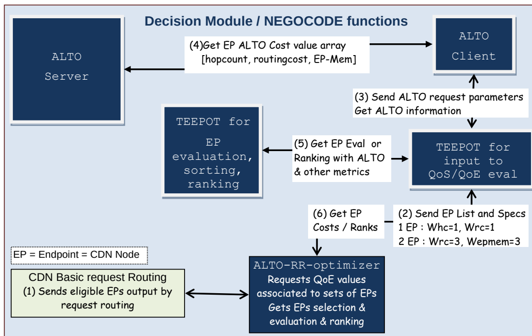
Figure 7 - The NEGOCODE functional block of the DM (components in blue) and their interaction
