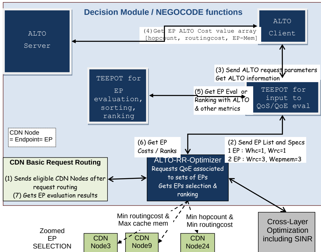
Figure 1 - Transactions between components (ALTO Client, Server, TEEPOTs) of the NEGOCODE block The figure shows how multiple costs for multiple sets on connections are requested and processed. NEGOCODE components are boxes in blue.
