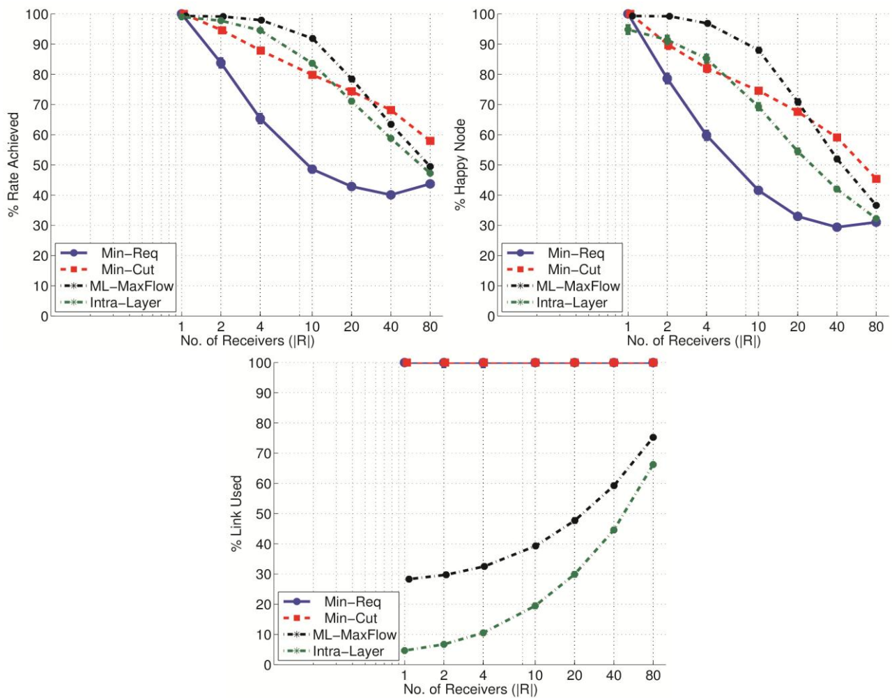
Figure 24 - Different number of receivers of 1 - 80 nodes, for a network with 160 nodes
