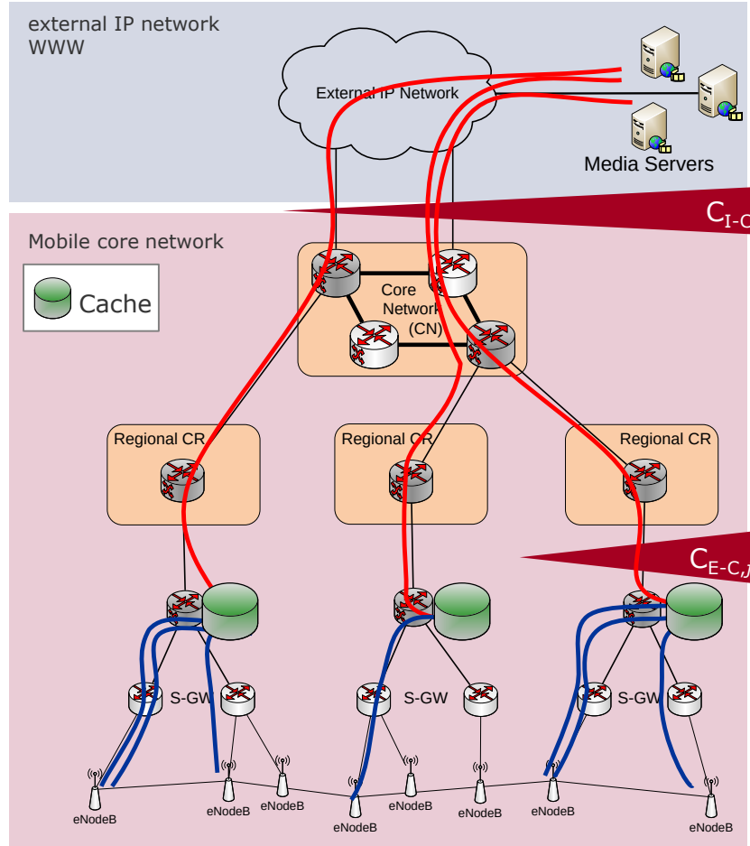
Figure 14 - Scenario 3: Autonomous regional caches
