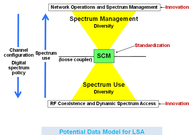
Figure 5-4: IEEE 1900.5 Data Model
