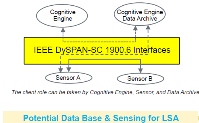
Figure 5-3: IEEE 1900.6 Interfaces
