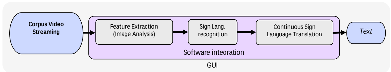
Figure 2. SignSpeak framework
