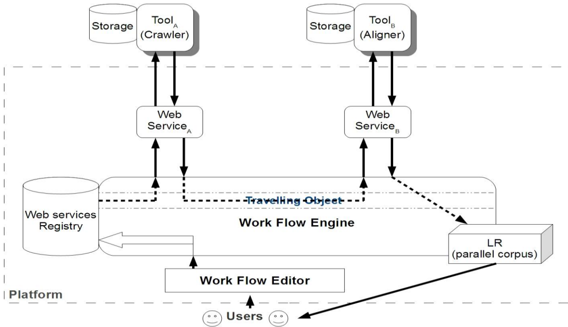
Figure 1: PANACEA platform. Starting point for the analysis
