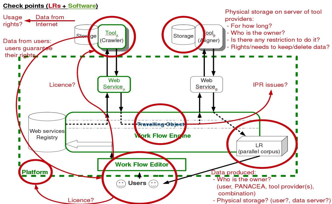
Figure 2: "Check-points" concerns to be handled within the platform
