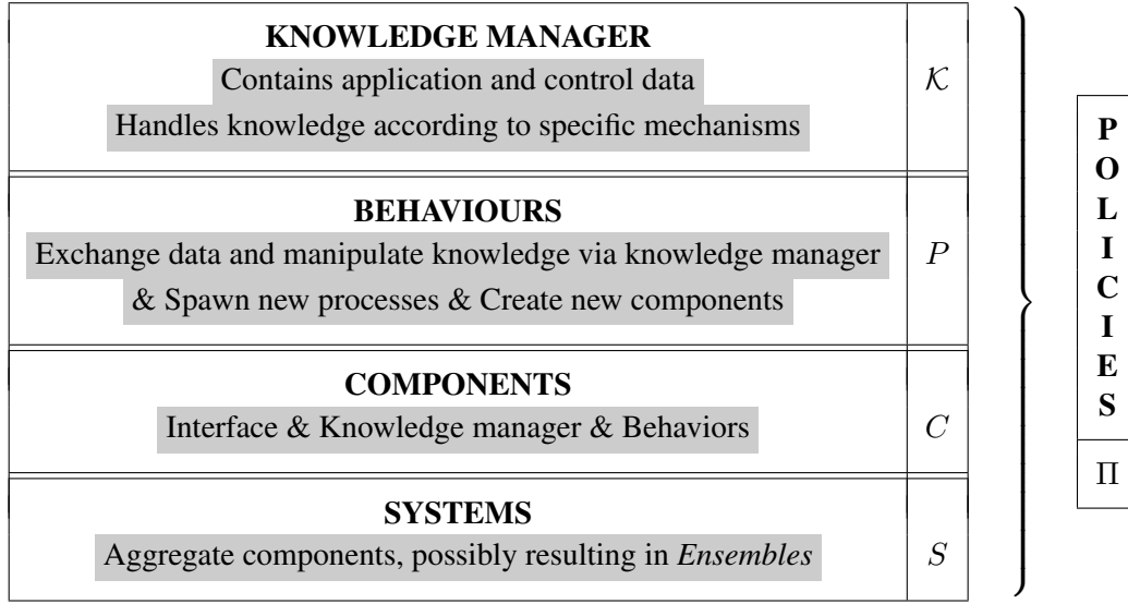
Figure 1: SCEL abstractions
