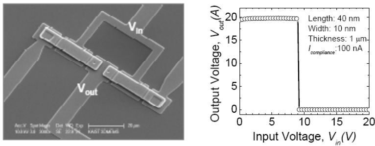
Figure 9. SEM image of an inverter based on MEM switches and the corresponding voltage transfer curve.
