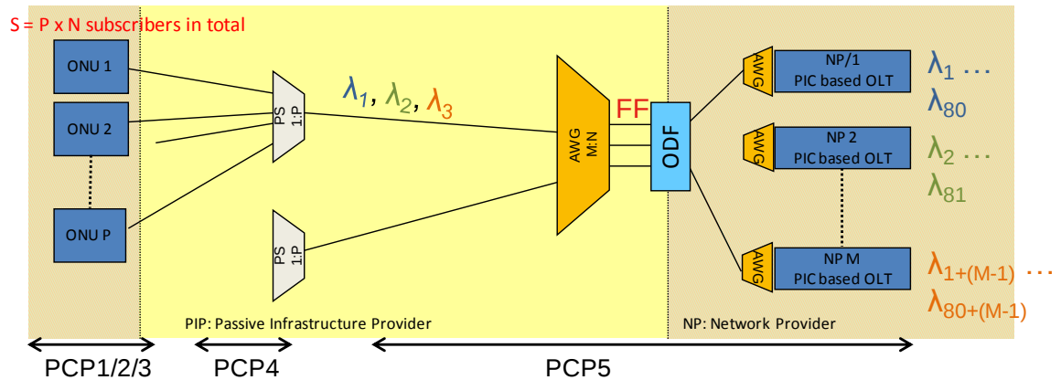
Figure 9: Schematic representation of open access on wavelength layer for HPON
