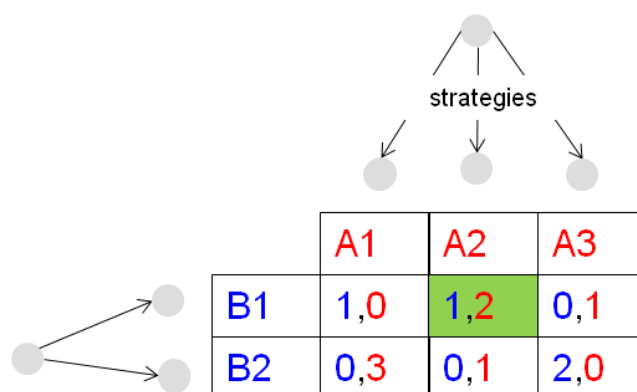
Figure 65: Strategic form of a game and Nash equilibrium
