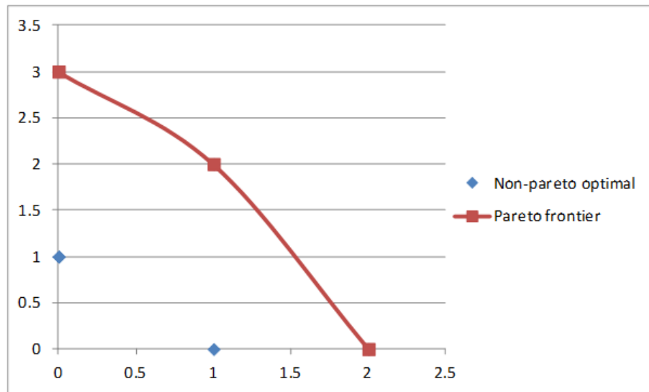
Figure 66: Pareto optimal strategy sets for the example game
