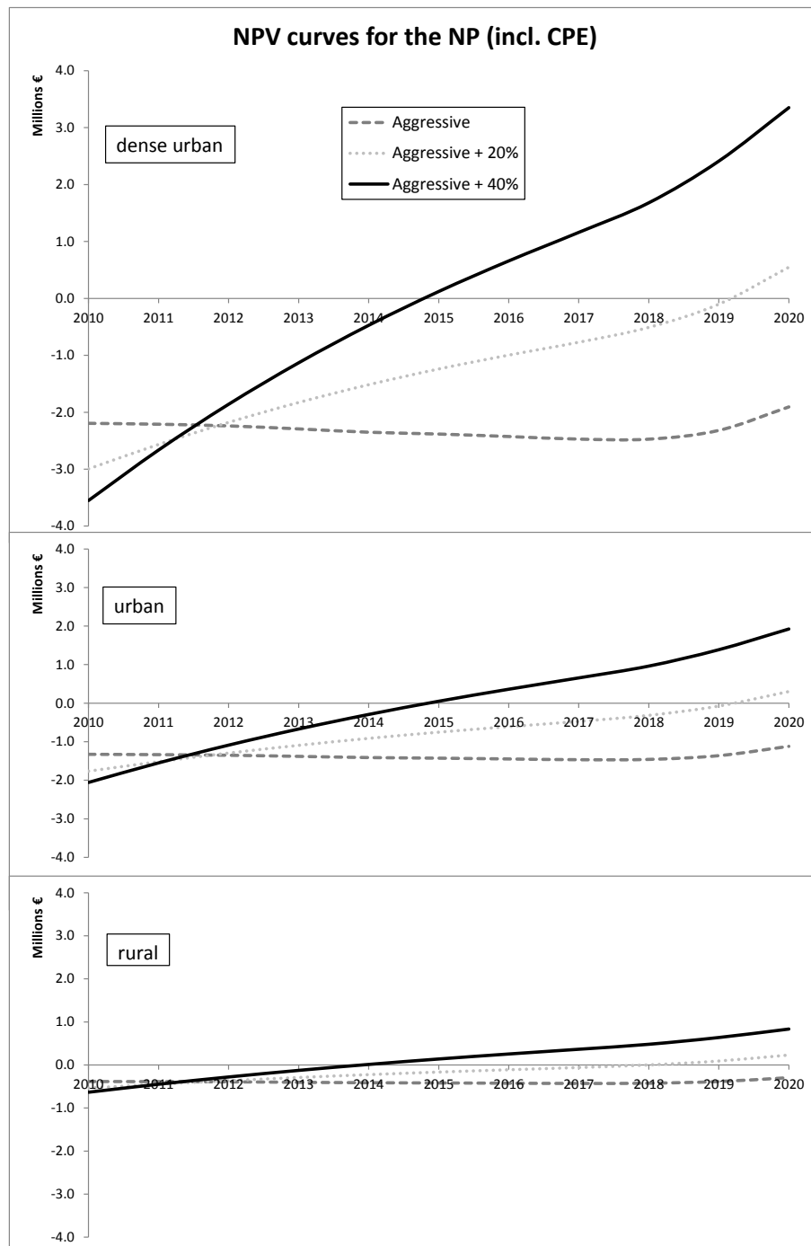
Figure 51: NPV curves for the NP business case based on GPON 1:32 and demand aggregation with 20% and 40% in 2010 (€10 monthly fee, 10% discount and cumulated)
