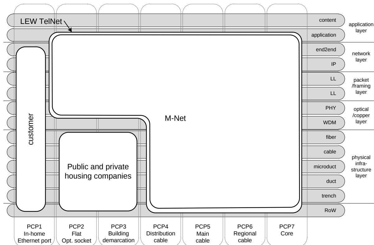
Figure 104: Division of roles based on Physical Connection Points (Bavaria case)
