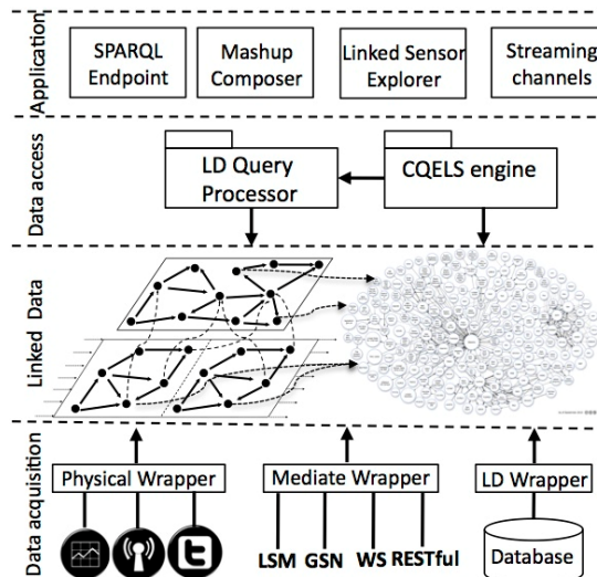
Figure 16: LSM Architecture
