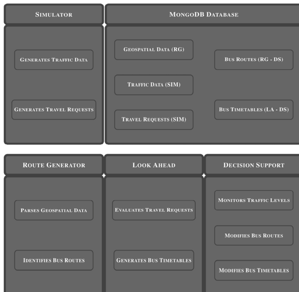
Figure 31: System architecture of the Transportation Planner
