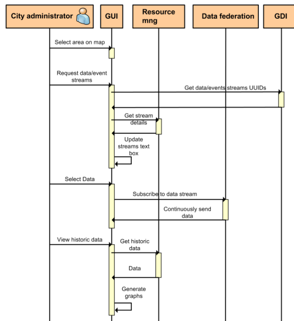
Figure 21: CityPulse dashboard workflow
