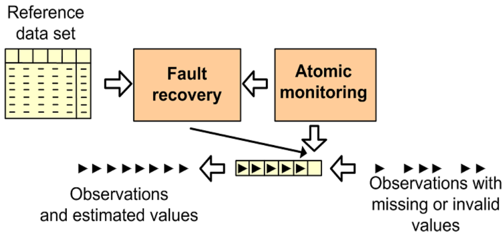
Figure 12: Fault Recovery process flow
