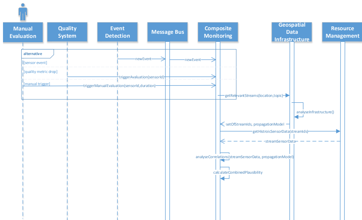
Figure 13: Sequence Diagram of the Composite Monitoring Process
