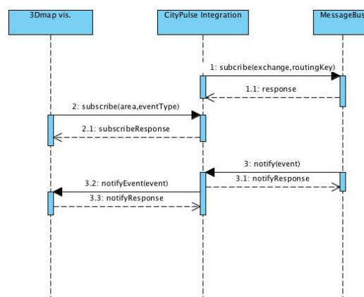
Figure 19: 3D Map - Sequence Diagram
