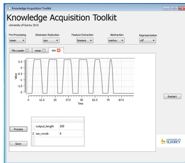
Figure 7: KAT - Create a Symbolic Representation
