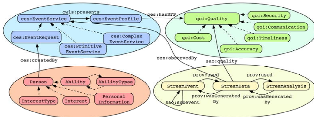
Figure 15: CityPulse Information Model
