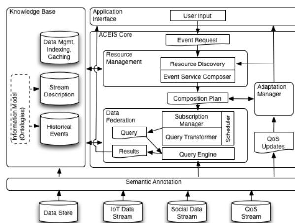
Figure 11: ACEIS Architecture
