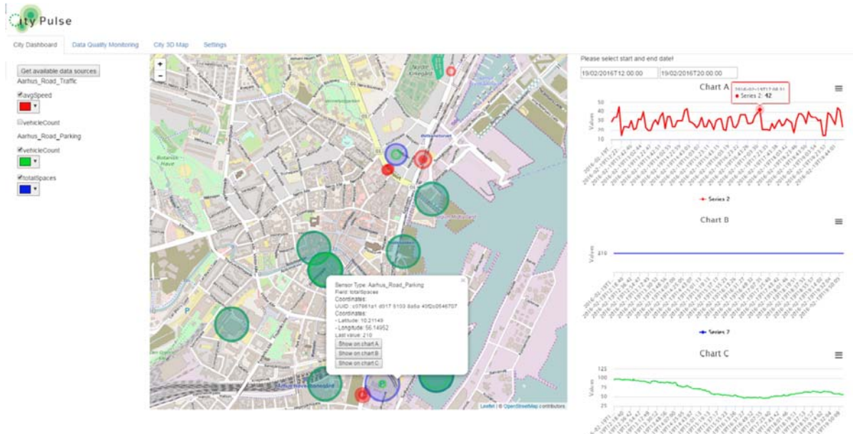
Figure 20: CityDashboard GUI
