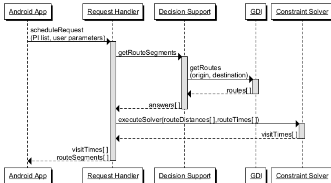
Figure 28: Sequence diagram to generate a schedule
