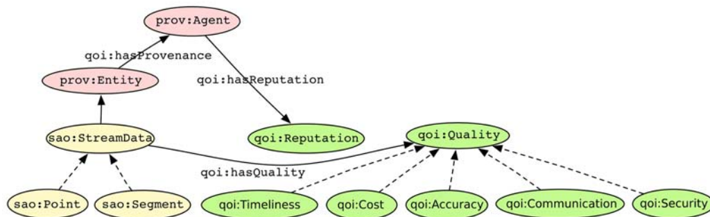
Figure 14: Quality Ontology
