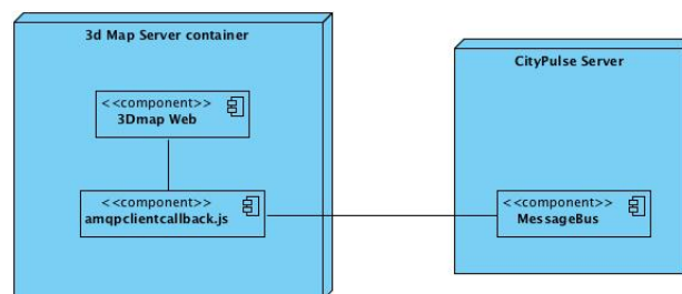
Figure 18: 3D Map application Deployment Diagram
