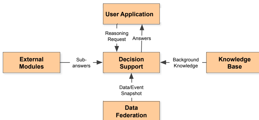
Figure 33: Decision Support Interactions
