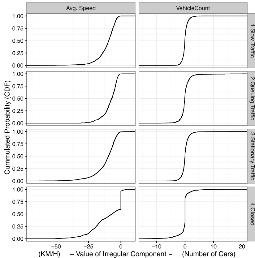
Figure 26: Avg. Speed (Irregular) and Vehicle Count (Raw) Change During Traffic Incidents
