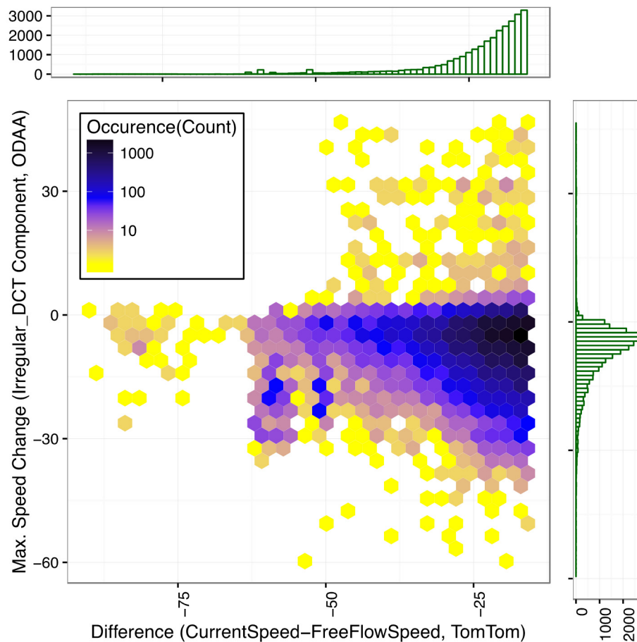
Figure 27: Heat Map of Measured Value Pairs of Measured Traffic Speed Changes
