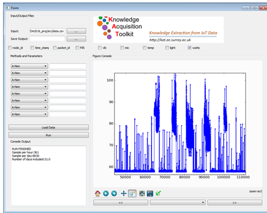
Figure 16: KAT Data Analytics Toolkit
