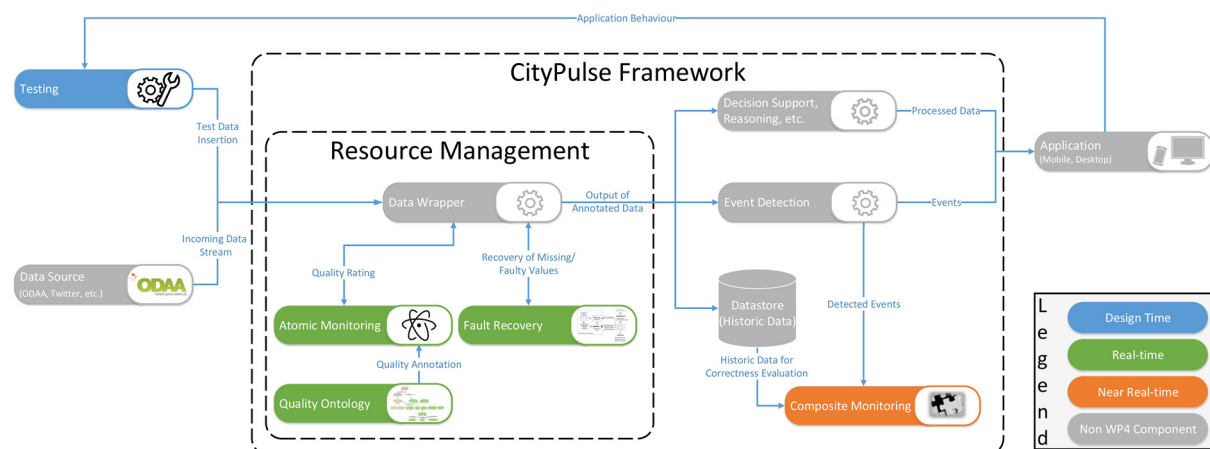
Figure 17: Reliable Information Processing Overview
