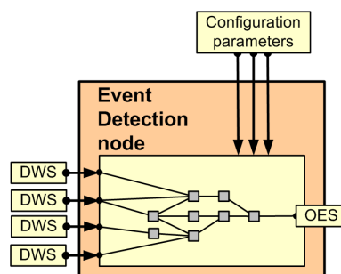
Figure 15: Event Detection Node
