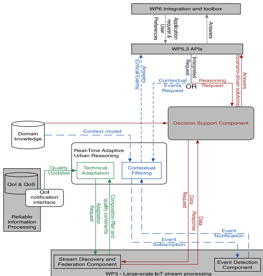
Figure 30: Overview of the Real-time IoT Intelligence Components
