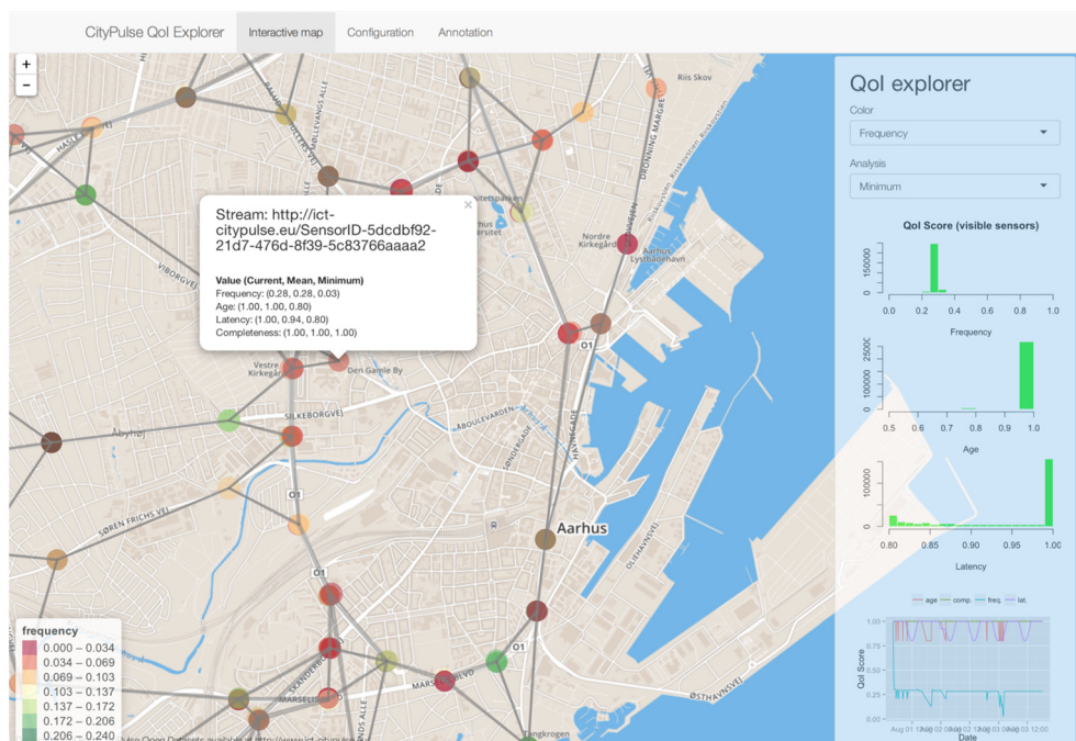
Figure 7: CityPulse Quality Explorer
