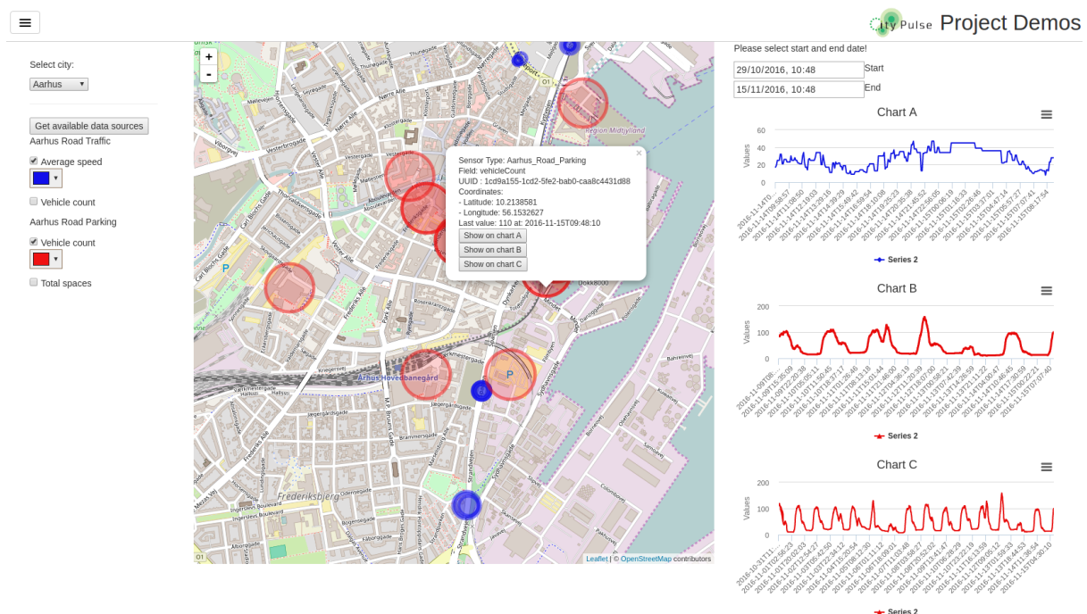
Figure 9: CityPulse Smart City Dashboard
