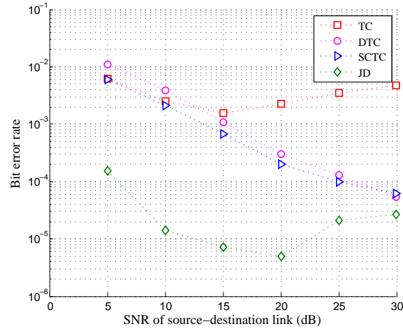
Figure 2.6.: Bit error rate vs. transmit-power normalized by noise for the proposed Stgy. II, where the minimum SINR requirement is set up to \text{SINRT} = 3 .
