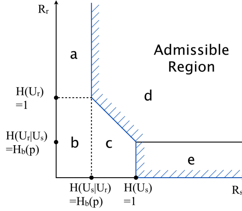
Figure 3.2.: The approximated admissible rate region for S and R determined by the Slepian-Wolf theorem.
