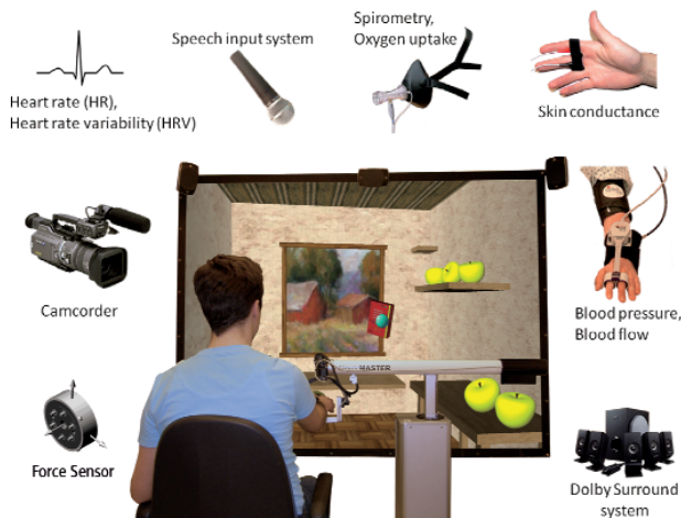
Setup for the upper extremity rehabilitation consists of a HapticMaster® system extended by an immersive multimodal environment and measurements of physiological data.
