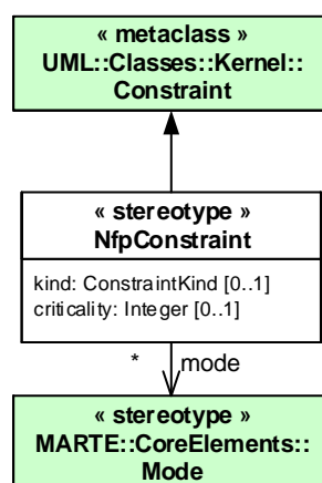
(b) UML view extensions to be proposed to the OMG
