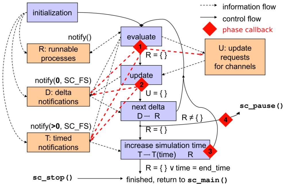
Figure 8: Extended SystemC simulation cycle
