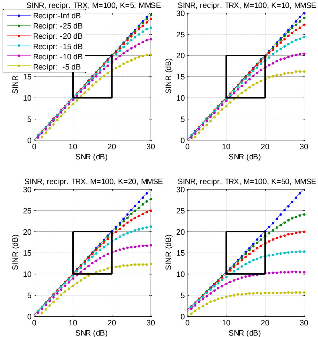
Figure 4 - SINR for non-reciprocal transceivers, MMSE pre-coding
