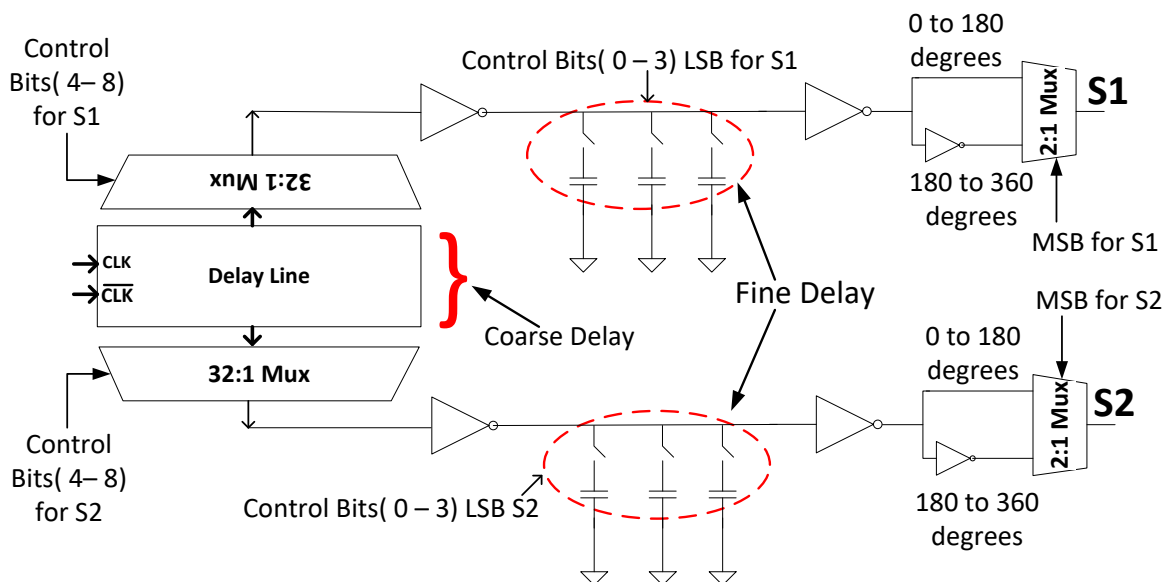
Figure 12 System level view with fine phase-shift varactors
