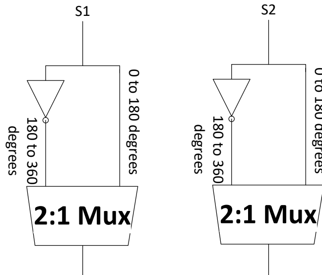
Figure 11 Lower frequency bound extension of delay line
