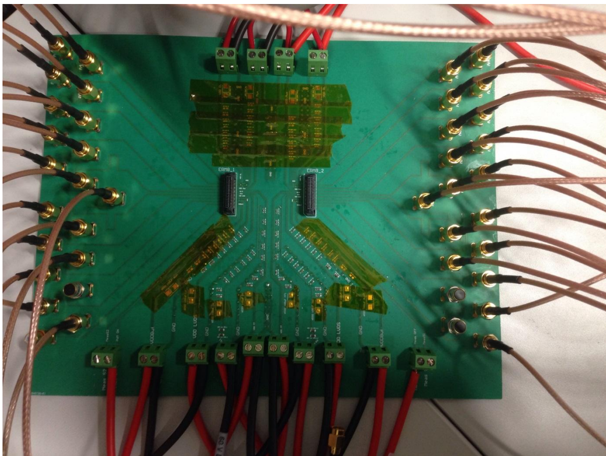
Figure 14 Main PCB
