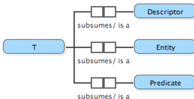
Figure 10.1. The top layer of the Descriptive Upper Ontology
