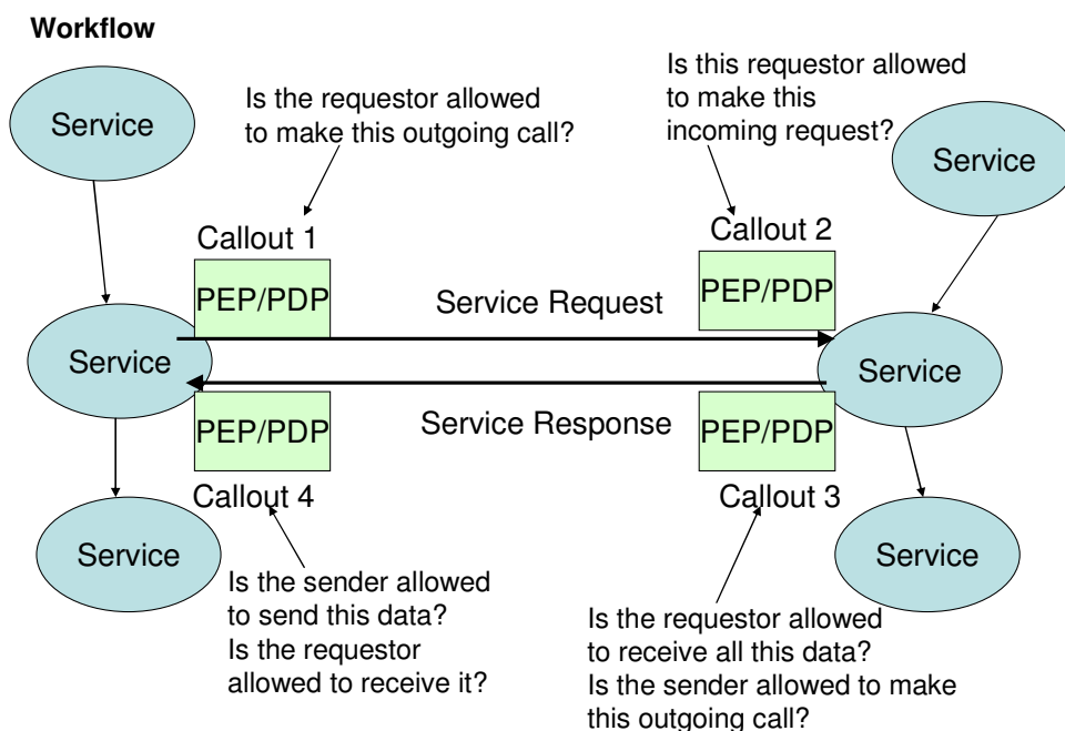
Figure 2.2 Application Callouts to the TAS 3 Authorization Infrastructure
