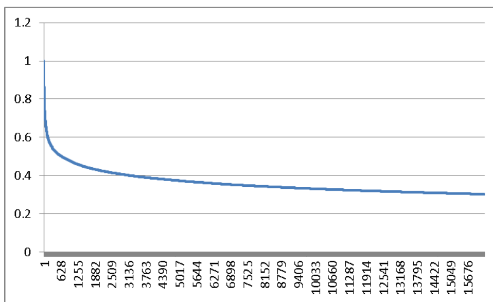
Figure 2: Top 1% of the EMACC document alignment probabilities from the highest to the lowest for the English-German ILSPA Automotive V2 corpus
