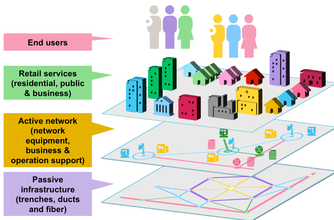
Figure 5 FTTH network layers (Source: FTTH Business Guide 2012 – FTTH Council Europe)
