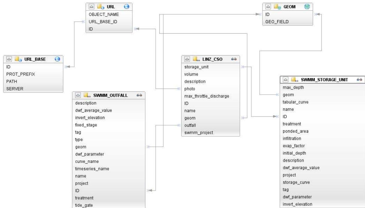
Figure 9: CSO entity modelled in cids Integration Base
