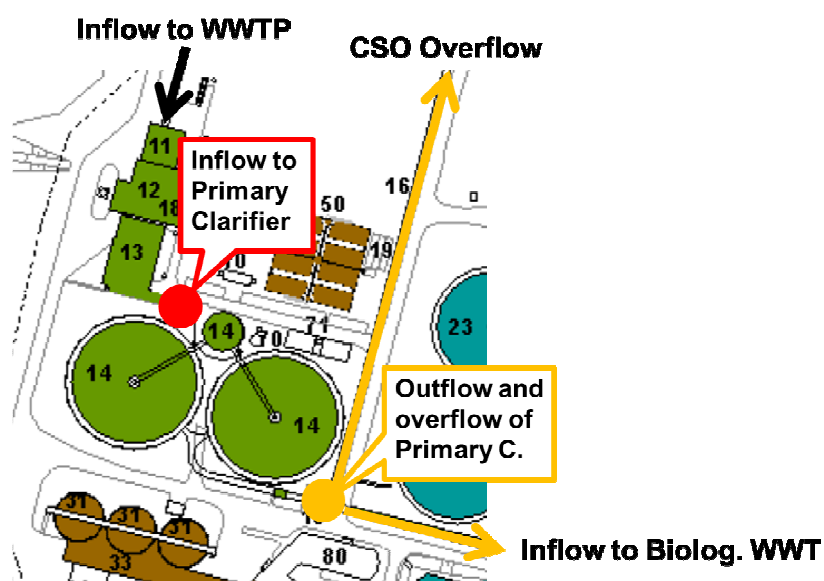
Figure 28: Overview of primary clarifiers at WWTP with inflow, overflow and outflow situation
