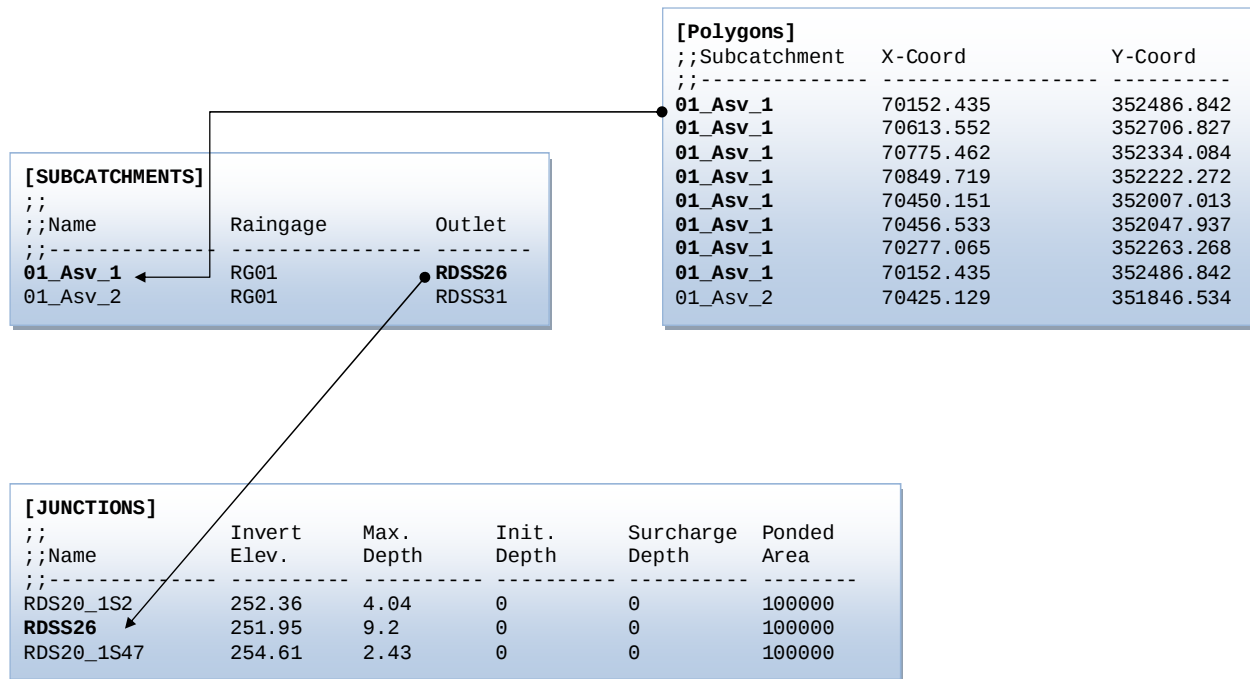
Figure 12: Relationships between entities in the SWMM input file
