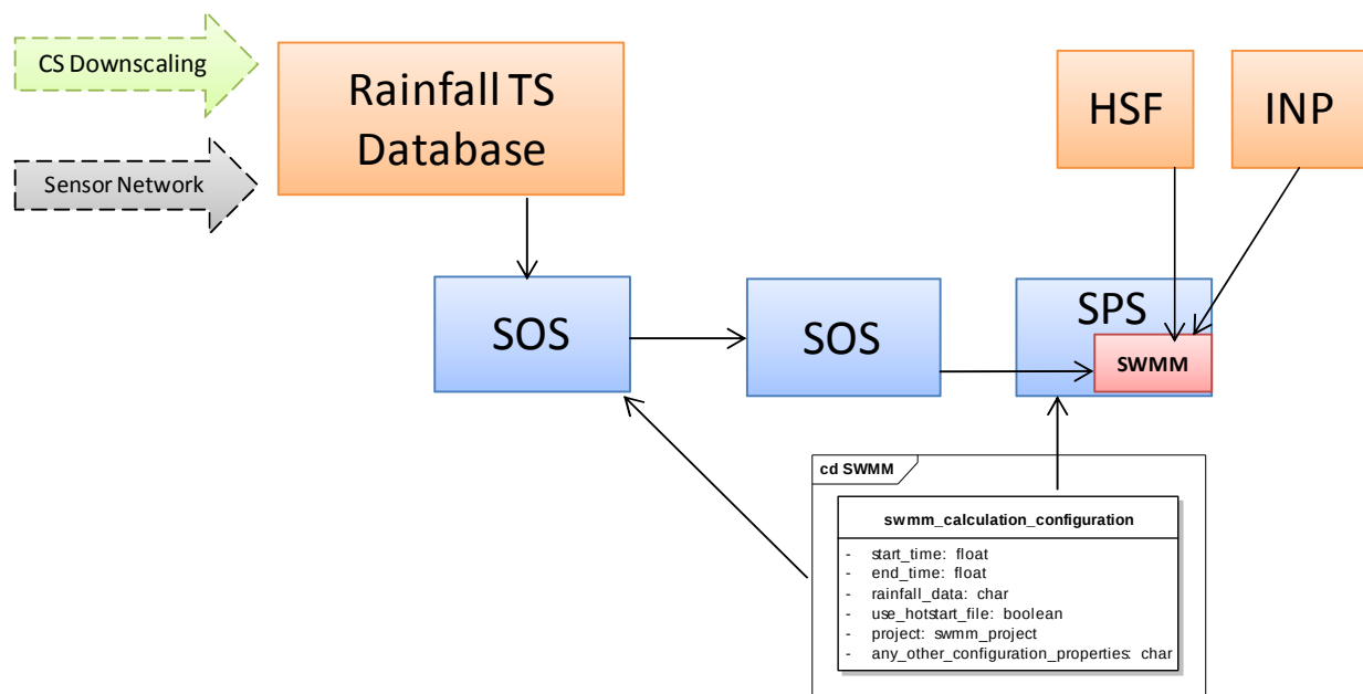
Figure 25: SWMM Model Run Configuration
