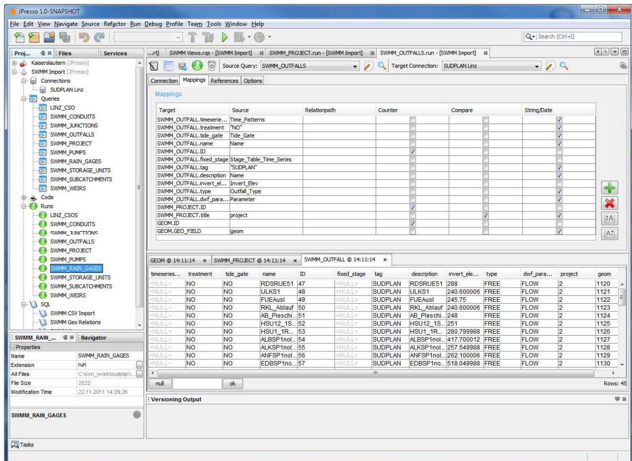
Figure 14: JPresso ETL Tool with SWMM Import Configuration
