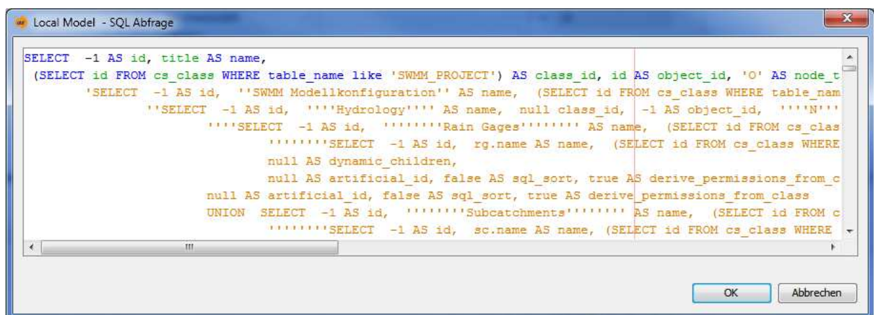
Figure 22: Dynamic Catalogue Configuration
