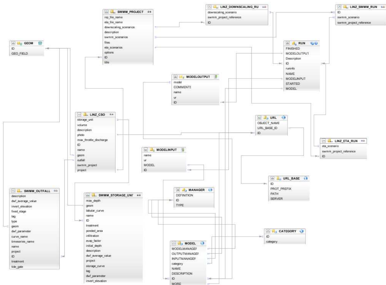
Figure 8: cids Linz Pilot Data Model (excerpt)
