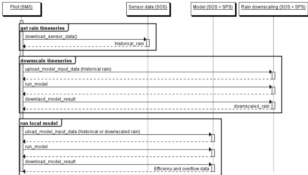
Figure 52: overall workflow between the pilot SMS and the services
