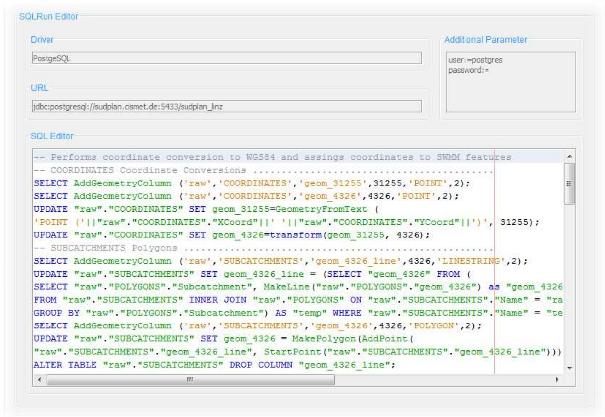
Figure 15: SQL Run Example
