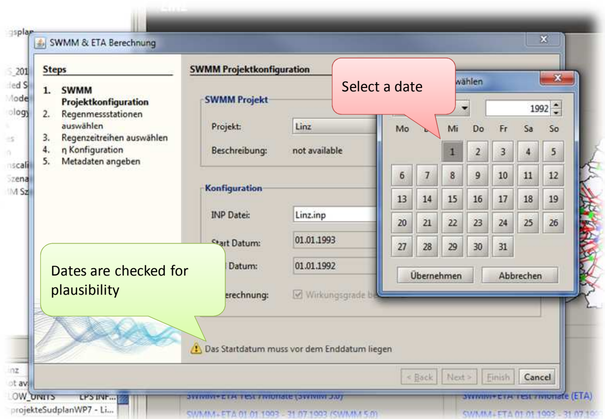
Figure 38: Date Plausibility Check
