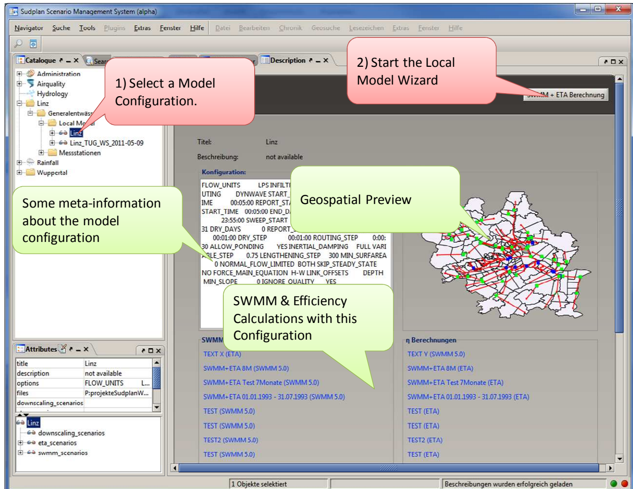
Figure 36: Select Model Configuration and run Local Model
