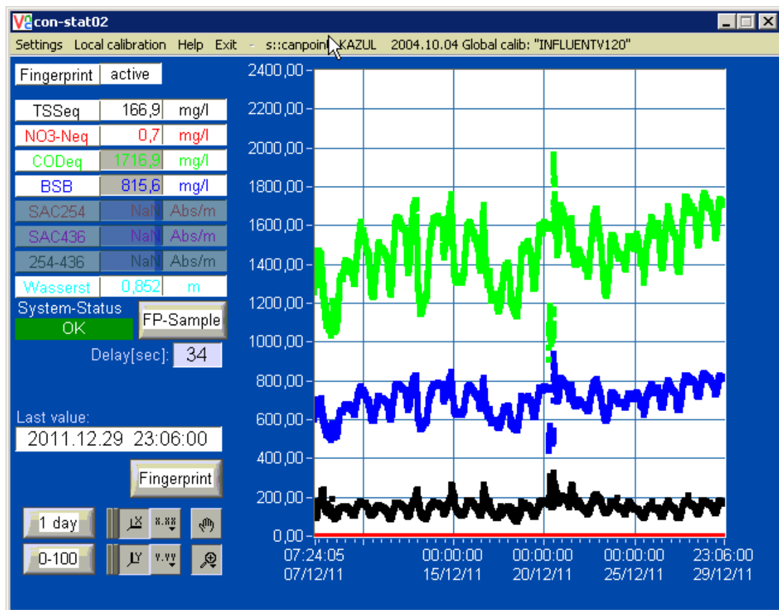
Figure 34: Recorded pollutographs for TSS eq , NO 3 -N eq , COD eq and BSB eq in the outflow channel of the primary clarifiers within a period 22 of days in December 2011
