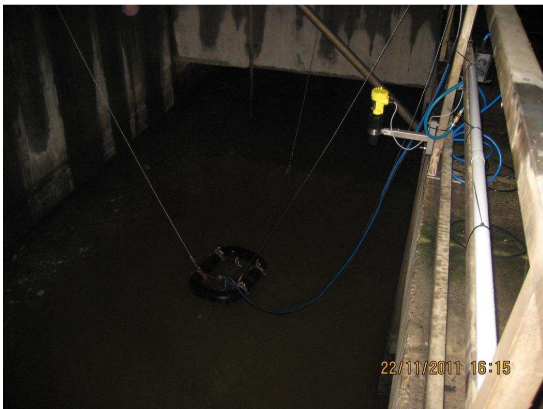
Figure 32: Installation site of the outflow devices (floating UV/VIS spectrometer and ultrasonic device)
