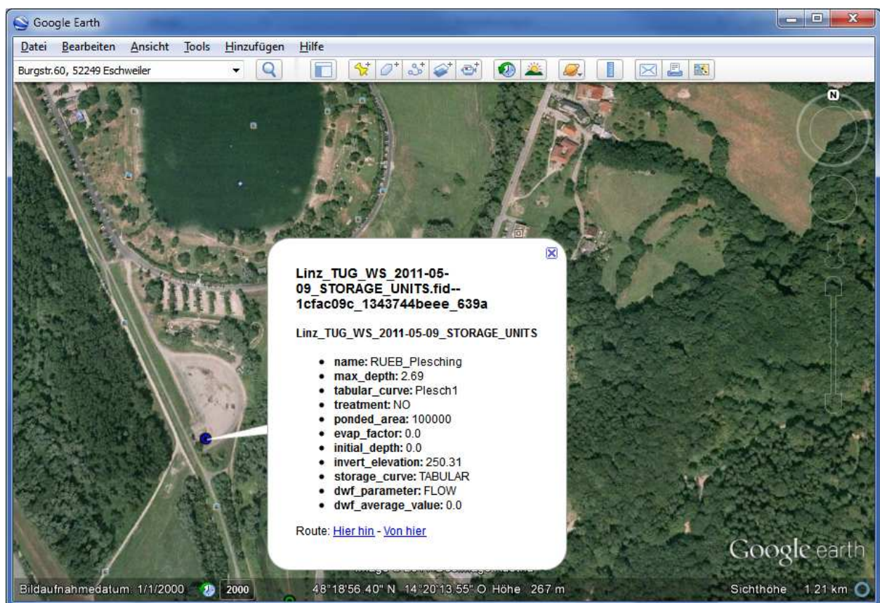
Figure 20: Geospatial Visualisation of a SWMM storage unit in Google Earth
