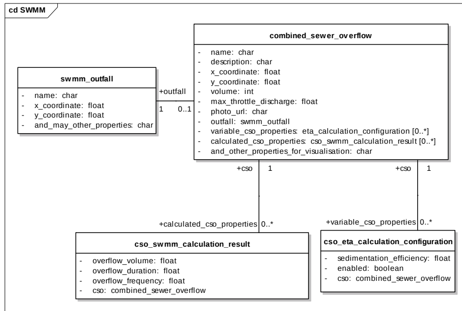
Figure 6: Initial Data Model of the CSO entity
