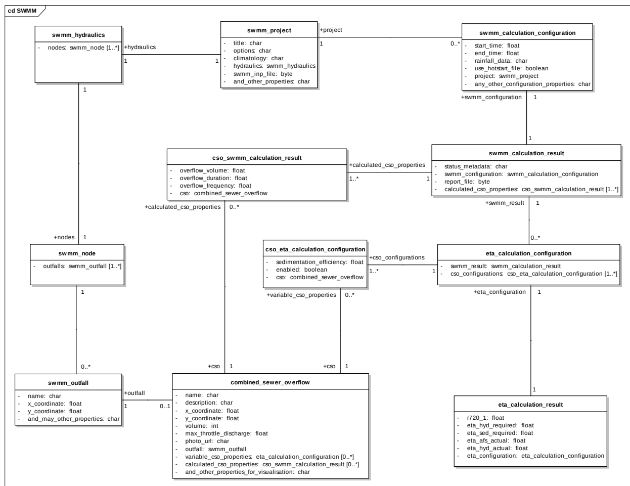
Figure 5: Initial Linz Pilot Data Model (excerpt)
