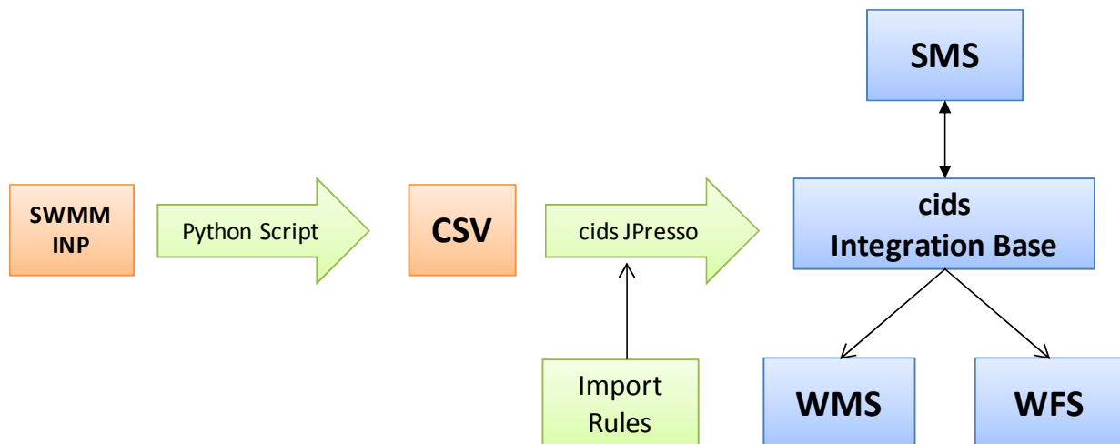
Figure 7: SWMM Model Configuration Import
