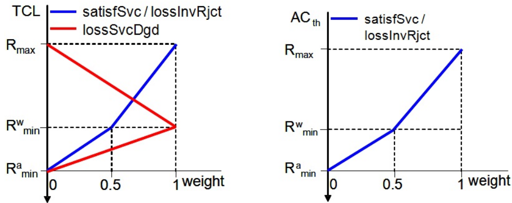
Figure 19: Impact of SLS-S BIs Weights on (a) TCL, and (b) AC Threshold.
