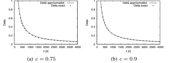
Fig. 6. \Delta optimum (approximated vs exact) for the hypo-exponential delay with target probability p = 0.8 and varying c .
