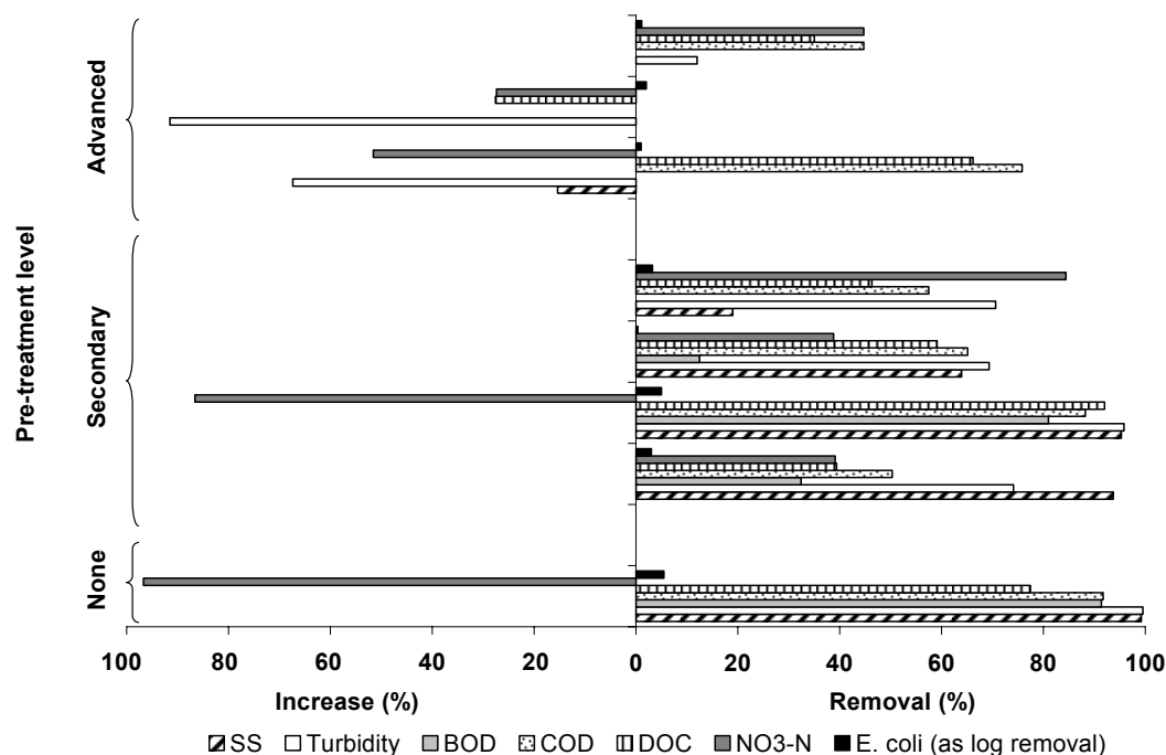
Figure 3.11 Influence of the injectant pre-treatment level on average percentage removals or increase after aquifer recharge at each site.
