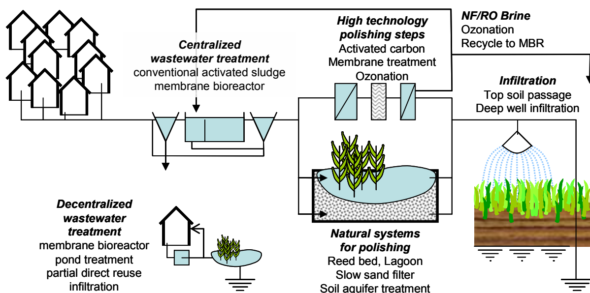
Figure 3.3 Schematic summary of the treatment steps investigated on within WP1
