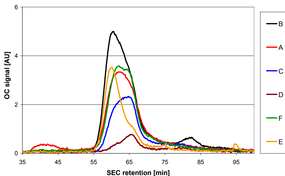
Figure 3.9 DOC characterisation by size exclusion chromatography in abstracted groundwater at six different SAT sites
