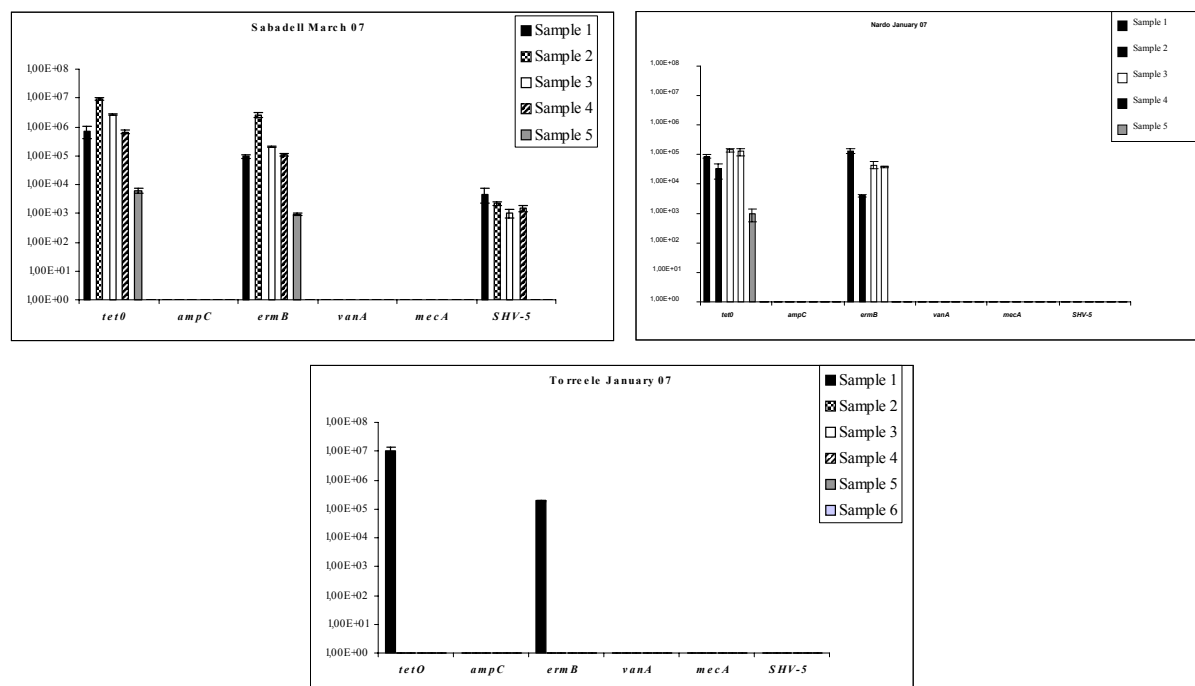
Figure 3.5 Elimination efficiency for antibiotic resistance genes at the artificial groundwater recharge sites (Bockelman et al 2009)
