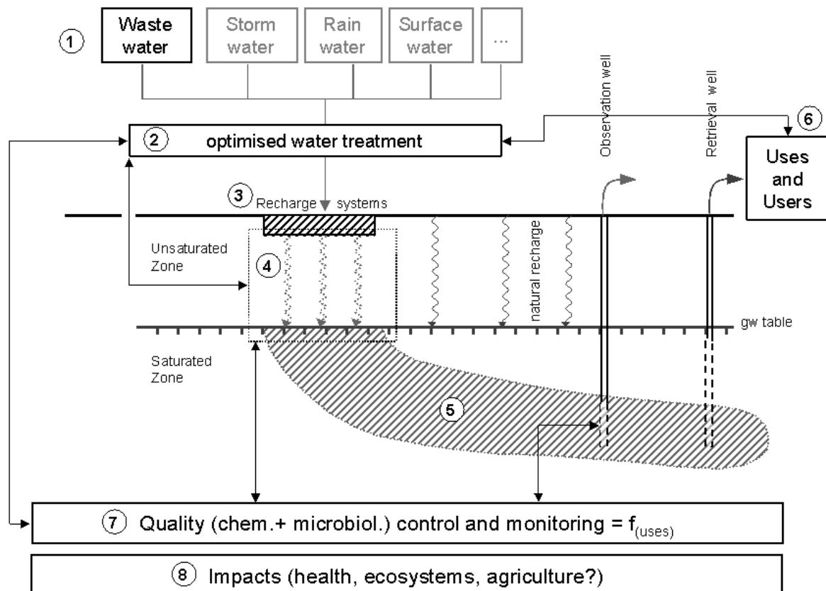
Figure 1.1 Concept of managed aquifer recharge and points of consideration
