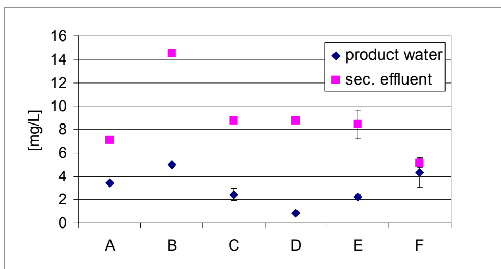
Figure 3.8 DOC of effluent and final groundwater at six different demonstration sites for groundwater recharge
