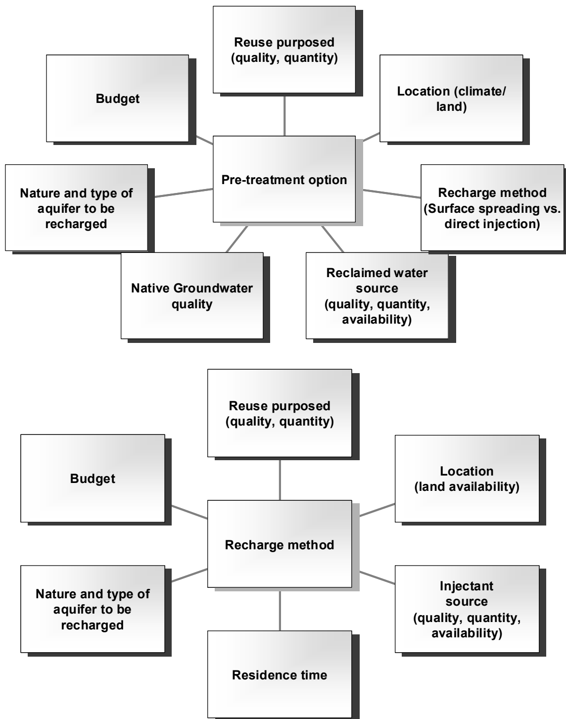
Figure 3.10 Factors affecting pre-treatment and recharge method choices for aquifer recharge of reclaimed effluent.
