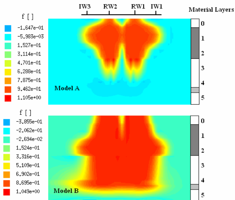
Figure 3.13 Vertical distribution of the mixing fraction for model A and model B showing the extent of the fresh plume within the aquifer after injection through RW wells (from Kremer et al. 2008). Horizontal scale is about 250 m while vertical scale is 50 m. A and Model B and differ in terms of the degree of vertical leakage of recharge water into the underlying low permeability layers, which is significantly higher in model B, and in the porosity values with 0.7 for model A while 0.25 (more realistic than A) for model B. Both models A and B were found to fit the field data equally well but result in very different solute distribution profiles.
