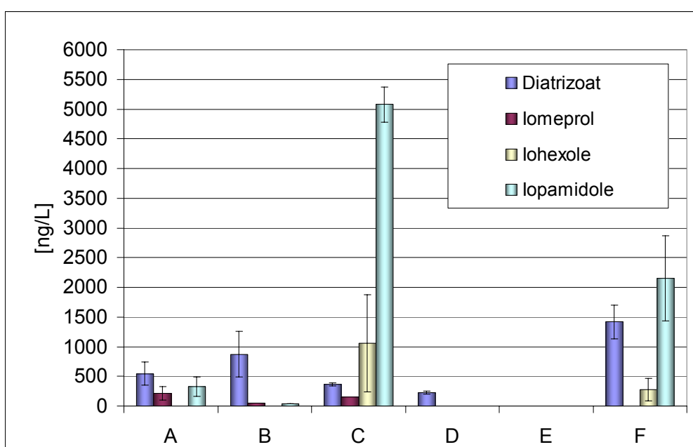
Figure 3.7 Product well ICM concentration at six SAT sites
