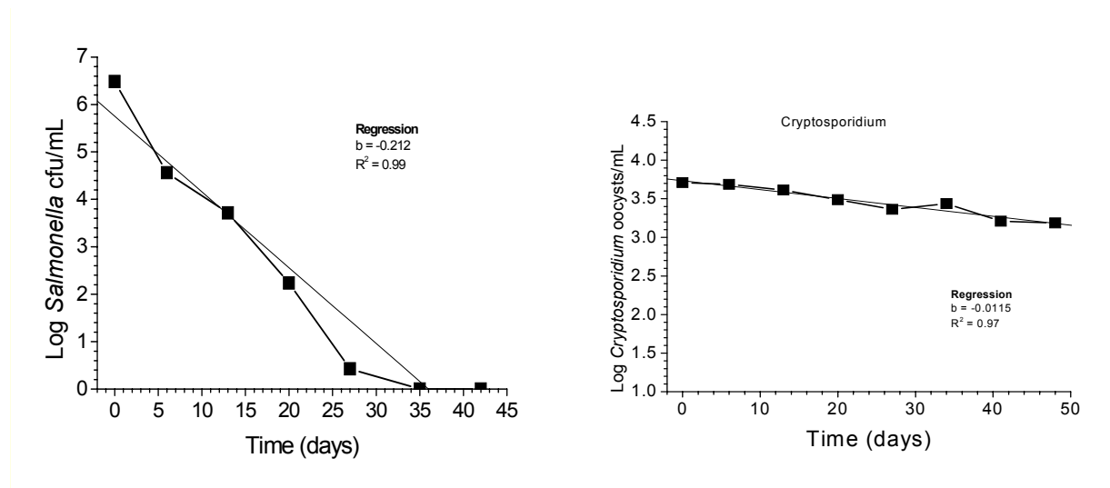
Figure 3.6 Decay slopes and corresponding regression lines for S. typhimurium cells and Cryptosporidium parvum oocysts in decay chambers
