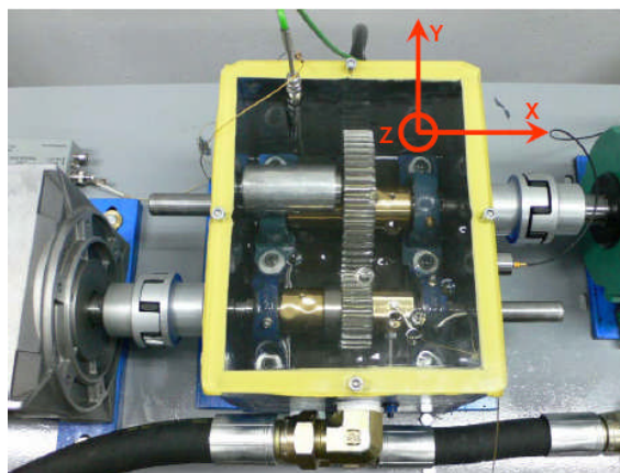
Experimental gear box set up
