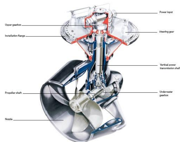
Figure 8: Schottel Rudder-propeller
