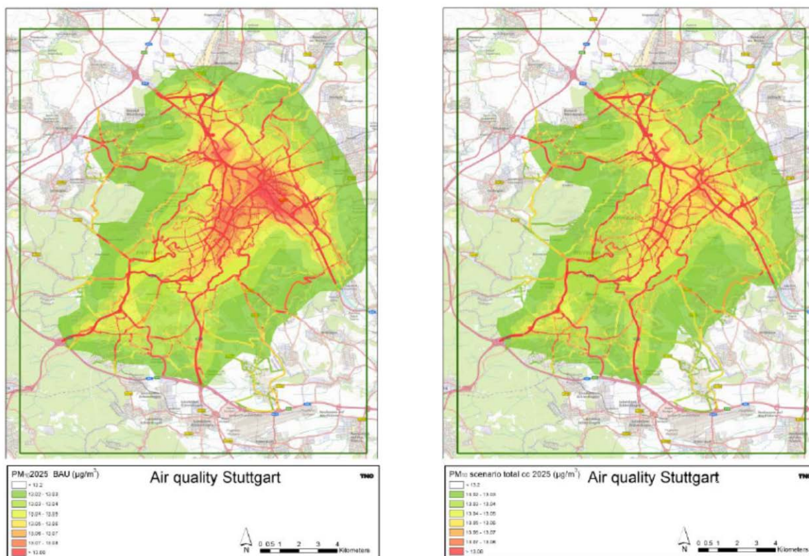
Figure 8 PM 10 concentrations in Stuttgart comparing local transport emissions for BAU (left) with the four reduction measures implemented by 2025 (N.B. pollution stemming from sources outside of Stuttgart and from other sources than transport are not taken into account)
