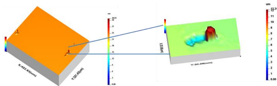
Figure 6.4 Measured surface containing significant defect exploded defect view. In situ coated film measurement, inset image 50 x 25um
