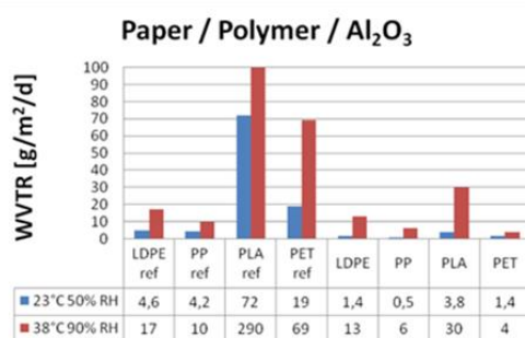
Figure 2.7 Improvement in WVTR for polymer substrates with ALD coating
