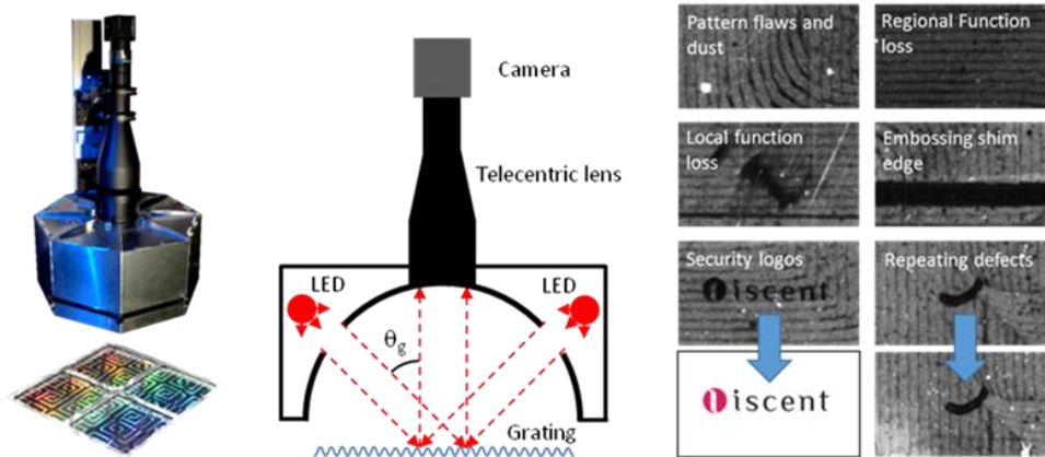
Figure 5.3 Implementation of the Fourier filtered imaging system (left). Schema of the system (centre). Examples of features and defects that can be resolved by image contrast.
