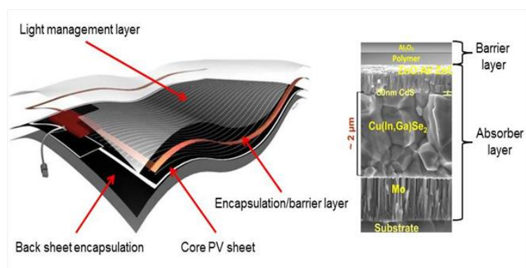
Figure 3.2 Function layers in flexible PV substrates (courtesy Flisom)
