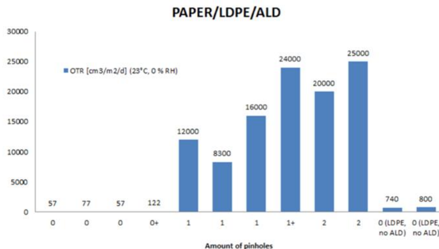
Figure 3.6 OTR levels through simulated defects in Paper/LDPE/ALD substrate
