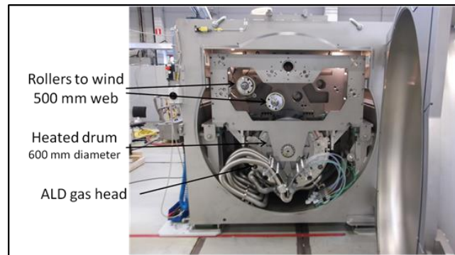
Figure 2.3 – R2R ALD tool (inside vacuum chamber)
