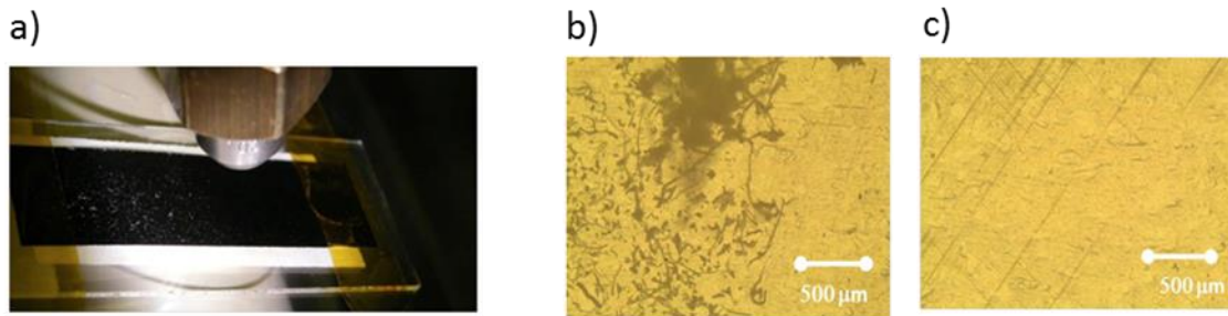
Figure 4.4 a) N 2 gas nozzle on R2R line at TNO b) coated paper pre-cleaning c) post-cleaning
