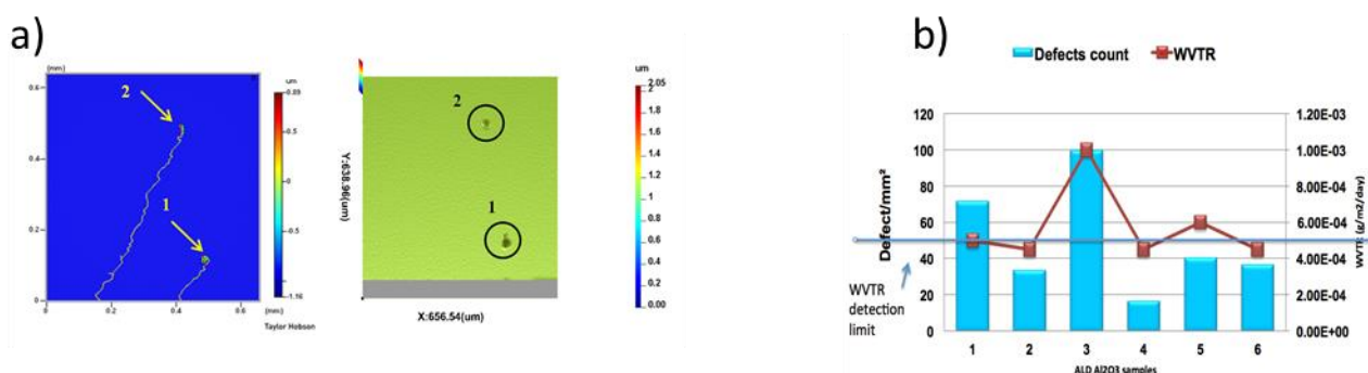
Figure 3.3a) 2 segmented defects extracted from surface measurement data b) and significant defect values density versus WVTR value
