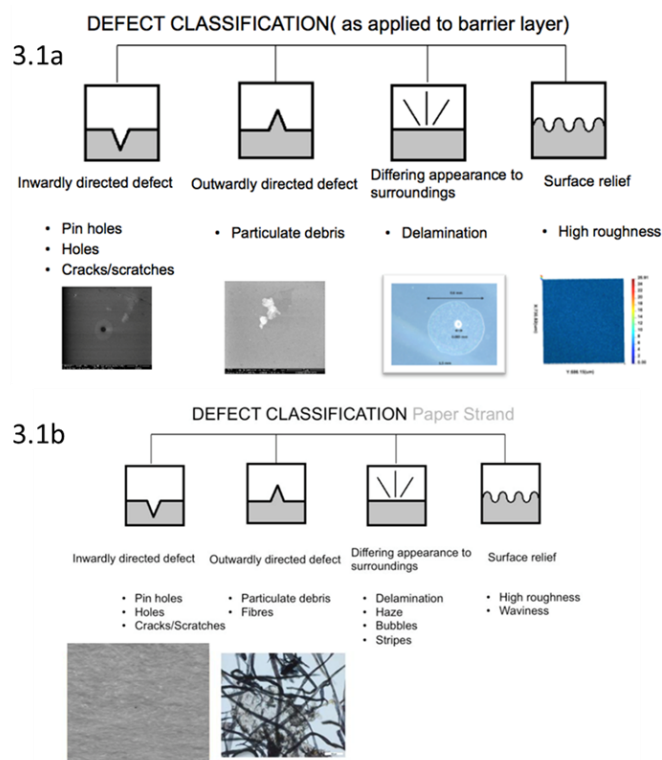
Figure 3.1 Defect classification system a) for barrier layers (CPI) b) Polymer coated paper (TUT, SE)
