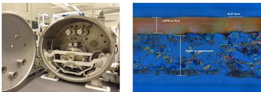
Figure 2.6 Beneq WCS 500 roll-to-roll ALD reactor at LUT Cross profile from fibre/polymer/ALD structure
