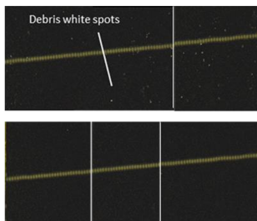
Figure 4.3 Optical microscope images of scribed Mo film with redeposited Mo particles before and after ( 1 \text{ l min}^{-1} N 2 gas jet cleaning at a nozzle – substrate angle of 45°, a distance of 2 cm and a web speed 2 m/min.
