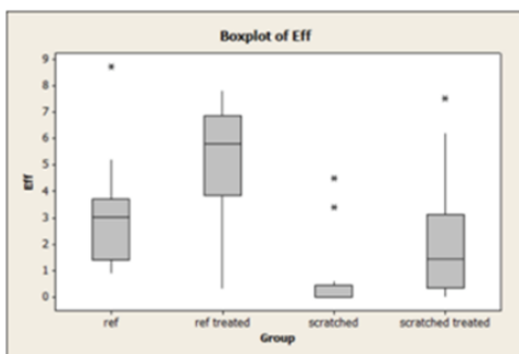
Figure 4.5 Box plot of efficiency of repaired poor quality cell compared to reference cell
