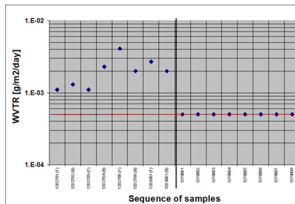
Figure 2.4 – 40nm barriers: pre-clean improvement
