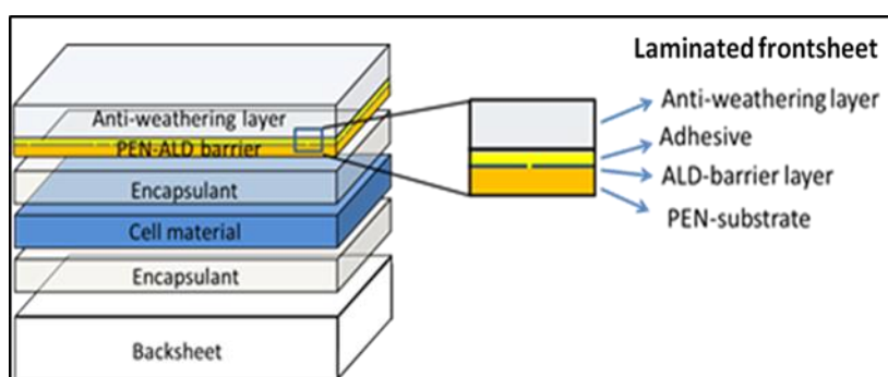
Figure 2.2 – Cross section of the Isovoltic frontsheet including produced ALD barrier layer
