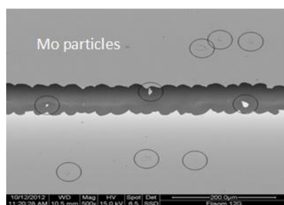
Figure 4.1 PV scribe line Figure
