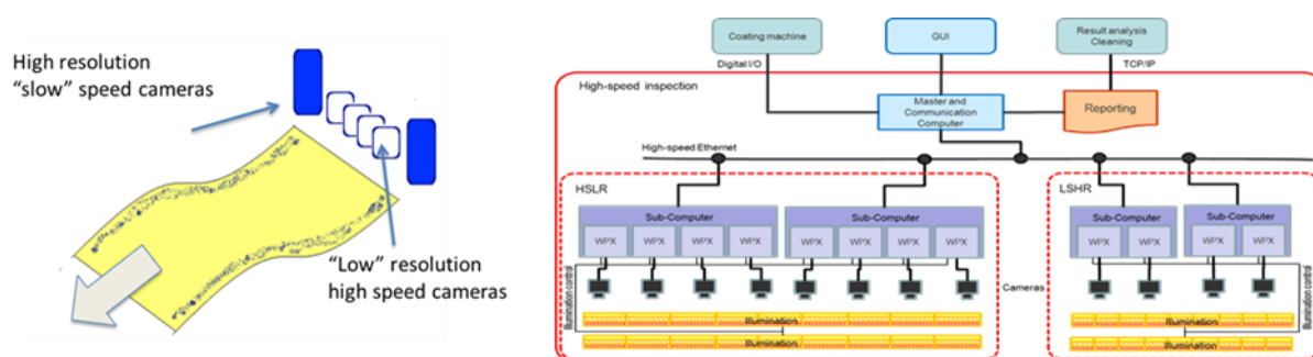
Figure 5.4 a) Schematic setup of the hybrid system at TUT b) Computer hierarchy adopted to deal with high data rates
