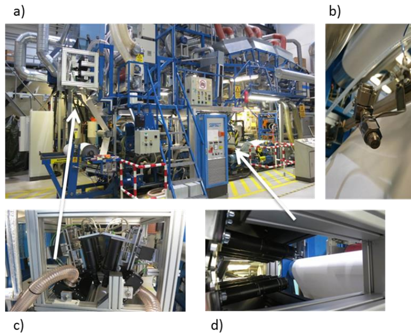
Figure 6.1 a) Pilot production line at TUT b) N2/pressurised air cleaning nozzle c) centre zone substrate inspection system d) edge zone inspection system
