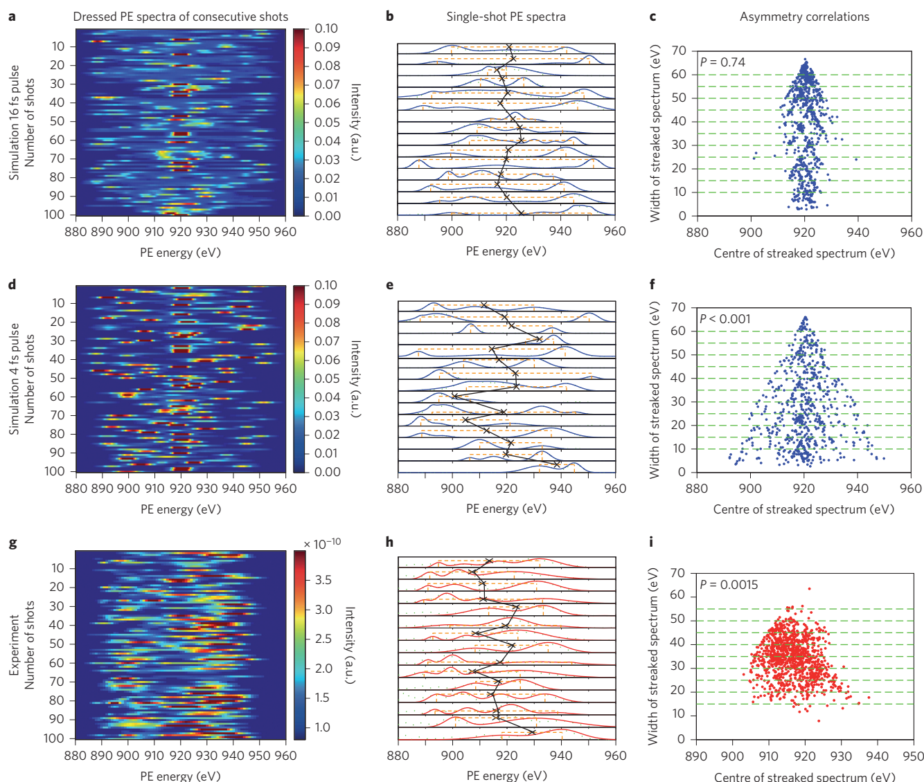
Figure 2 | Dressed single-shot X-ray photoelectron spectra and correlation plots. a–i , Simulations (blue, a–c , d–f ) for the sideband regime with 16 fs FEL pulses ( t_{\text{period}}/t_{\text{X-ray}} = 1/2 , a–c ) and for the streaking regime with 4 fs FEL pulses ( t_{\text{period}}/t_{\text{X-ray}} = 2 , d–f ) are compared with experimental findings ( g–i , red). On the left ( a,d,g ), colour-coded intensity images of 100 consecutive dressed photoelectron (PE) spectra are plotted. In the middle ( b,e,h ), 15 single-shot spectra are extracted for the three cases. For each, the spectral width (orange, dashed lines) and centre position (black crosses) are marked, with black lines connecting the centres of consecutive spectra. On the right, the centre positions and widths of the spectra for 1,000 simulated shots ( c,f ) and for the experimental data ( i ) are mapped out in correlation scatter plots.
