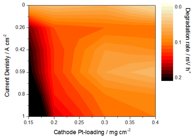
Figure 15: Pseudo 3D plot showing the irreversible degradation rate (color scale) versus current density and cathodic Pt-loading. The degradation values at loadings 0.15, 0.20, 0.30, 0.4 \text{mg}_{\text{Pt}} \text{cm}^{-2} are real experimental data; the values at loadings 0.25 and 0.35 \text{mg}_{\text{Pt}} \text{cm}^{-2} are interpolated data.
