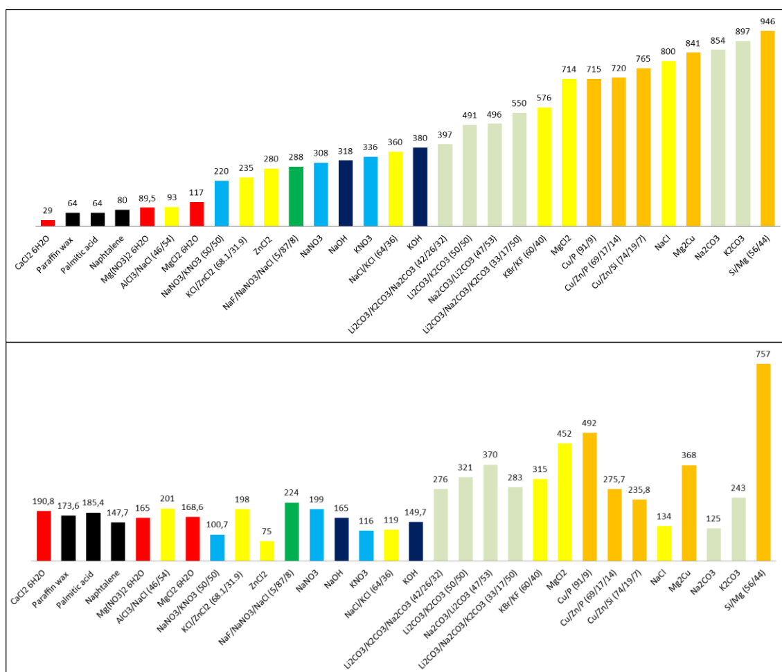
Figure 37. Phase change (melting) temperatures (above, in ^\circ\text{C} ) and latent heats (below, in \text{J/g} )
