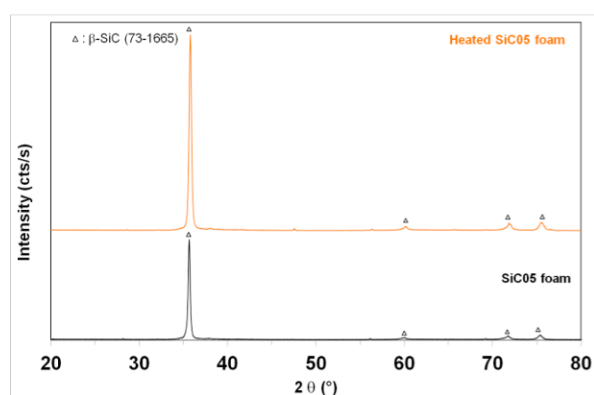
Figure 22. Diffraction patterns collected for no-heated and heated sample SiC05: -SiC (triangle).
