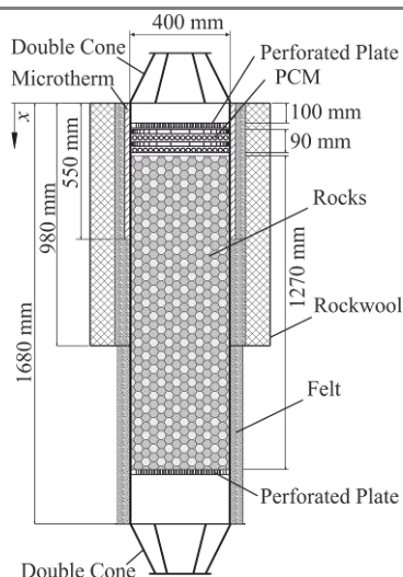
Figure 36. Configuration of the 42 kWhth lab-scale prototype used in the ETH experimental campaign.
