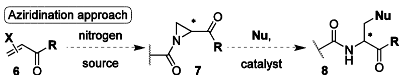
Scheme 1 New methods for the formation of peptide bonds
