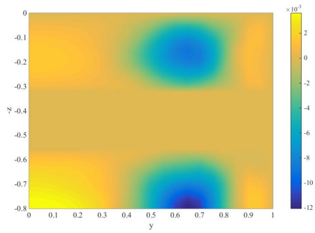
Fig. 1 Higher order term of the velocity potential during the steep wave impact on a plate with an intermediate open area.
