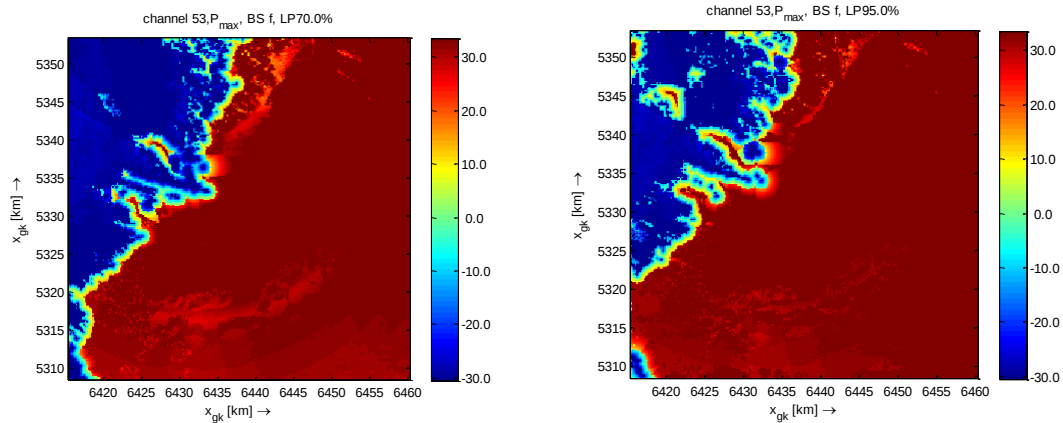
Figure 20 P_{\text{wsd,max}} in case of 70% (left) and 95% coverage protection area.
