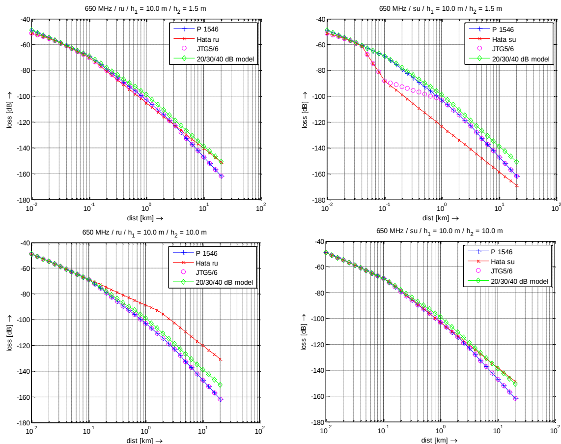
Figure 13 Analysis of propagation models.
