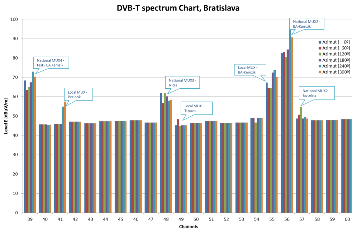
Figure 5 Average field strength in Bratislava area (azimut 0°, 60°, 120°, 180°, 240° and 300°).
