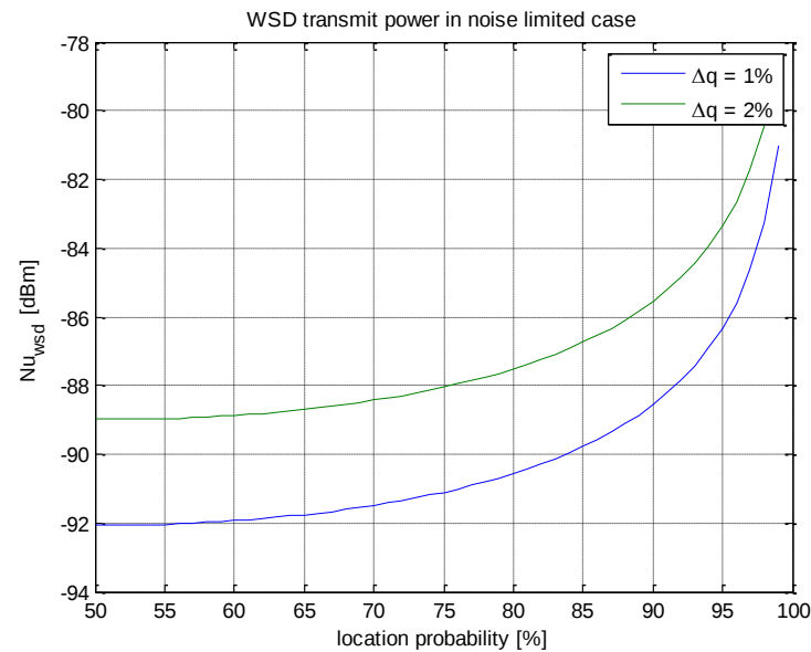
Figure 26 Increase in Nu_{wsd} due to higher degradation
