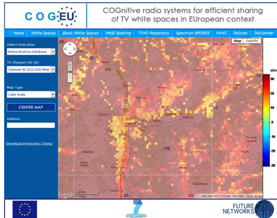
Figure 40 P_{wsd,max} for channel 40 in the Banská Bystrica region (20x30 Km).
