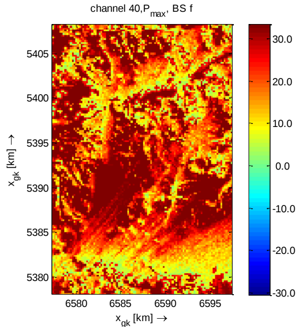
Figure 18 P_{\text{wsd,max}} for Channel 40 in the Banska Bystrica region.
