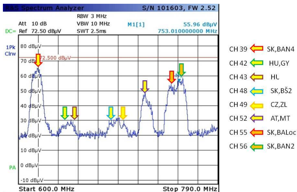
Figure 4 Example of a spectrum analyser screen shot in the urban scenario of Bratislava.
