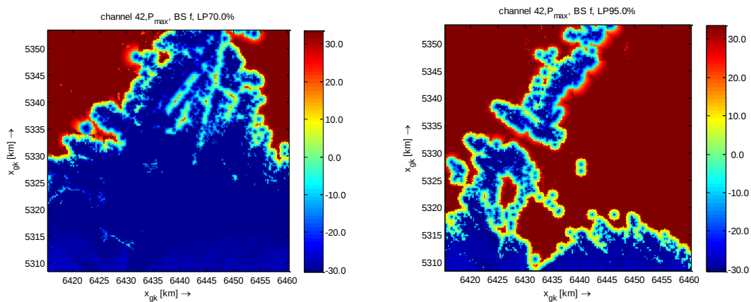
Figure 21 Smooth transition of location probability causes differences in P_{\text{wsd,max}} in large areas.
