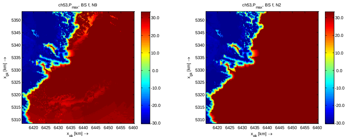
Figure 29 P_{\text{wsd,max}} in ch53 for Bratislava region for N_{\text{adj}} = 9 and N_{\text{adj}} = 2
