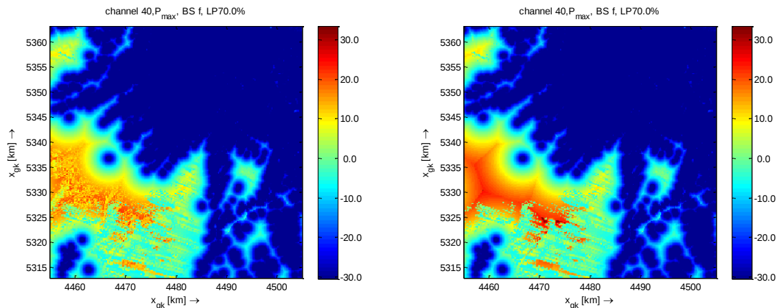
Figure 31 Difference in P_{wsd,max} for N_{adj} = 9 (left) and N_{adj} = 2 (right)
