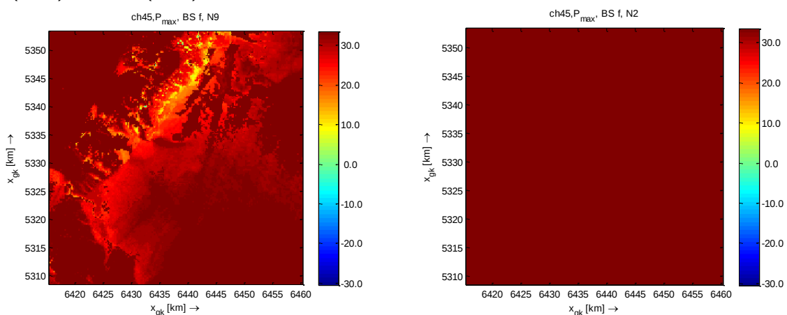
Figure 28 P_{wsd,max} in ch45 for Bratislava region for N_{adj} = 9 and N_{adj} = 2
