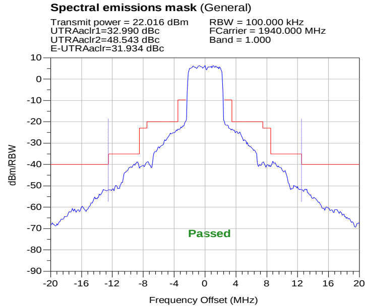
Figure 27 Emission spectrum provided by Nokia (source: SE43(10)89)
