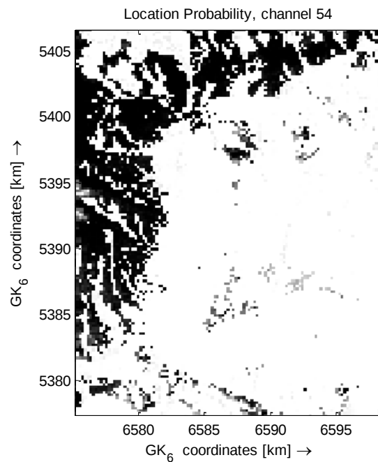
Figure 16 Location probability for Channel 54 in the Banska Bystrica region.
