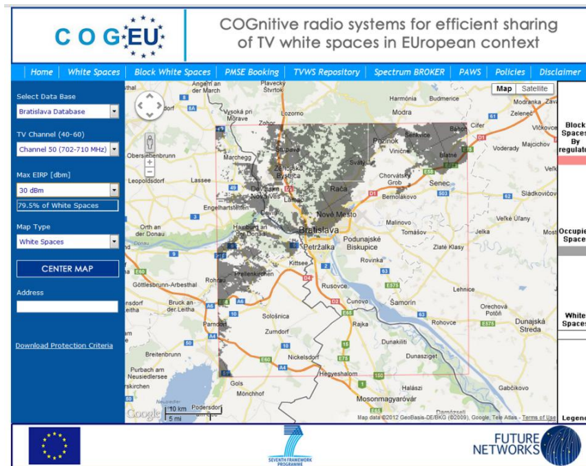
Figure 38 White spaces map for channel 50 in the Bratislava region. The white areas inside the red square are locations where WSDs transmission is possible with transmit power higher than 30 dBm (meaning 79% of the considered area).
