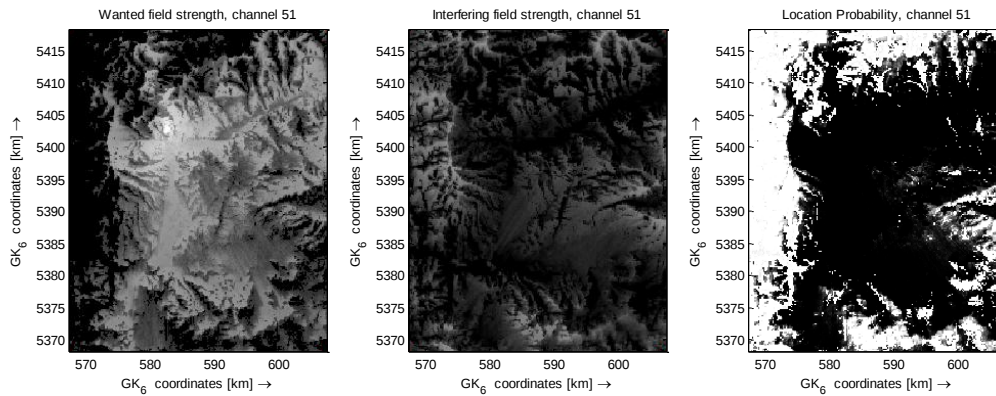
Figure 12 Wanted and unwanted field strength and location probability for channel 51 in the Banska Bystrica region
