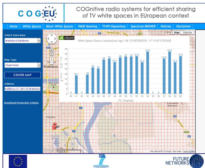
Figure 39 Chart point map for the Bratislava database. In the geo-pixel marked with red 13 vacant channels allow more than 30 dBm for WSD operation, total of 104 MHz are free.
