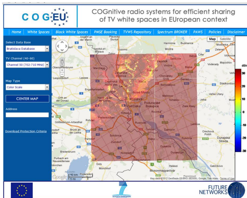
Figure 37 P_{wsd,max} for channel 50 in the Bratislava region (50x50 Km).
