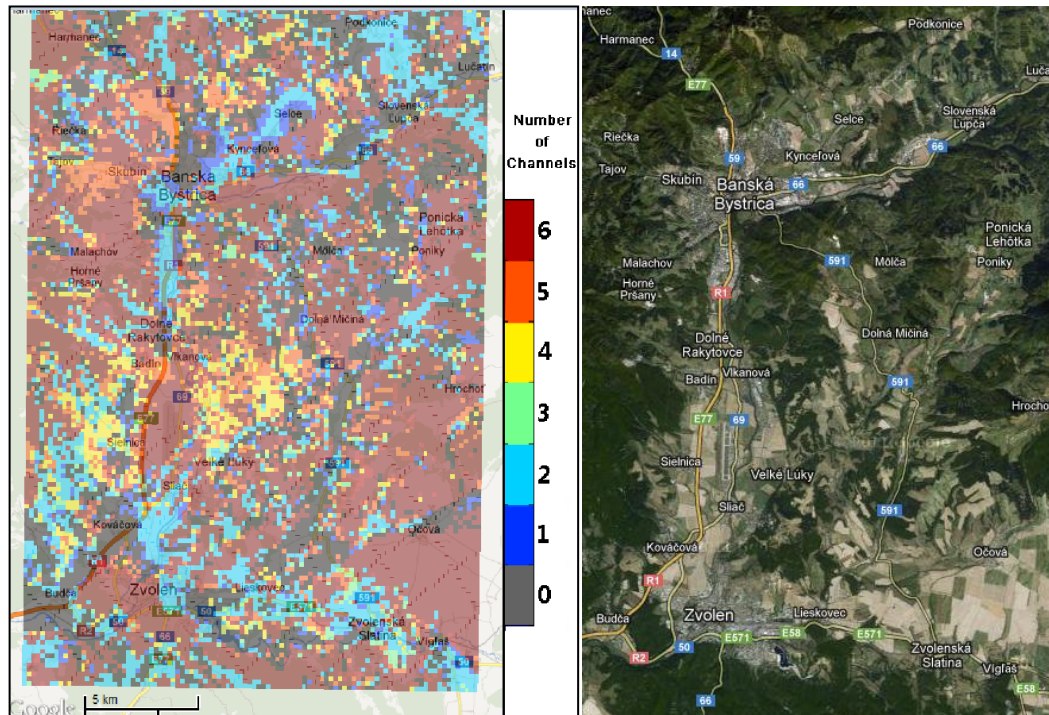
Figure 34 Number of available channels where the max allowed power is higher than 30 dBm for the mountain area of Banská Bystrica.
