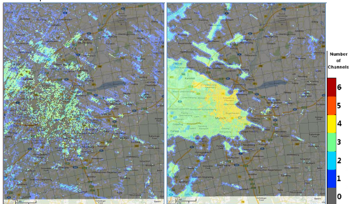
Figure 32 Available channels in Munich area for 'more restrictive' and 'less restrictive' protection of DVB-T.
