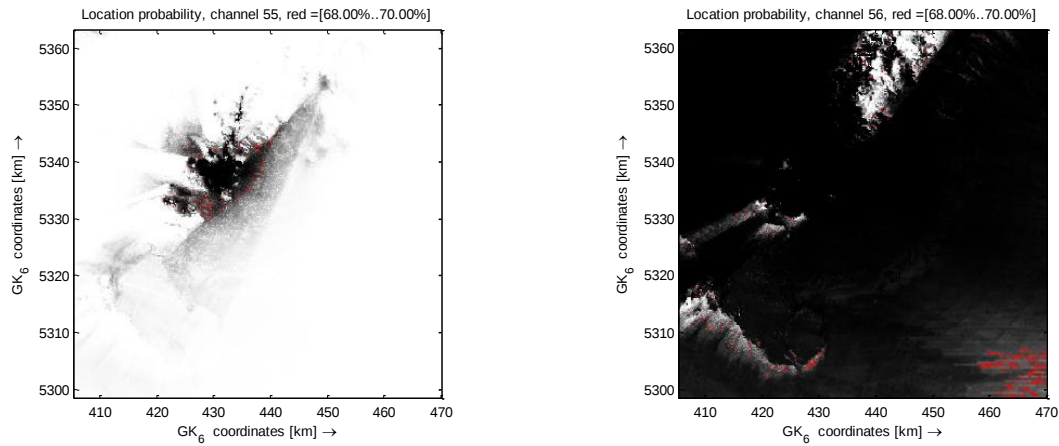
Figure 24 Location probability in Bratislava region for ch55 and ch56
