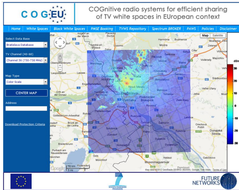
Figure 36 P_{wsd,max} for channel 56 in the Bratislava region (50x50 Km).
