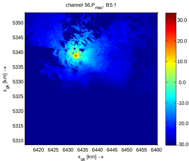
Figure 19 P_{\text{wsd,max}} for channel 56 in the Bratislava region.
