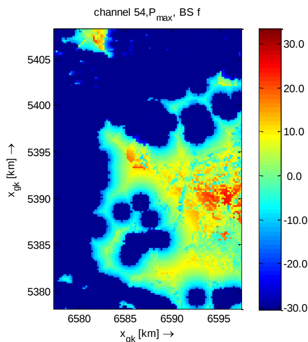
Figure 17 P_{wsd,max} for Channel 54 in the Banska Bystrica region.
