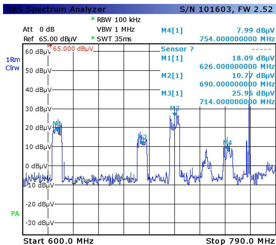
Figure 8 Example of a spectrum analyser screen shot in the rural scenario of Poniky (15 Km from Banska Bystrica).
