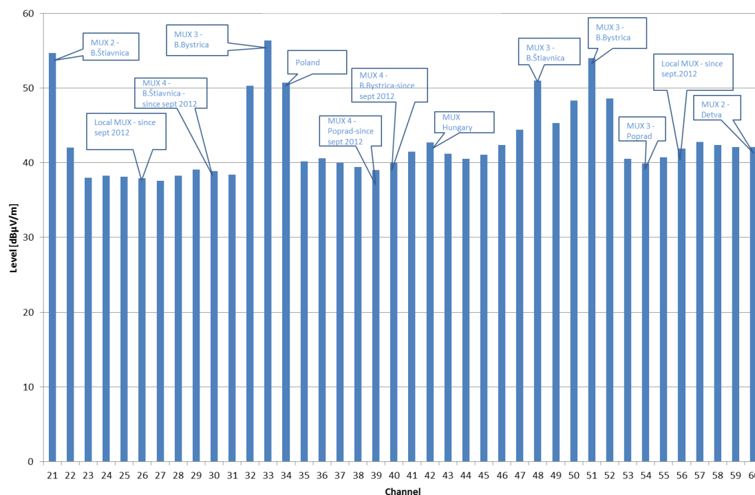
Figure 10 Average field strength in Banka Bystrica area.
