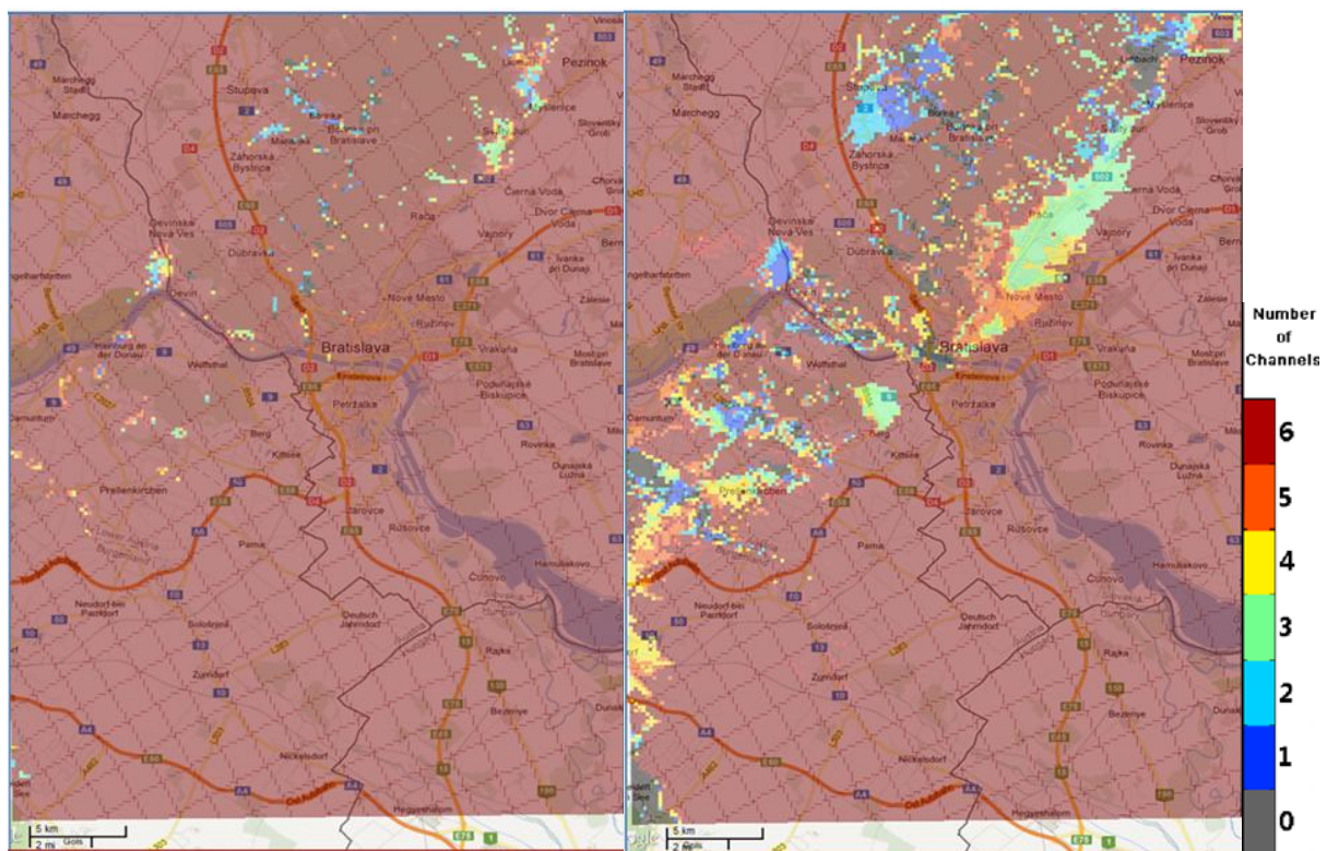
Figure 33 Available channels in Bratislava for max WSD 20 dBm (left) and 30 dBm (right)
