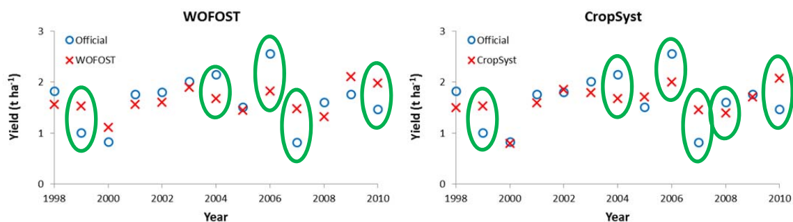
Figure 29 Multi-model soft wheat monitoring in Nord Ouest region; decade: 3 before maturity.
