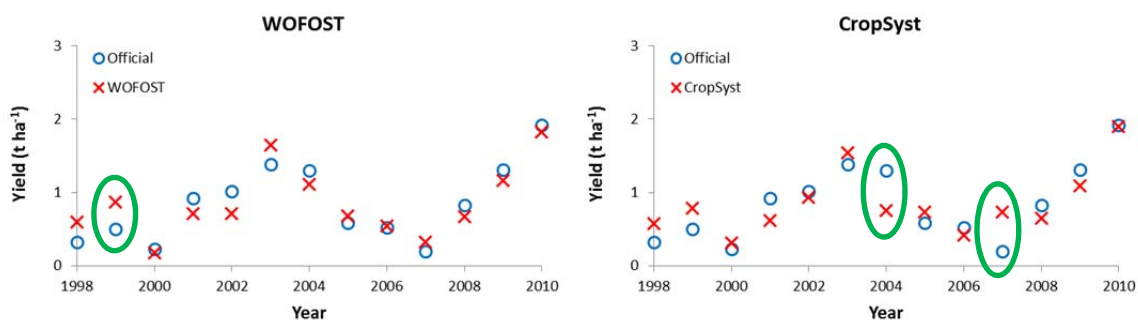
Figure 6 Multi-model durum wheat monitoring in Oriental region; decade: maturity.
