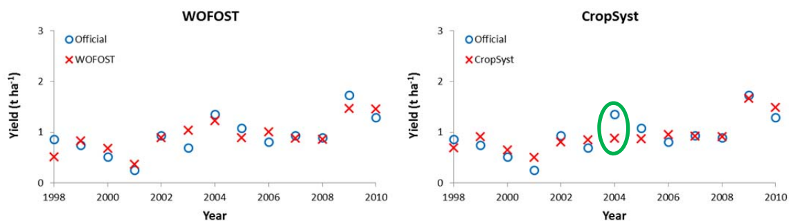
Figure 31 Multi-model soft wheat monitoring in Sud region; decade: 3 before maturity.
