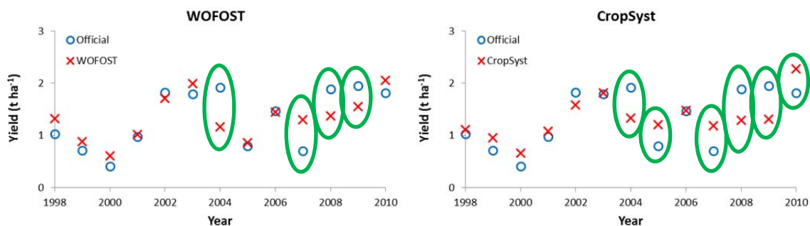
Figure 12 Multi-model durum wheat monitoring in Centre Sud region; decade: 3 before maturity.
