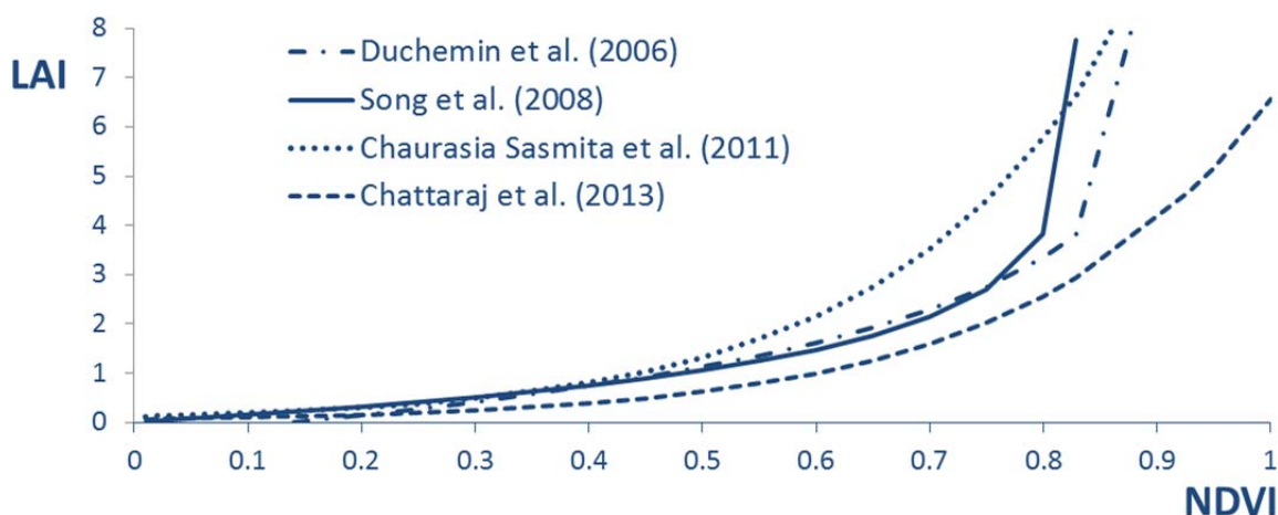
Figure 1: Leaf area index (LAI, m^2 m^{-2} ) values computed as a function of NDVI with the four alternative methods tested.
