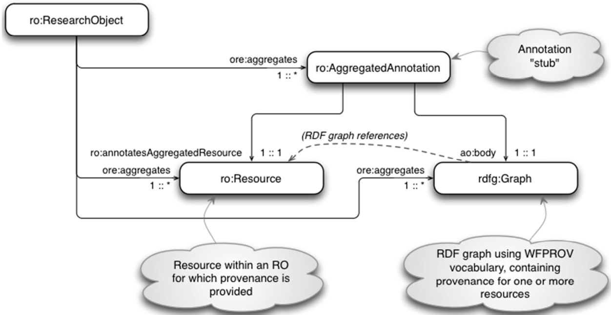
Figure 1 Provenance of workflow results
