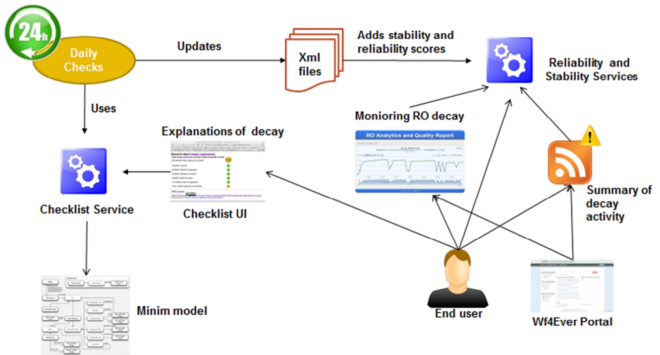
Figure 18 Wf4Ever quality assessment components interactions
