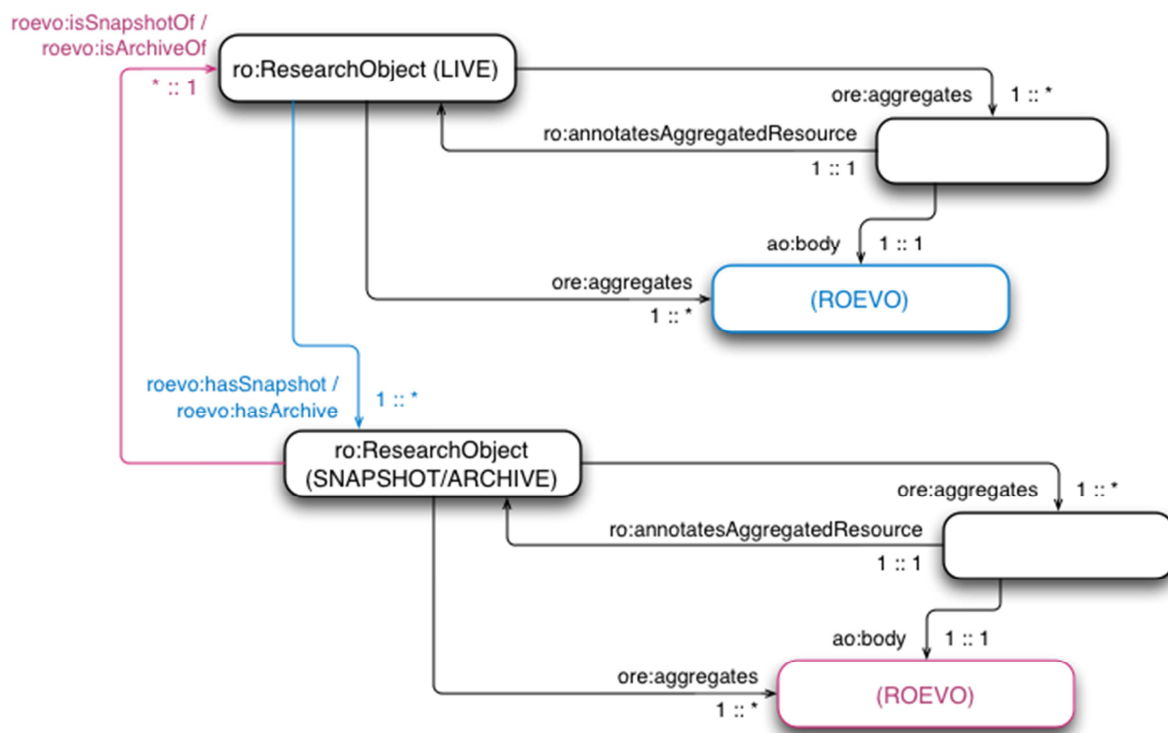
Figure 2 roevo provenance diagram
