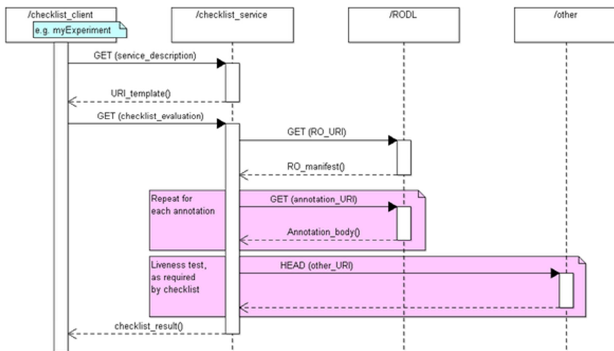
Figure 15 Sequence diagram of the checklist service.
