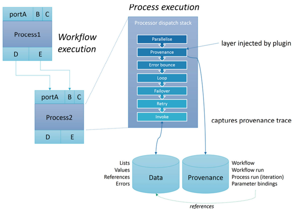
Figure 3 Taverna provenance architecture.
