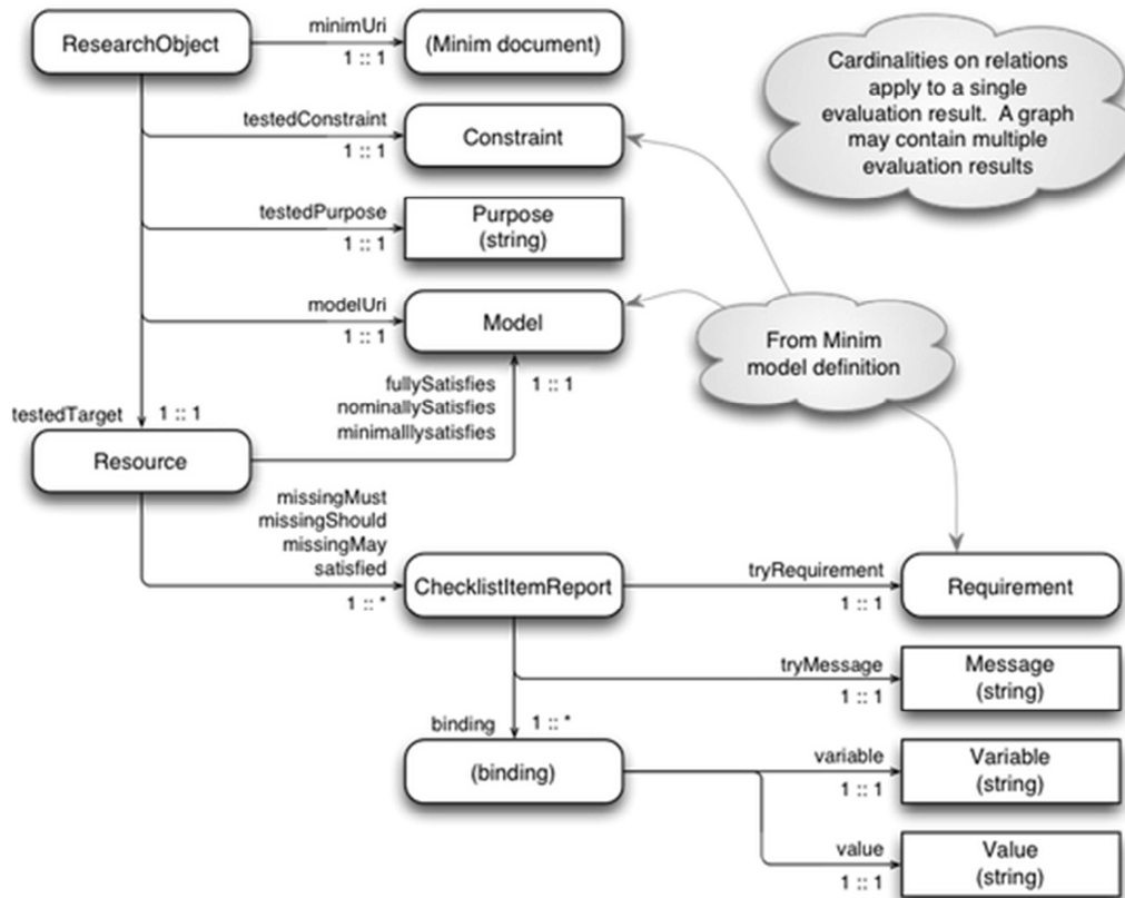
Figure 12 Minim Results Model
