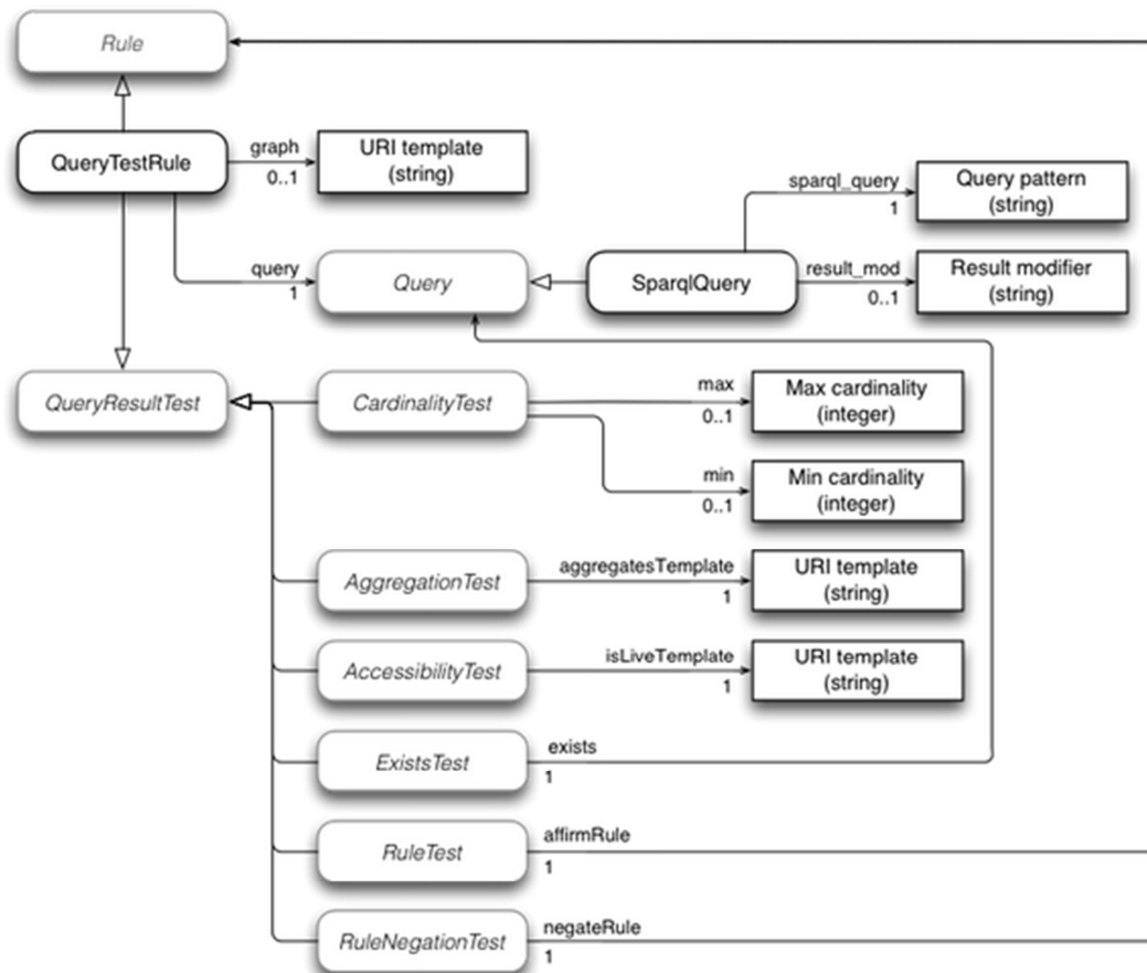
Figure 11 Rule Model Diagram
