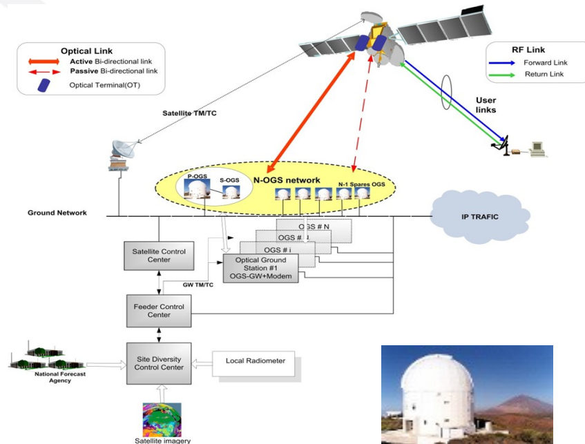
Figure 3.4/C : A typical satellite broadband system relying on optical feed links
