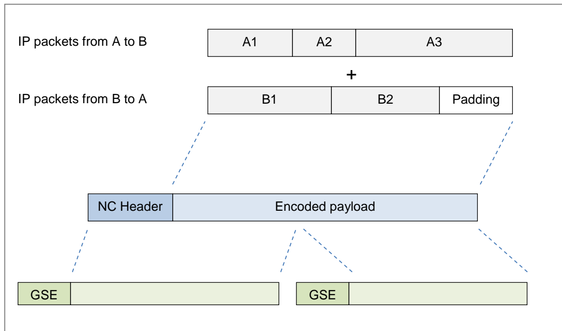
Figure 5-3 Packet encapsulation
