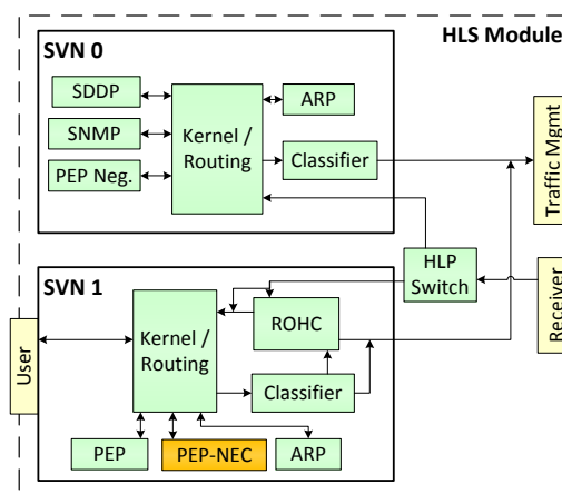
Figure 5-13 PEP-NEC integration
