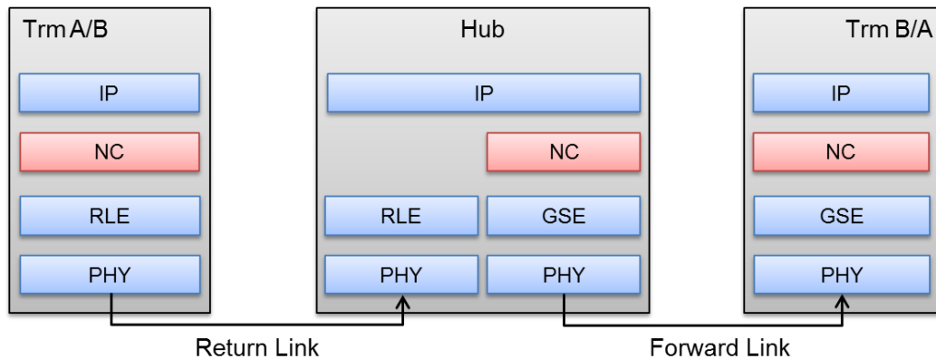
Figure 5-2 Protocol Stack.
