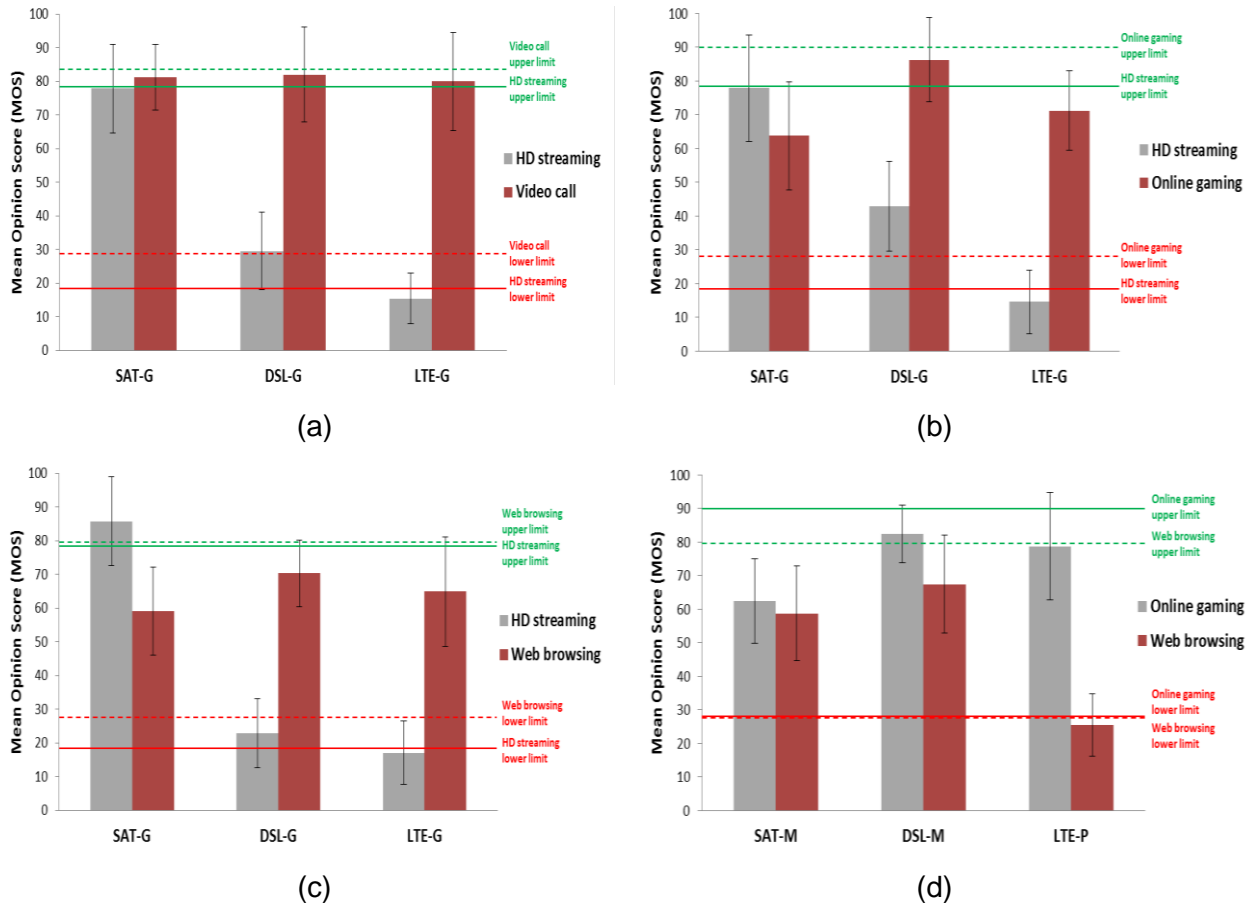
Figure 2-24: MOS results in Experiment II – Part 1
