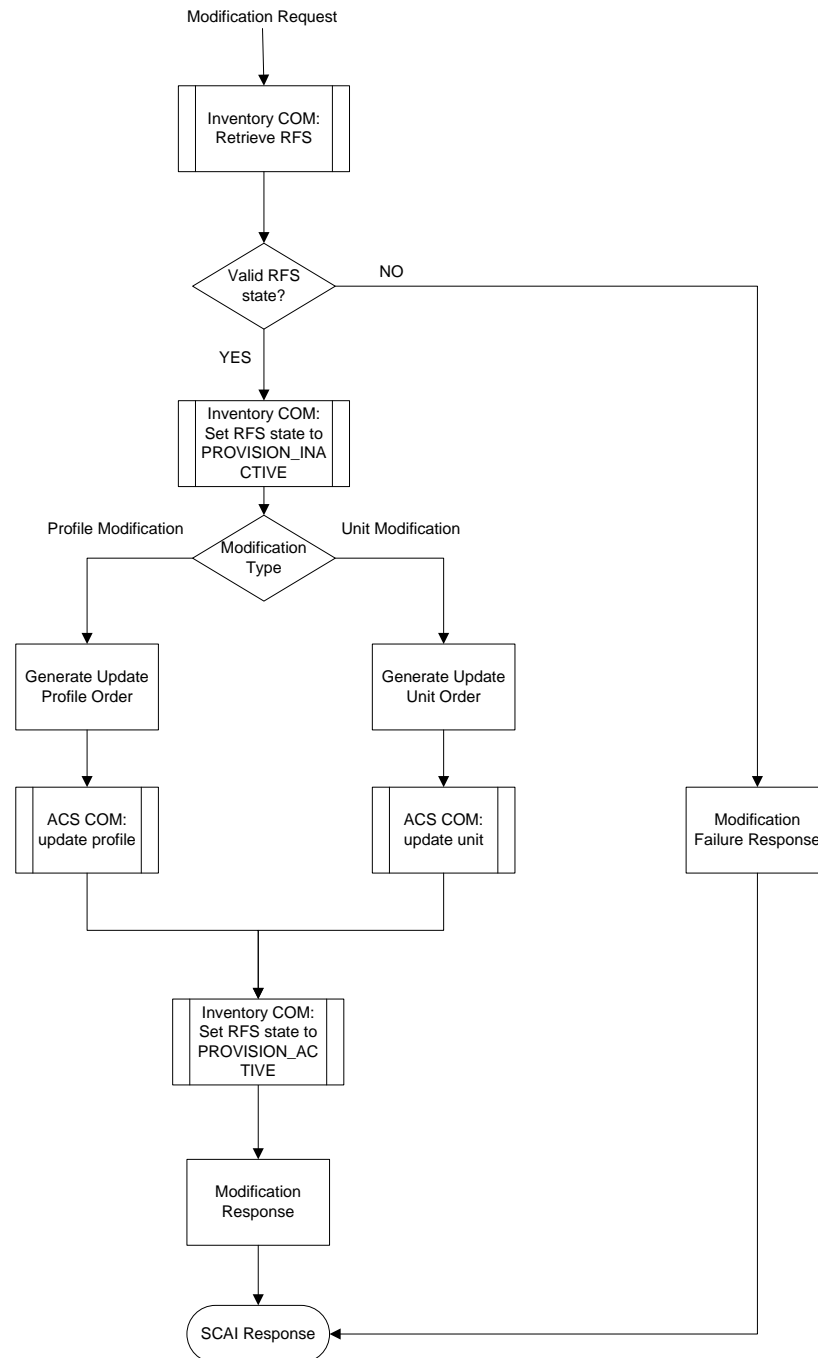
Figure A-6-15 SCAI modification specifics for ACS
