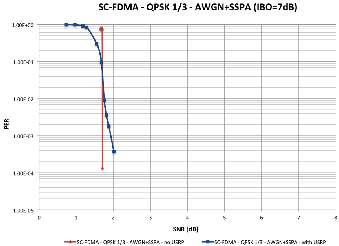
Figure 5-28: Packet Error Rate – QPSK 1/3 – AWGN+SSPA – with and without USRP
