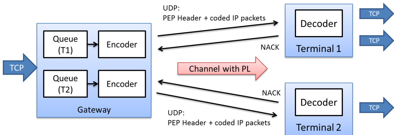
Figure 5-11 PEP-NEC implementation.
