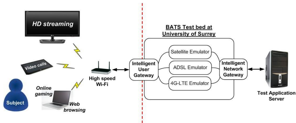
Figure 2-10 Overview of the lab trials test bed used for the subjective experiments
