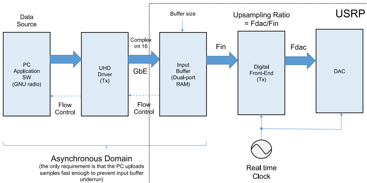
Figure 5-20: User Terminal: Baseband to Frontend interface
