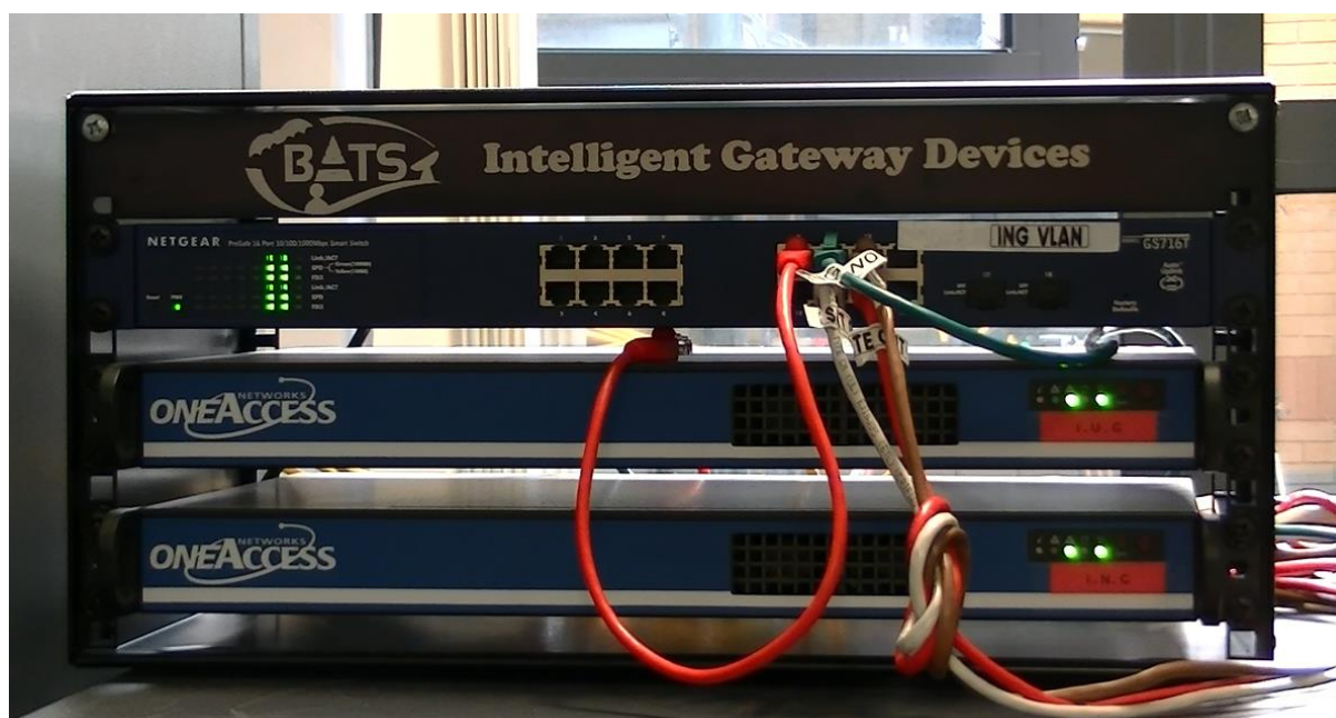
Figure 2-6 The IUG, ING and associated VLAN switch
