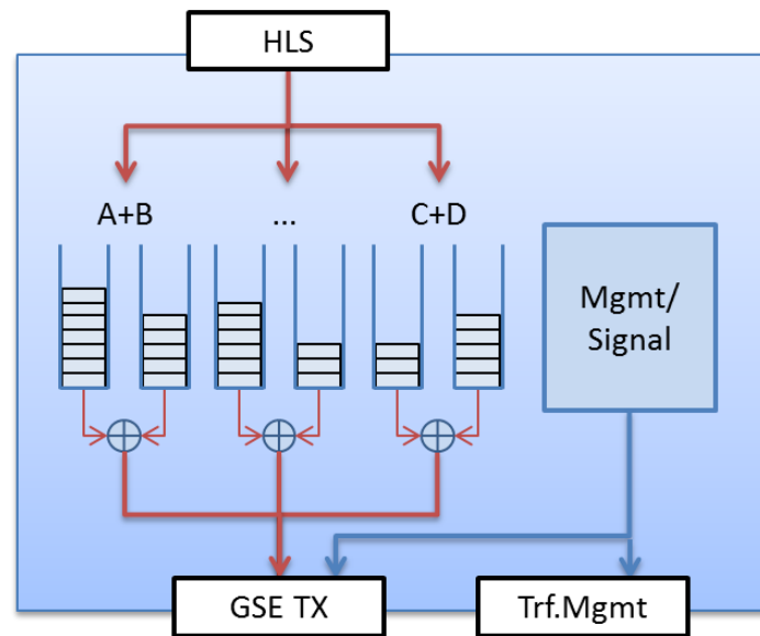
Figure 5-6 NC Hub Module
