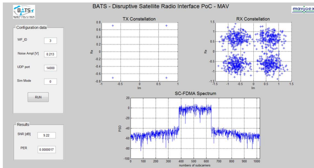
Figure 5-23: SC-FDMA Test-Bed: GUI implementation
