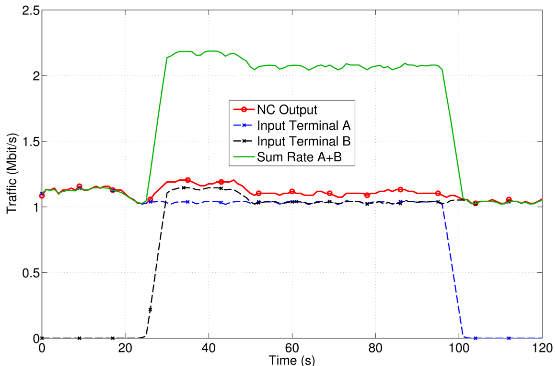
Figure 5-8: Data rates.
