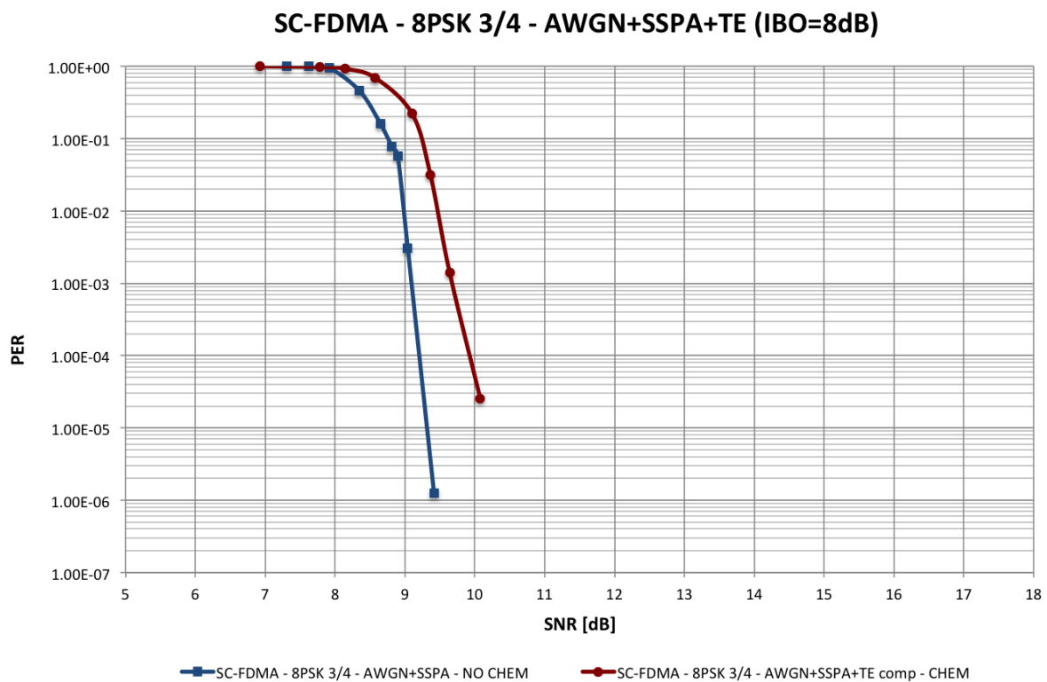
Figure 5-36: Packet Error Rate – 8PSK 3/4 – AWGN+SSPA NO CHEM and AWGN+SSPA+TE with CHEM
