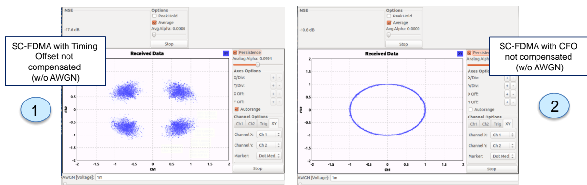
Figure 5-24: Timing offset (left) and CFO (right) not compensated
