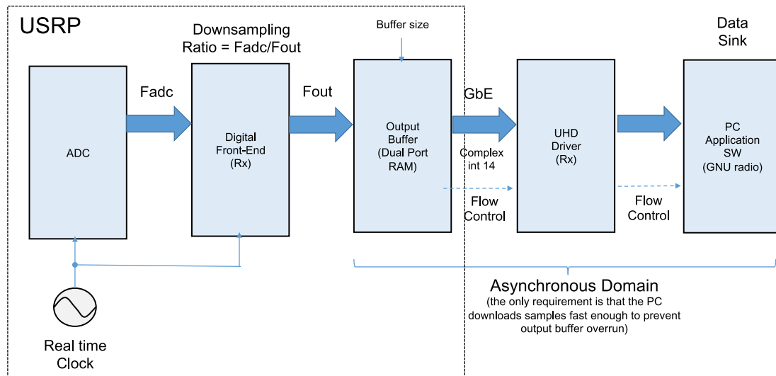
Figure 5-21: Gateway: Front-End to Baseband interface
