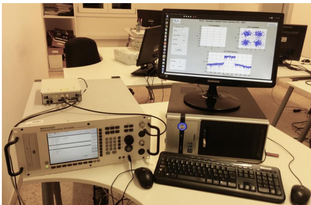
Figure 5-22: SC-FDMA Test-Bed - STEP 3 integration with the Channel Emulator
