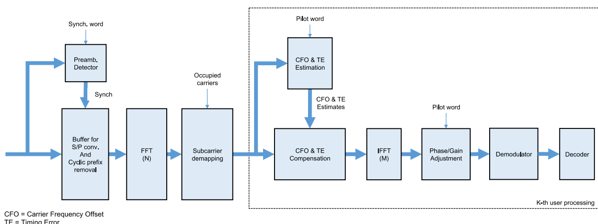
Figure 5-18: Gateway: RX Baseband processing
