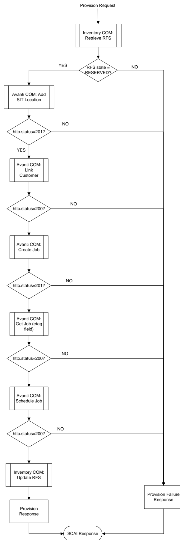
Figure A-6-3 Provision process and ESB implementation
