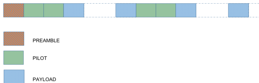
Figure 5-17: Frame structure
