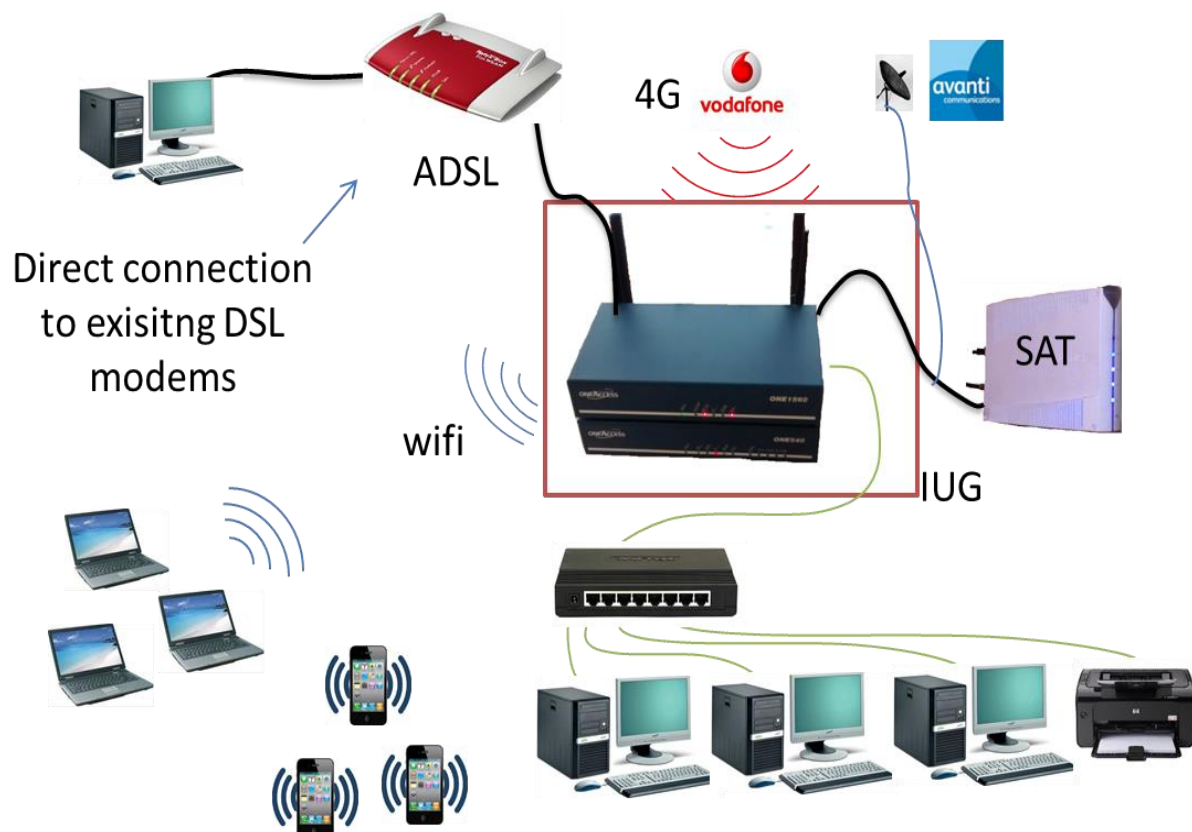
Figure 3-1 Setup for home office user
