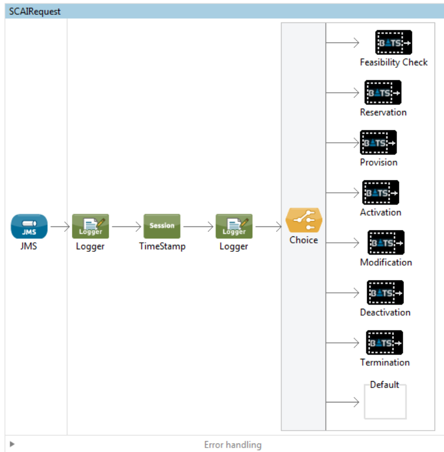
Figure 5-60: JMS Workflow
