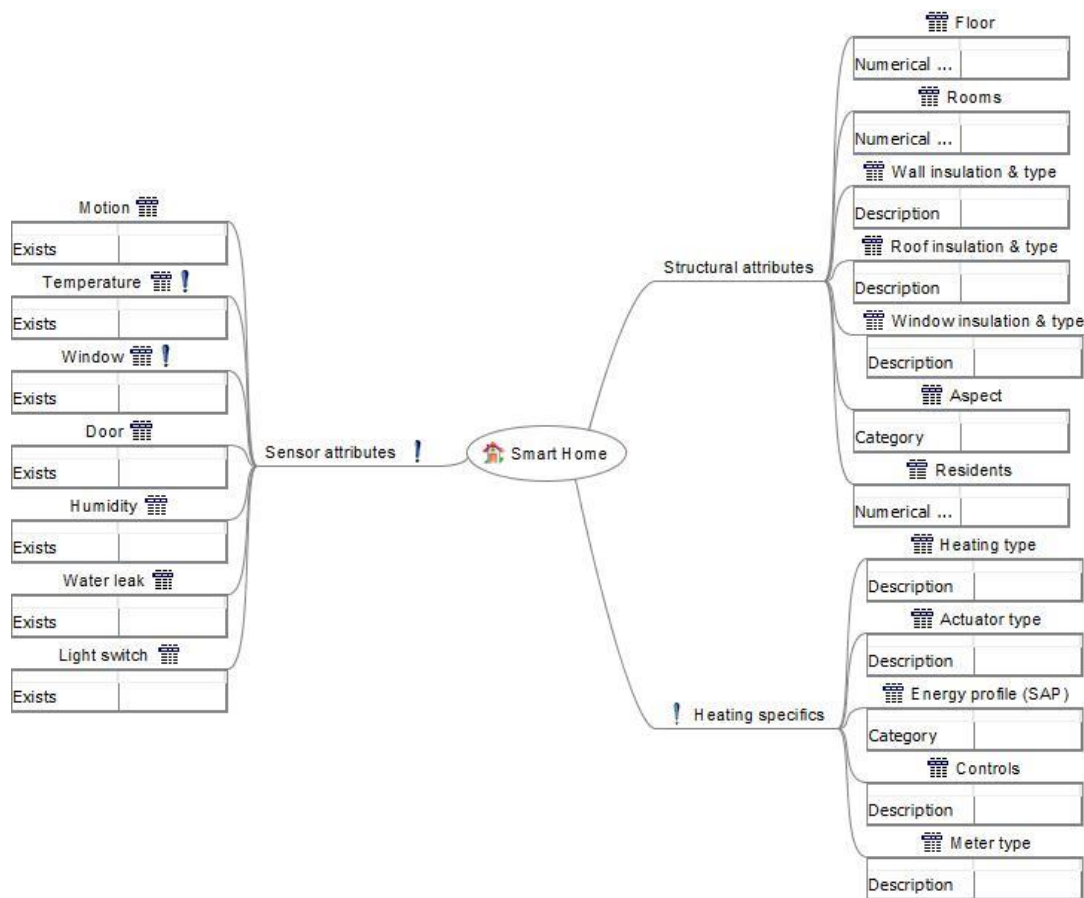
Figure 2: Smart Home Domain Specific Ontology Map
