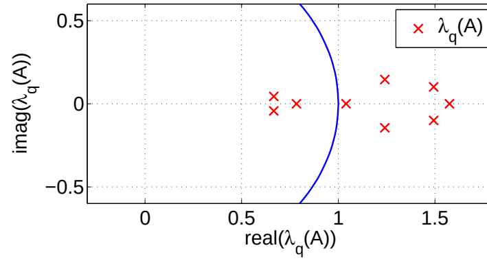
Figure 3.3: Eigenvalues of the system considered in the case study. The solid line indicates the stability bound.
