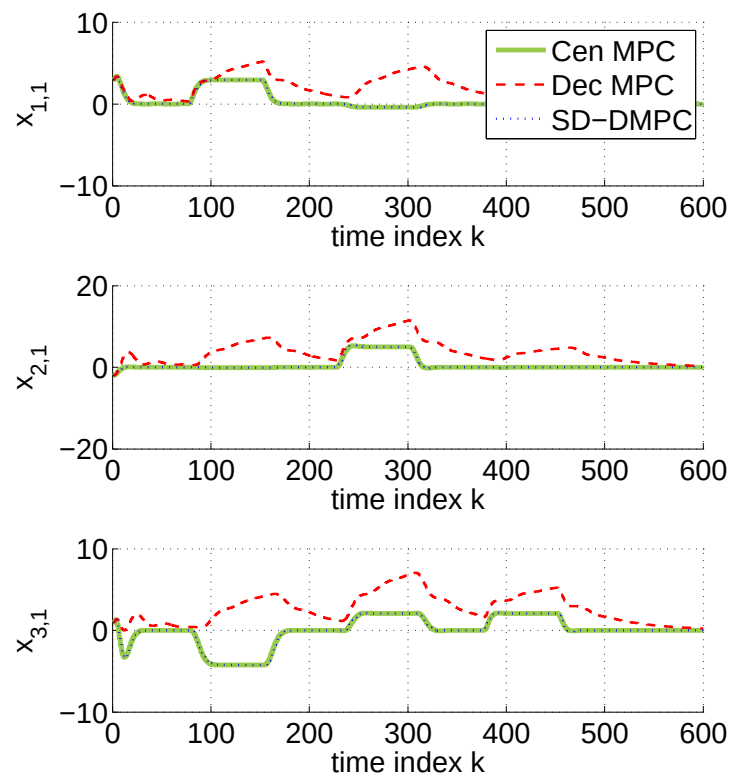
Figure 3.4: State trajectories
