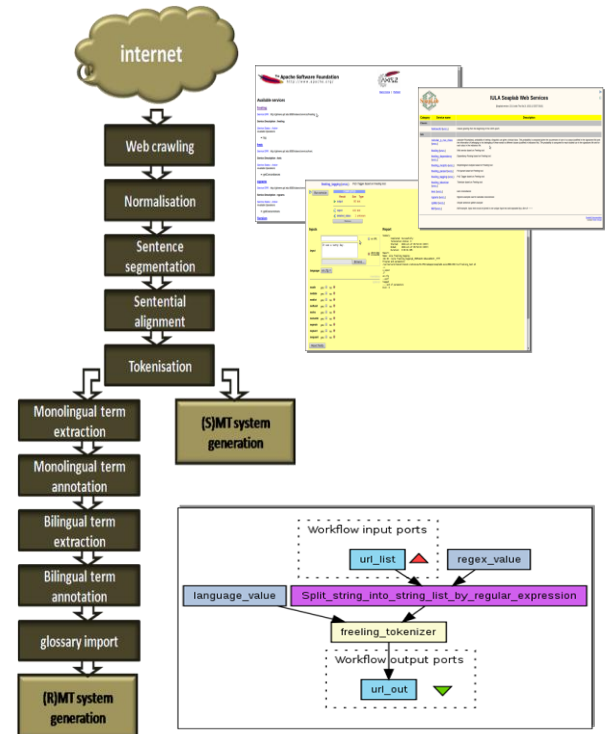
2. Different perspectives of web service workflows
