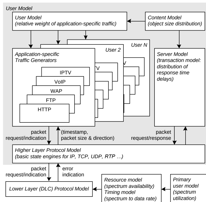
Figure B-11: User model data traffic generator
