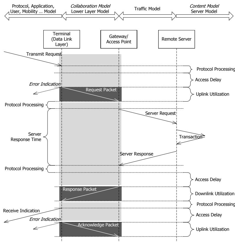
Figure B-10: Media access timing assumed
