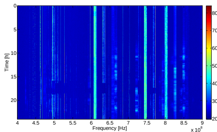
Figure B-2: One-day spectrum measurement
