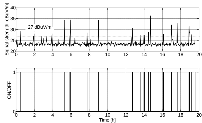
Figure B-3: Signal strength and ON/OFF activity
