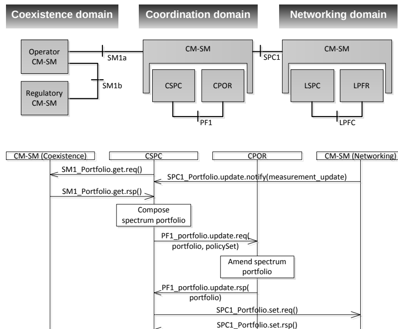
Figure 5-1: Accessing the CSCP in cellular scenarios and sample MSC
