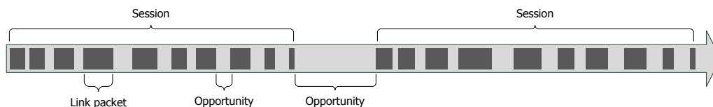
Figure B-12: Terminology: link utilization and access opportunities
