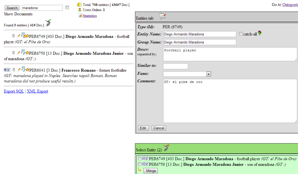
Figure 7: The Management Page of the current version of the tool.
