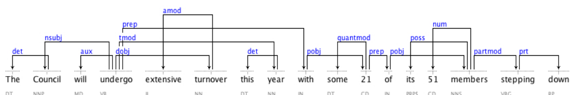
Figure 1: Example sentence with typed dependencies
