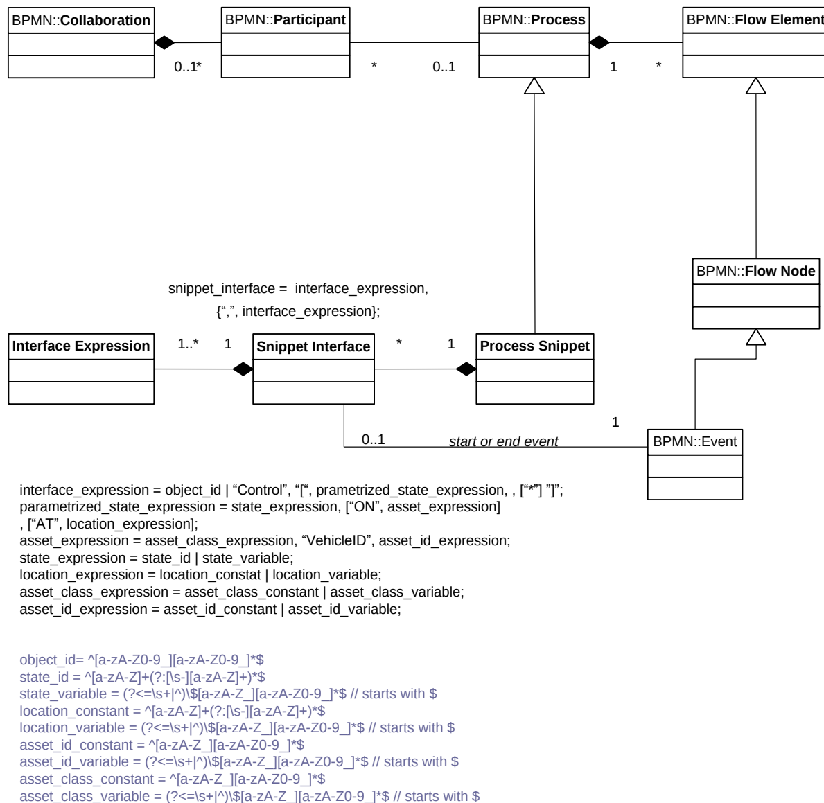
Figure 8: Metamodel for snippet interfaces
