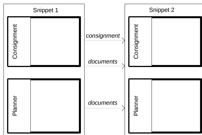
Figure 4: Snippet composition
