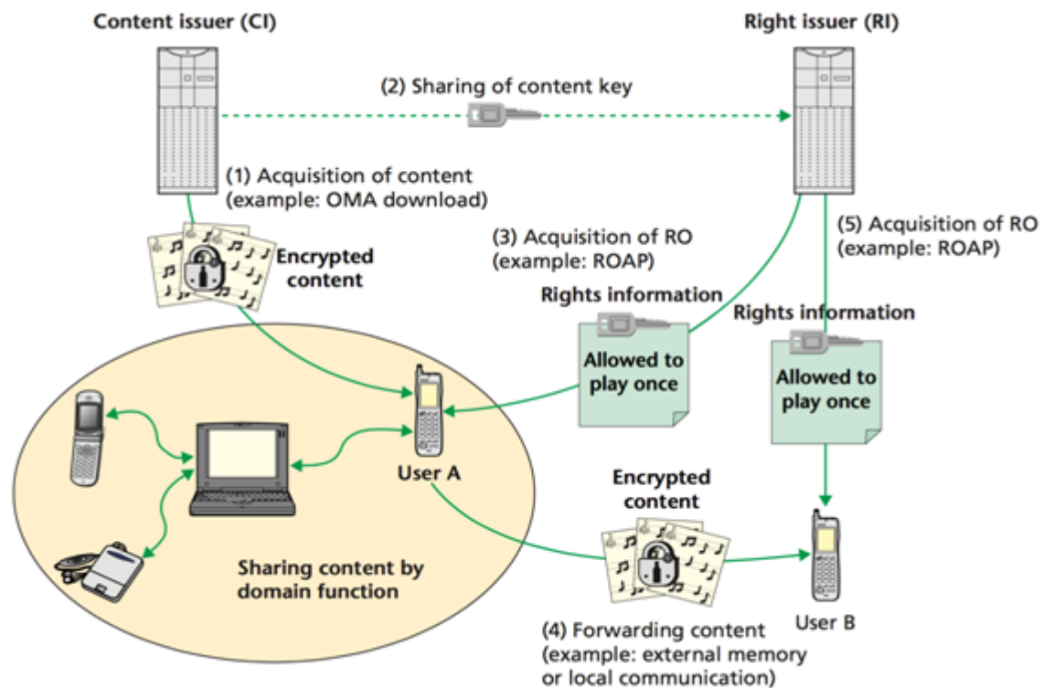
Figure 16 – Architecture of OMA DRM v2.0 [35]
