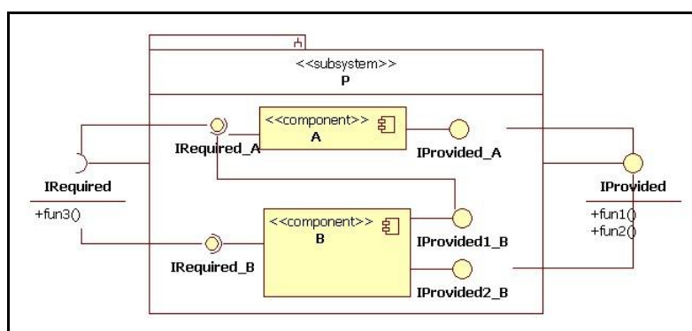
Figure 10: use UML to describe a pattern
